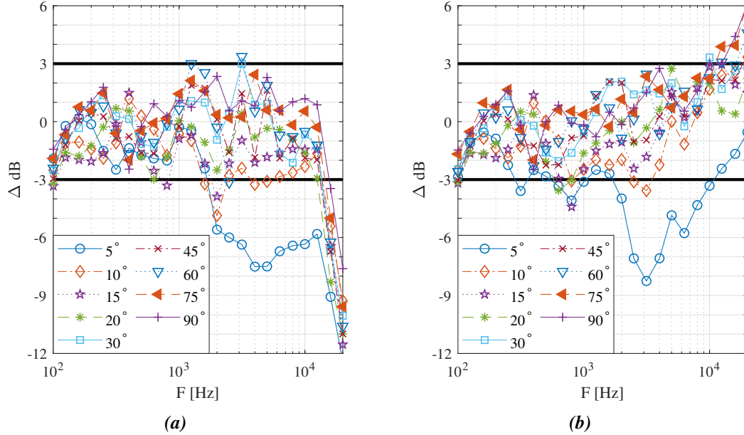
Figure 7: The differences (re: free-field) when the configurations were placed over three inches of sand and oriented at 0^\circ azimuth relative to the sound source for (a) inverted and (b) embedded microphone.
