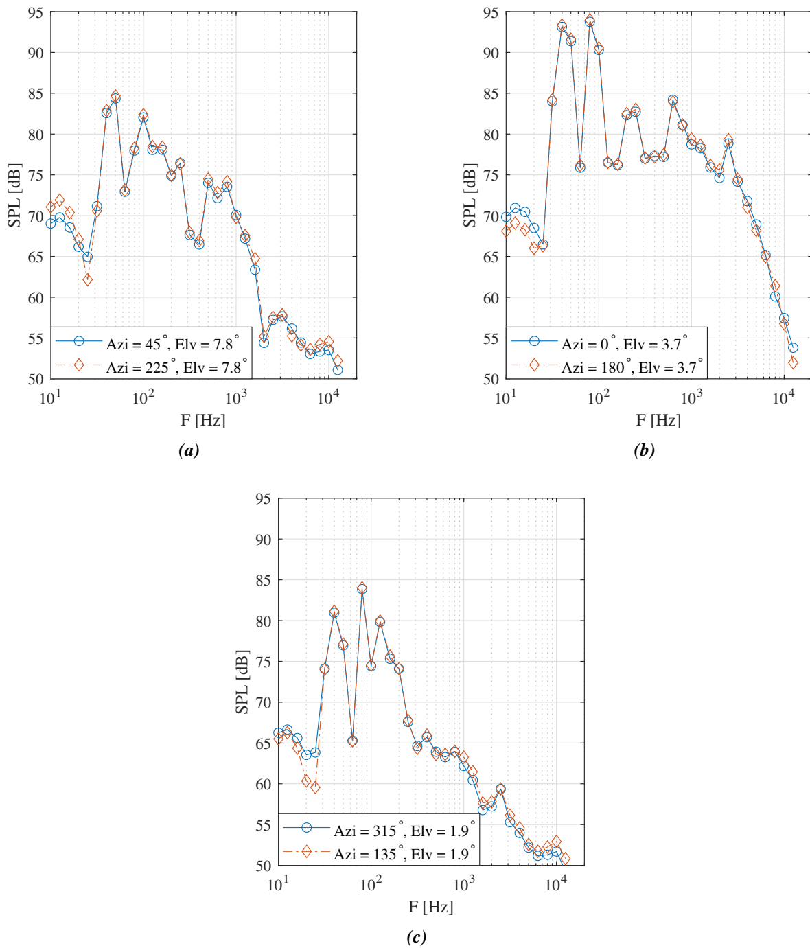
Figure 13: The spectra for two oppositely-oriented embedded microphones during a -9^\circ descending flight of an S-76D Helicopter flying at 60 kts for (a) approach, (b) pass-by, and (c) departure.
