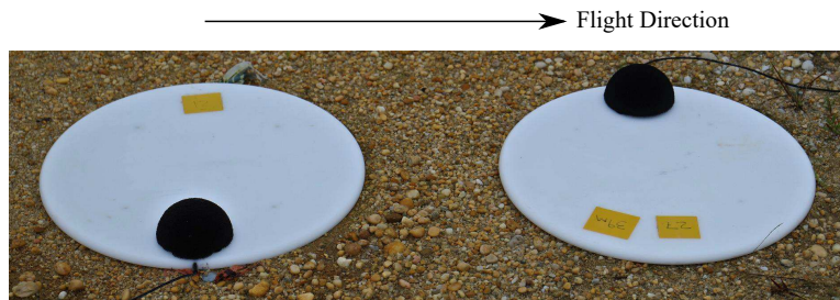
Figure 5: The two embedded microphone configurations that were used for the field test with windscreens.
