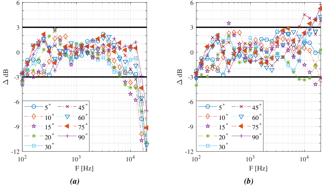
Figure 10: The differences (re: free-field) when the configurations were placed on plywood over three inches of sand and oriented at 180^\circ azimuth relative to the sound source for (a) inverted and (b) embedded microphone.
