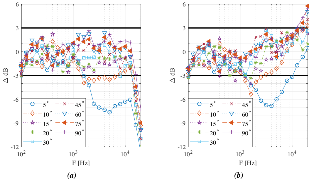
Figure 11: The differences (re: free-field) when the configurations were placed over three inches of sand and oriented at 45^\circ azimuth relative to the sound source for (a) inverted and (b) embedded microphone.
