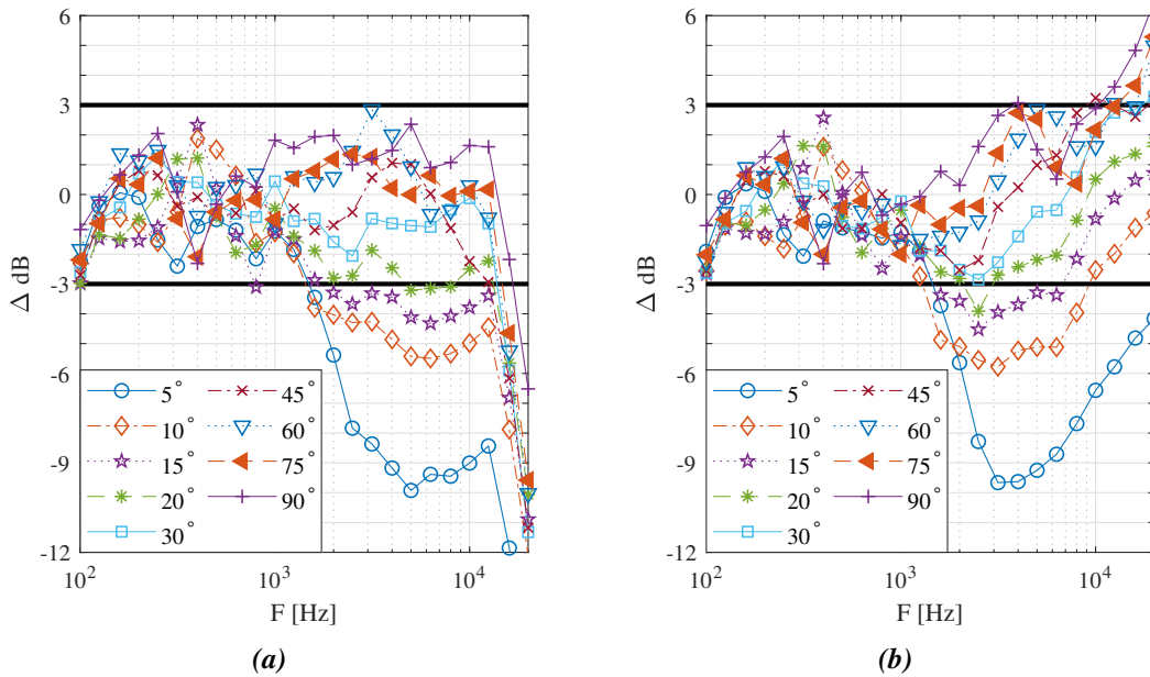
Figure 9: The differences (re: free-field) when the configurations were placed over three inches of sand and oriented at 180^\circ azimuth relative to the sound source for (a) inverted and (b) embedded microphone.
