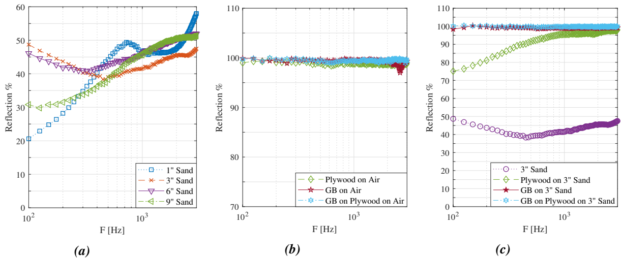
Figure 6: Normal impedance tube reflection results as a function of frequency for multiple configurations. (a) Reflection percentage from different depths of sand. (b) Reflection percentage from different solid surfaces placed over an air substrate. (c) Reflection percentage from various combinations tested in the anechoic phase of the experiment.
