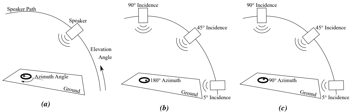
Figure 3: Schematic sketch of the anechoic chamber test setup, including (a) definition of the elevation and azimuthal angles. The ground board location was adjusted to place the microphone at the same location for each test, with azimuthal angle of (b) 180°, and (c) 90°.
