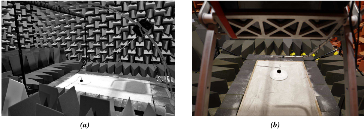
Figure 2: Photographs of the arc setup in the anechoic chamber with both a (a) wide-angle view of the entire setup and (b) speaker-oriented view of a microphone configuration under test.
