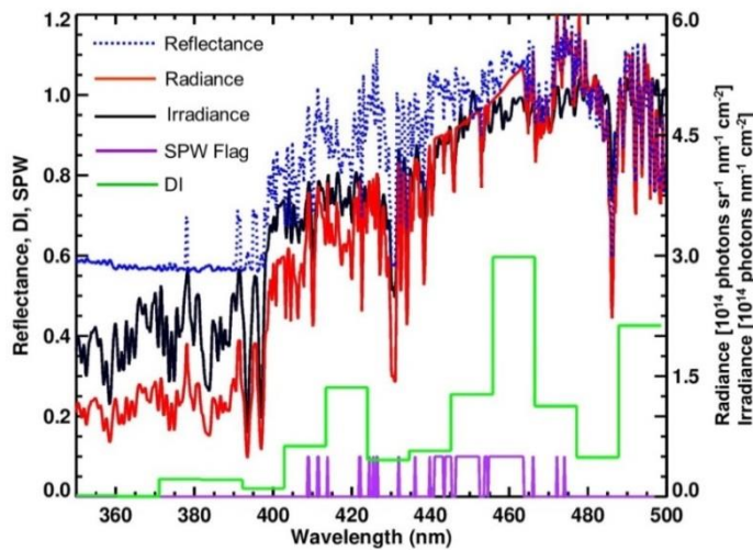
Figure 5: Similar to Fig. 2 but for pixel iTimes 824, row 15, orbit 7987 indicated by arrows in Fig. 4(c,d) showing solar glint from Lake Salar de Uyuni.
