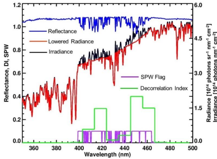
Figure 3: Similar to Fig. 2 but for iTimes - 807, Row - 20, orbit 7990, January 14, 2006 in cloud region B (see arrows in Fig.1 c,d). The radiance was lowered by a few percent for better comparison.
