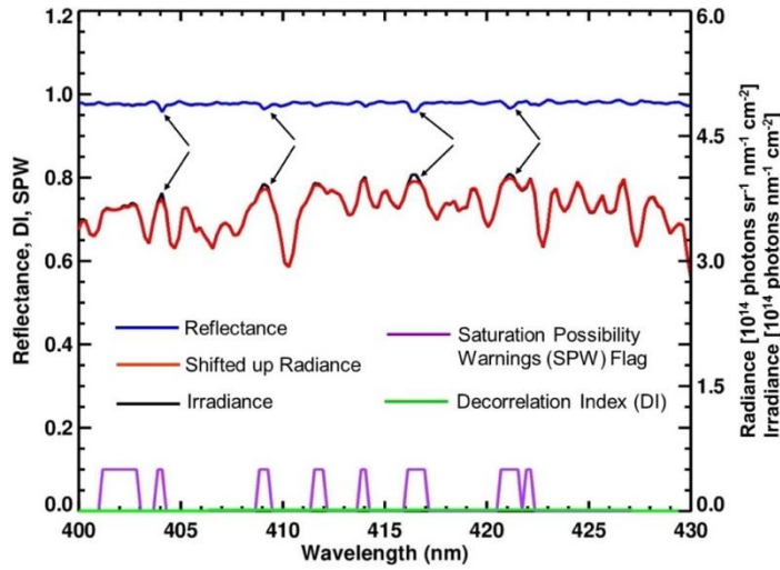
Figure 2: Data for iTimes 839, row 15, orbit 7990, January 14, 2006 in zone A (this pixel is marked by arrows in Fig. 1(c,d). The blue line at the top of the picture is reflectance \pi I/[F_0 \cos(\theta)] , where \theta is solar zenith angle. Reflectance in this zone has slight variations caused by minor saturation in the atmospheric spectrum as indicated by the arrows. The purple line shows the binary SPW (Saturation Possibility Warning) flags multiplied by 0.1. The green line is the DI < 0.01 for bands 403-413, 413-424, 424-434 nm. The intensity of the radiance spectrum is shifted upwards slightly for clearer comparison with the irradiance spectrum.
