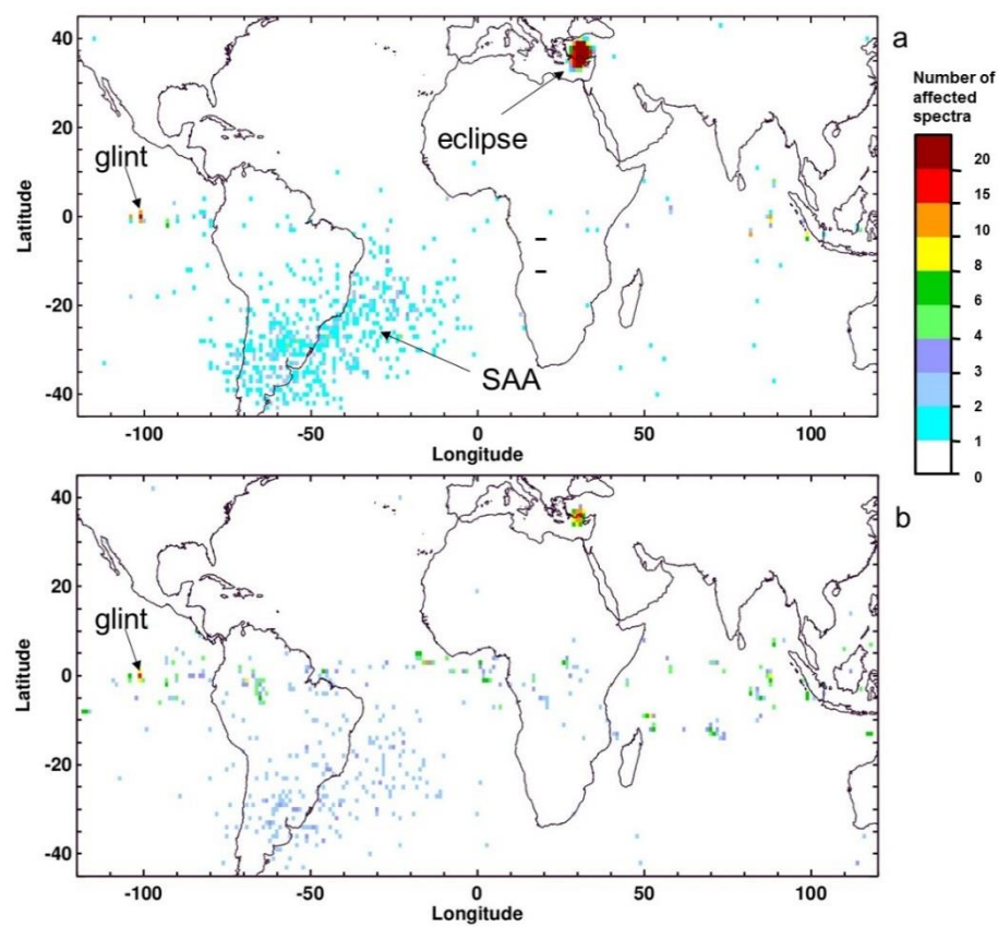
Figure 8: Gridded (1°x1°) distributions of the number of affected spectra for March 2006; (a) Vis band 424.1-434.5 nm, DI > 0.03; (b) Vis 445.3-455.7 nm, DI > 0.25. The South Atlantic Anomaly (SAA) and a region affected by solar eclipse are clearly visible; the remaining pixels with high DI values are mostly associated with sun glints and bright clouds.
