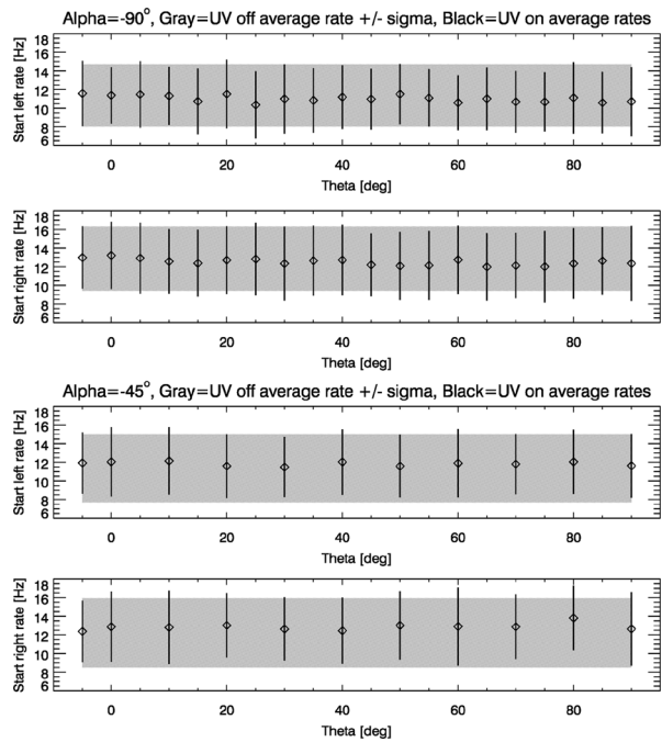
Fig. 63 Results of UV contamination tests for Strofiio MCPs
