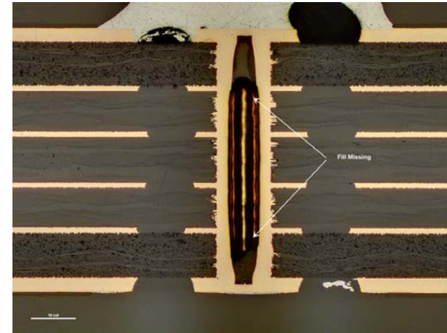
Capped via with fill less than 75%
