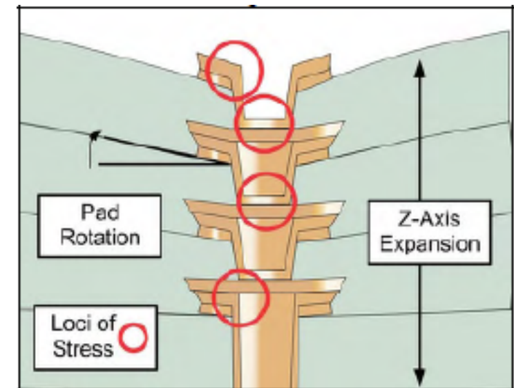
Target pad cracks [2]
