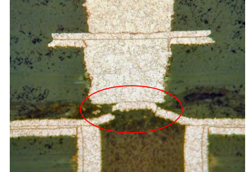
Target pad cracks [2]
