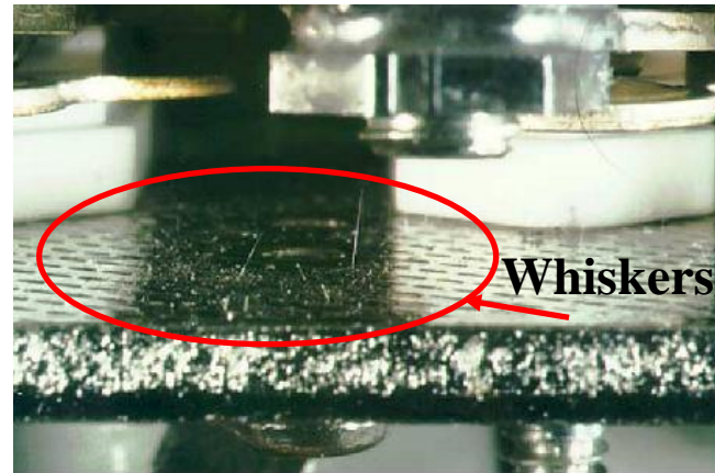
Whiskers on the armature of a relay
