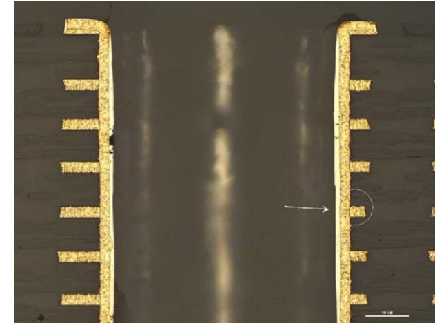
Internal Annular Ring (IAR) less than the minimum 5.0 mil
