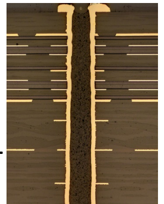
PTH in Cross-section
