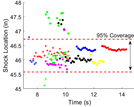
Fig. 15 Scatter of HDCR combustion induced shock location measurement.
