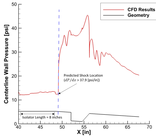
Fig. 5 Current CFD combustion-induced shock location methodology.
