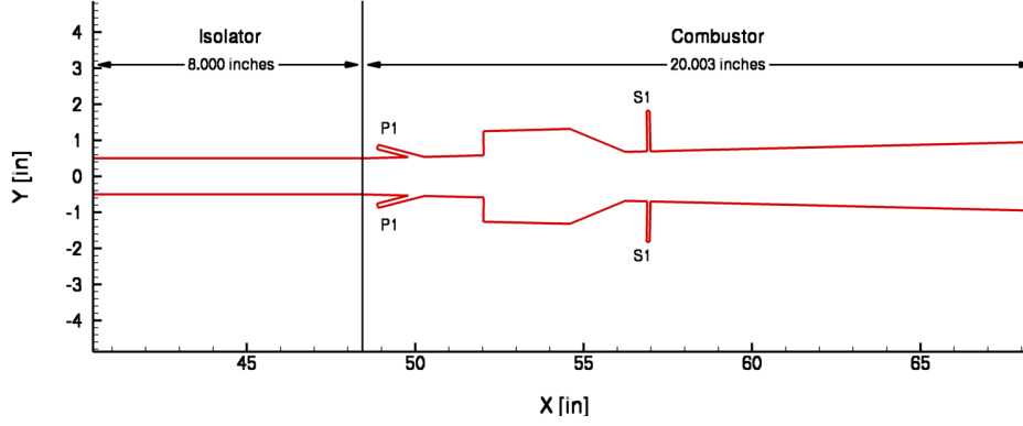
Fig. 2 Two-dimensional profile of the HIFiRE Flight 2 isolator and combustor geometry.
