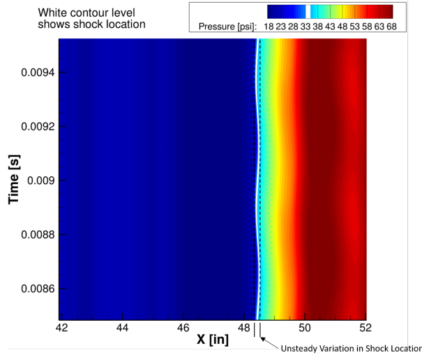
Fig. 13 Unsteady variation in the combustion-induced pressure rise as a function of time.
