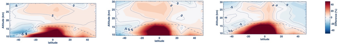
Figure 4. Panels (a) through (c) show the difference between the aerosol climatology when reflectivity is greater than 0.3 and when reflectivity is less than 0.3. Extinction climatology at 745, 869 and 997 nm. The dashed line is tropopause altitude. The contour line shows differences greater than \pm 5\% .
