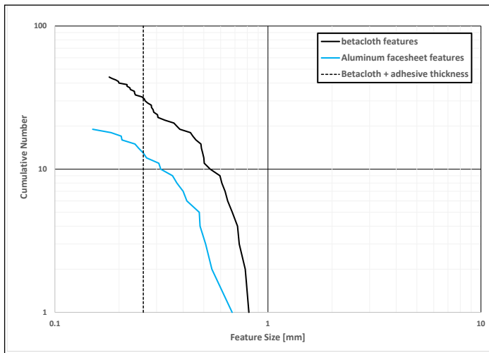
Figure 5. BCDU-0016 cumulative number as a function of feature size. A total of 44 impact features were observed in the Betacloth blanket, the holes ranging from 0.18 mm to 0.81 mm in diameter. Nineteen additional craters in the aluminum facesheet or anodized fixtures were noted; these ranged from 0.15 mm to 0.68 mm in diameter. See also Table 2.
