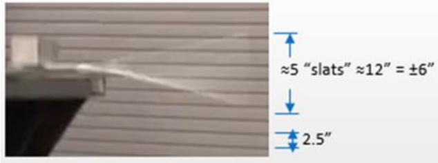
Figure 6: Tip Displacement
