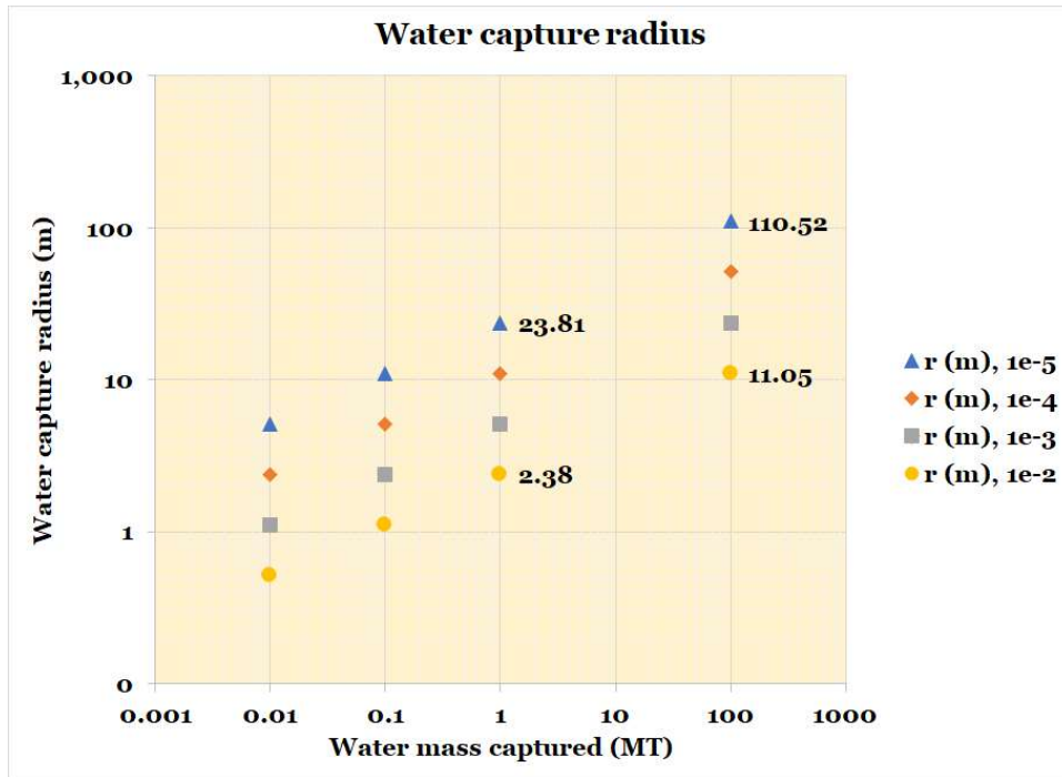
Figure 18. Water mining storage vessel radius, Phobos, water mass fraction: 1 \times 10^{-5} to 1 \times 10^{-1}
