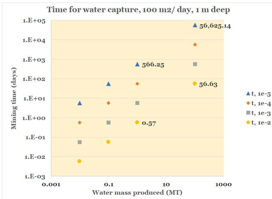
Figure 19. Water mining time, Phobos, water mass fraction: 1 \times 10^{-5} to 1 \times 10^{-1}
