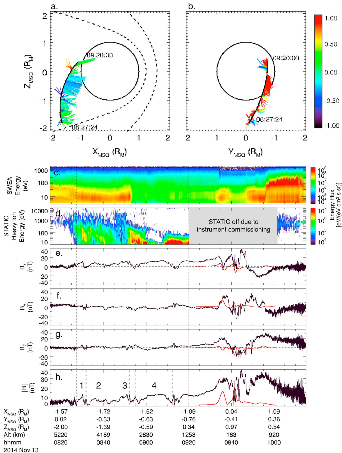
Figure 1. A portion of MAVEN's orbit on 13 November 2014 (corresponding to vertical dashed lines in time series) viewed from (a) the meridional ( X_{\text{MSO}}-Z_{\text{MSO}} ) plane and (b) behind the planet toward the Sun ( Y_{\text{MSO}}-Z_{\text{MSO}} ). Nominal IMB and bow shock positions [Trotignon et al. , 2006] are indicated by dashed lines. Normalized magnetic field vector projections are plotted along the trajectory where the color represents the normalized out-of-plane component: B_y (Figure 1a) and B_x (Figure 1b). MAVEN plasma and magnetic field data: (c) SWEA electron energy spectra; (d) STATIC energy spectra of heavy ions with M/q \geq 12 ; (e-h) magnetic field components, B_x , B_y , and B_z , in MSO coordinates and total field magnitude, |B| , provided by MAG (black lines). Red lines in Figures 1e-1h represent crustal magnetic field spherical harmonic model outputs from Morschhauser et al. [2014]. In Figure 1h vertical dotted lines mark times that magnetic flux ropes were detected.
