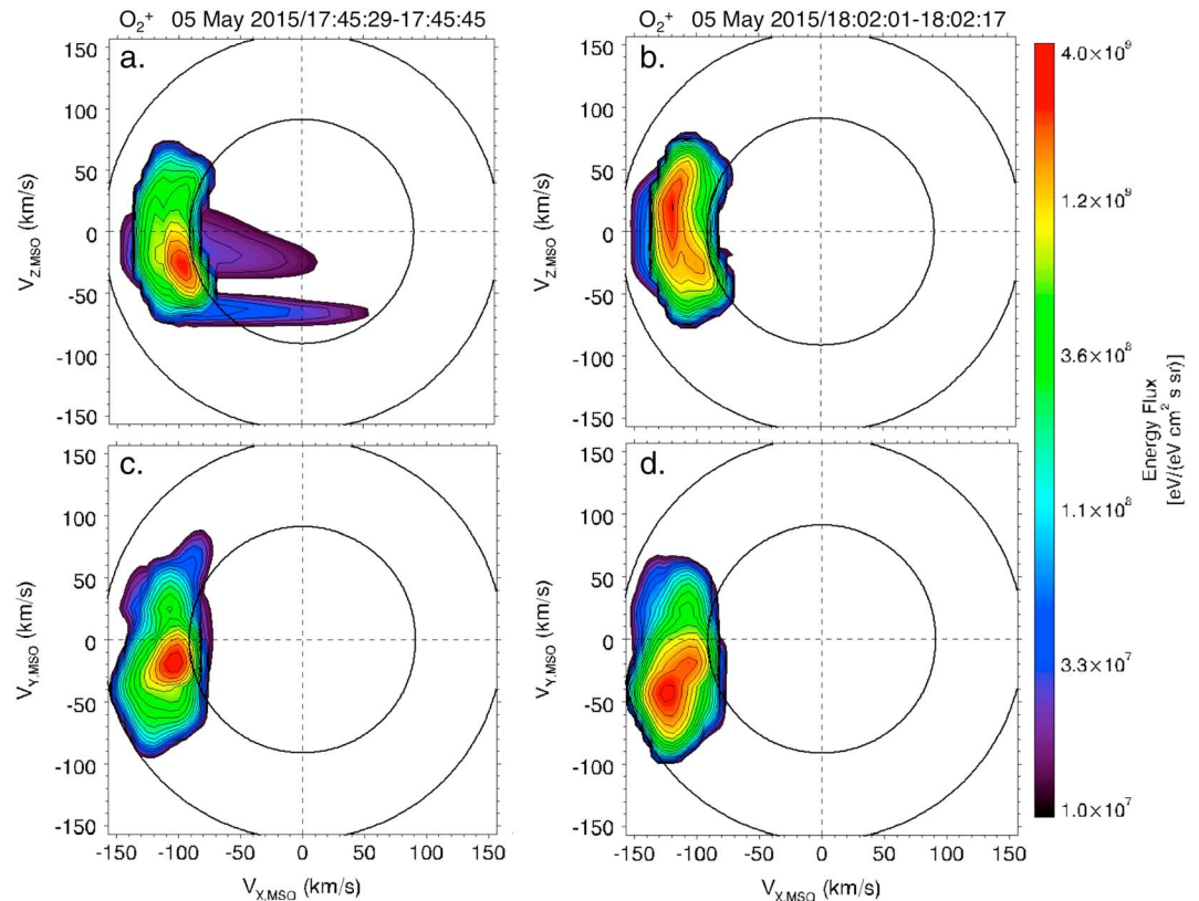
Figure 3. Slices of O_2^+ velocity distribution functions in the (a and b) V_{X,MSO} – V_{Z,MSO} and (c and d) V_{X,MSO} – V_{Y,MSO} planes for energies between 1–5 keV (concentric circles) during the (Figures 3a and 3c) partial and (Figures 3b and 3d) full current sheet crossings in Figure 2.
