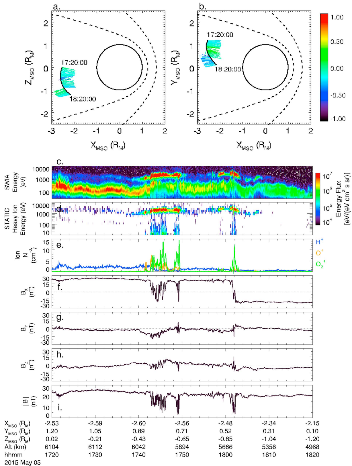
Figure 2. A portion of MAVEN's orbit on 5 May 2015 viewed from the (a) meridional ( X_{\text{MSO}}-Z_{\text{MSO}} ) and (b) equatorial ( X_{\text{MSO}}-Y_{\text{MSO}} ) planes. See Figure 1 caption. MAVEN plasma and magnetic field data: (c) SWIA ion energy; (d) STATIC energy of heavy ions with M/q \geq 12 ; (e) densities of \text{H}^+ , \text{O}^+ , and \text{O}_2^+ ; (f-i) magnetic field components, B_x , B_y , and B_z , in MSO coordinates and total field magnitude, |B| .
