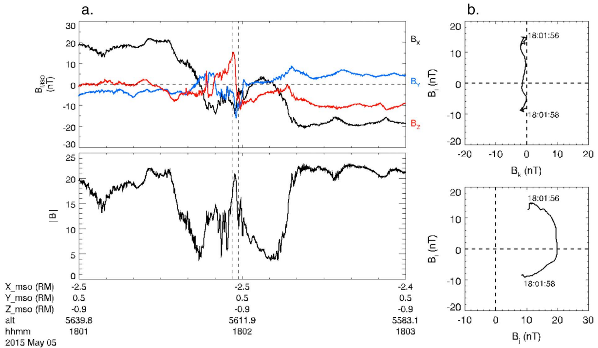
Figure 4. (a) MAG data during the 5 May 2015 current sheet traversal. Vertical dashed lines mark the minimum variance analysis interval. (b) Magnetic field hodograms in minimum variance analysis coordinates.
