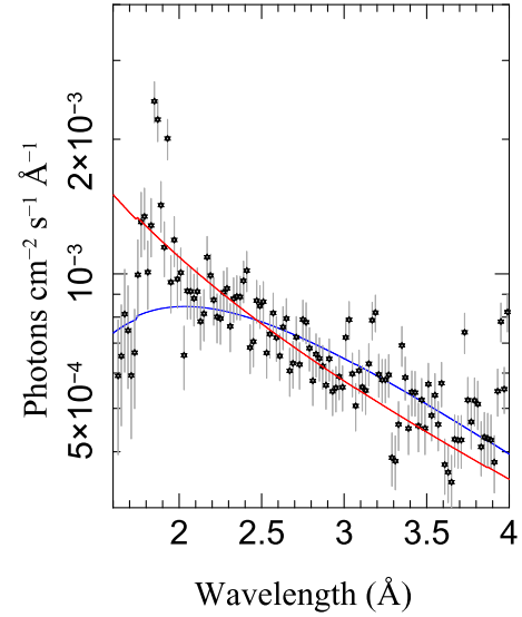
Figure 6. Comparison of the power-law fit (red) to the blackbody fit (blue) in the Fe K line region (the data are black).
