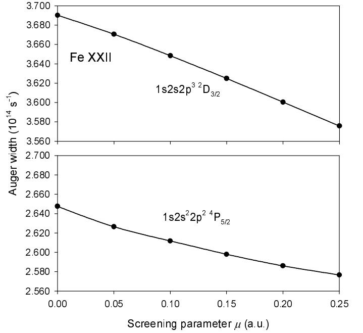
Fig. 7. Variation of the Auger width with the plasma screening parameter \mu for two K-vacancy levels in Fe XXII.
