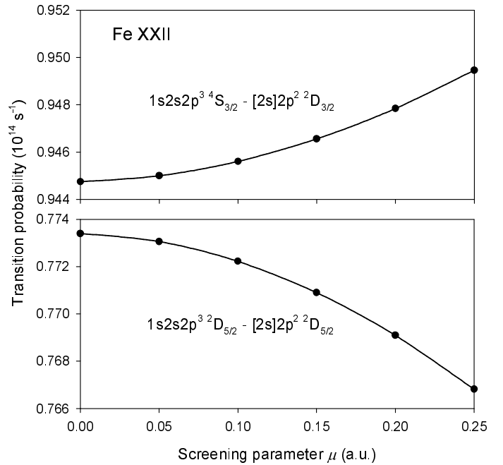
Fig. 6. Variation of the transition probability (A-value) with the plasma screening parameter \mu for the 1s2s2p^3\ ^4S_{3/2} - [2s]2p^2\ ^2D_{3/2} and 1s2s2p^3\ ^2D_{5/2} - [2s]2p^2\ ^2D_{5/2} lines in Fe xxii.
