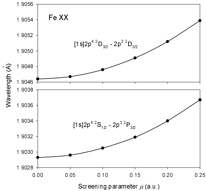
Fig. 4. Wavelength reddening as a function of the plasma screening parameter \mu for the [1s]2p^4\ ^2D_{3/2} - 2p^3\ ^2D_{3/2} and [1s]2p^4\ ^2S_{1/2} - 2p^3\ ^2P_{3/2} K \alpha lines in Fe xx.
