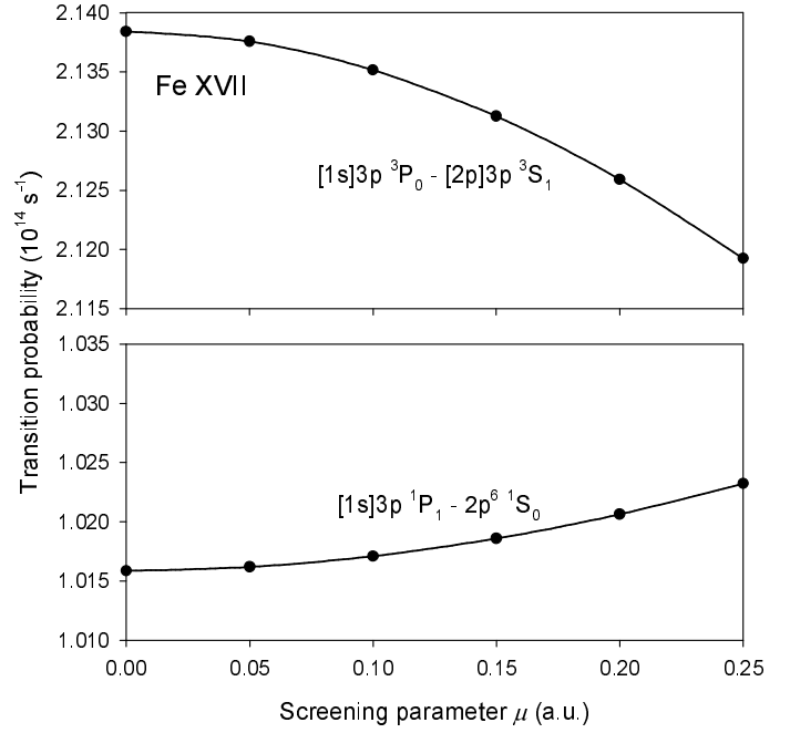
Fig. 5. Variation of the radiative transition probability (A-value) with the plasma screening parameter \mu for the [1s]3p\ ^3P_0 - [2p]3p\ ^3S_1 and [1s]3p\ ^1P_1 - 2p^6\ ^1S_0 lines in Fe xvii.
