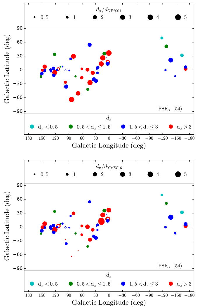
Figure 14. Ratio of VLBI parallax distance to the NE2001 model distance (top panel) and the YMW16 model distance (bottom panel). The results are shown as a function of Galactic longitude and latitude. Circle sizes indicate the value of the ratio, as shown in the upper legend in each panel. Circle colors denote parallax distance in kpc as in the lower legend in each panel. Filled circles denote distance measurements, while the three open circles indicate lower bounds on pulsar distances.
