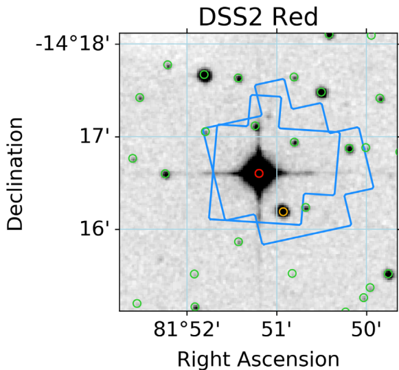
Figure 2. The 3' \times 3' DSS2 (red filter) image with the Sectors 5 and 6 SPOC photometric apertures overlaid in blue. Colored circles denote the positions of Gaia DR2 sources within 2' of TOI-421: red circle is TOI-421 (2984582227215748864), orange circle is a likely bound M dwarf companion (2984582227215748224), and other sources are in green. We computed the contamination from the companion and other stars contributing flux to the aperture, but it is insignificant at 1.8 \pm 0.4\% (and consistent with the TIC contamination ratio of 0.024605; see Section 2).
