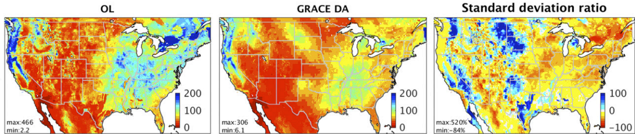
FIG. 2. Groundwater storage standard deviation (mm) derived from CLSM open loop (OL) and GRACE data assimilation (GRACE-DA) runs for the 2003–16 period and the standard deviation ratio (%), represented as [(\text{GRACE-DA}/\text{OL}) - 1] \times 100 .
