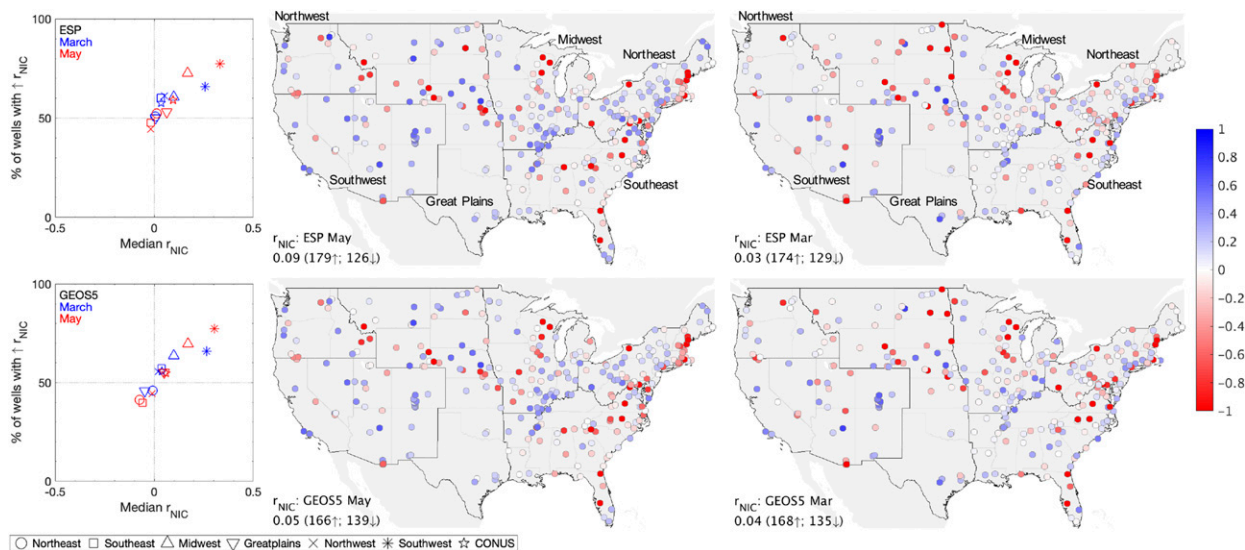
FIG. 4. As in Fig. 3, but for r_{NIC} values.
