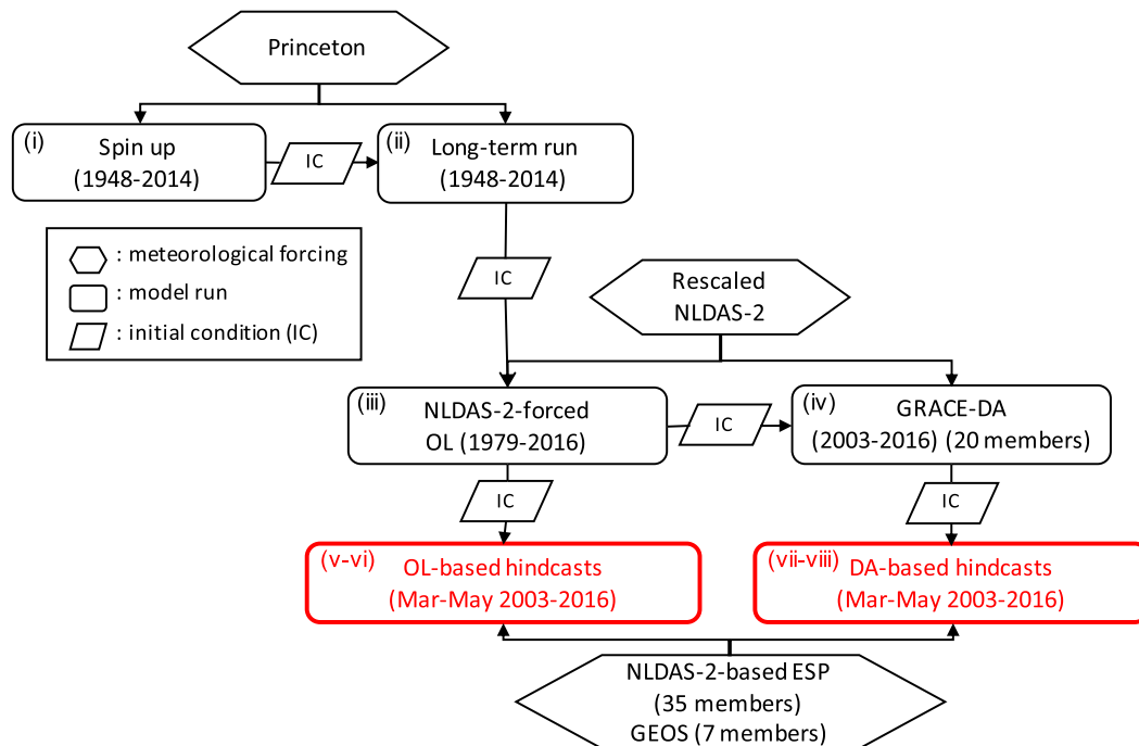
FIG. 1. Modeling flowchart. Experiments are ordered with roman numerals.
