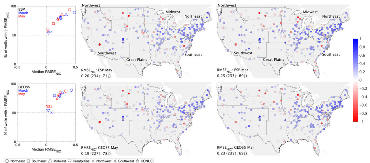
FIG. 3. GRACE-DA impact on the seasonal hindcast initialization using surface meteorological data from ESP and GEOS historical forecasts. (right) Spatial distribution of \text{RMSE}_{\text{NIC}} values derived from daily 3-month groundwater hindcasts initialized in May and March over the 2003–16 period. At the bottom left of each map, the median value and number of wells with improved ( \uparrow ) and degraded ( \downarrow ) metrics. (left) Median ( x axis) and percentage of wells with positive NIC values ( y axis) computed for daily 3-month hindcasts initialized in May and March for each U.S. region (Northeast, Southeast, Midwest, Great Plains, Northwest, and Southwest).
