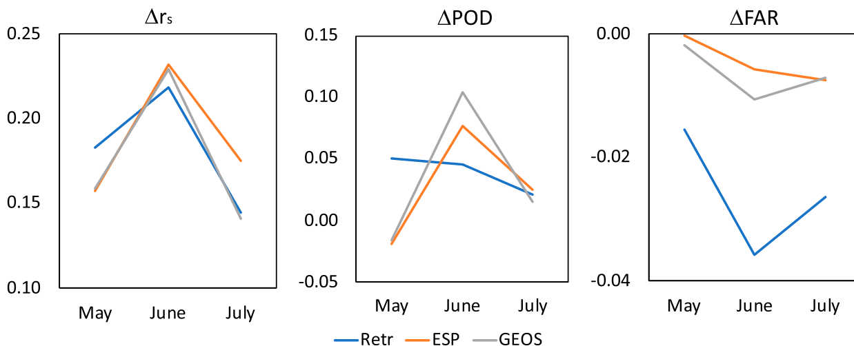
FIG. 8. Differential spatial correlation ( \Delta r_s ), probability of detection ( \Delta POD ) and false alarm rate ( \Delta FAR ) of drought severity index maps for three dates in 2014, as shown in Fig. 7. POD and FAR thresholds were defined as the extreme ( D_3 ) and exceptional ( D_4 ) drought events combined, corresponding to the 5th percentile. Values correspond to the improvement in skills when ESP and GEOS forecast techniques are initialized with GRACE-DA (i.e., GRACE-DA – OL). Differential values for the retrospective runs (Retr) are also shown for comparison purposes. Improvement is represented by positive values for r_s and POD, and negative values for FAR.
