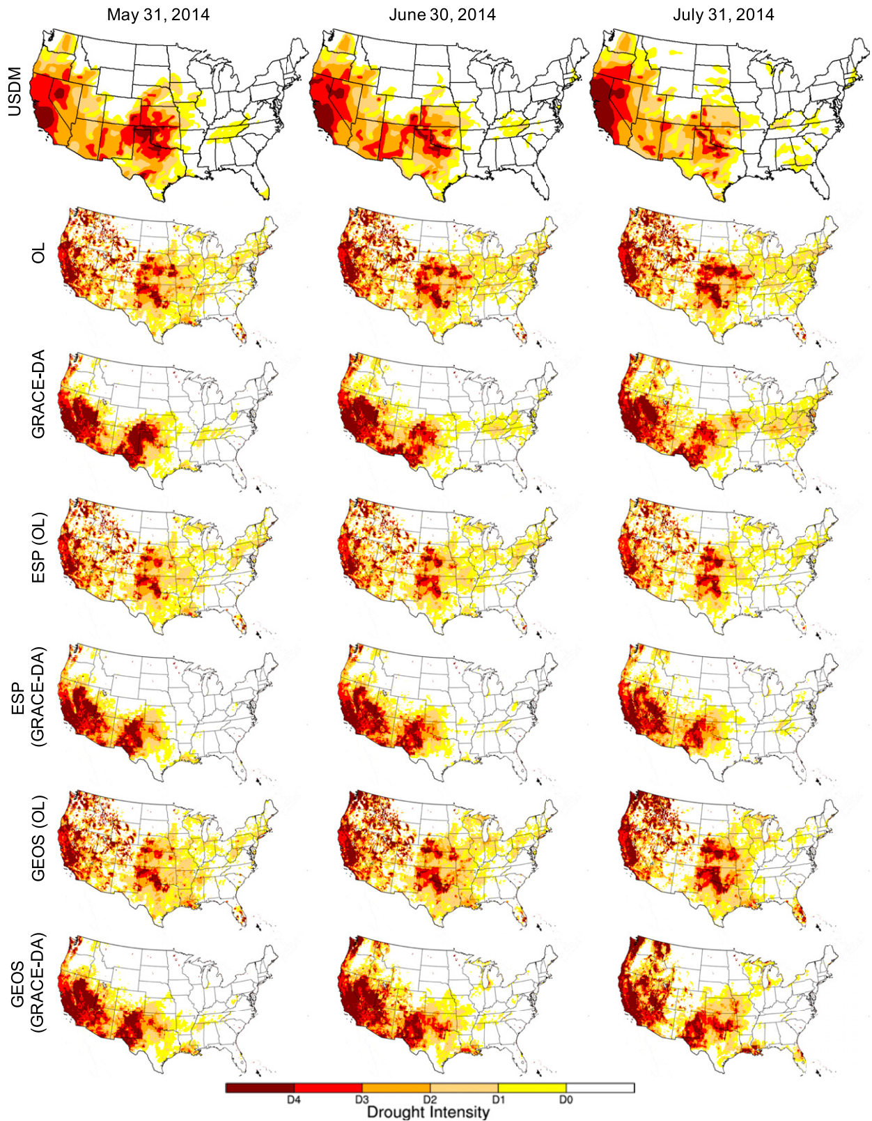
FIG. 7. U.S. drought intensity maps during major droughts in the western and southern United States between May and July 2014. Shown from top to bottom are U.S. Drought Monitor, retrospective OL and GRACE-DA runs, and ESP and GEOS hindcasts initialized with the 1 May GRACE-DA states. USDM estimates correspond to drought intensity on 3 Jun, 1 Jul, and 5 Aug, and the other experiments are snapshots at the dates displayed on the top of each column.
