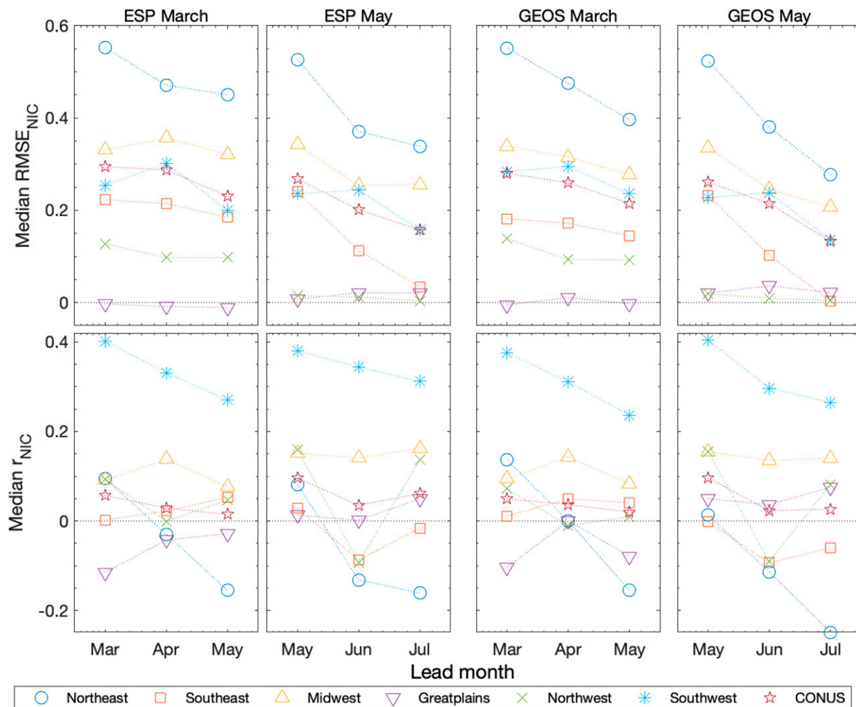
FIG. 6. Impact of initializing groundwater storage seasonal forecasts with GRACE-DA, for each lead month and region, for the 2003–16 period. The impact is defined as the normalized information contribution (NIC) of the RMSE and correlation r .
