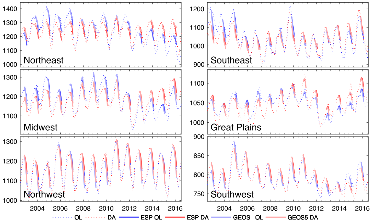
FIG. 5. Daily groundwater variability averaged for six U.S. regions. Dotted lines represent OL and GRACE-DA retrospective runs, and bold lines are 3-month ESP and GEOS hindcasts initialized on 1 May.
