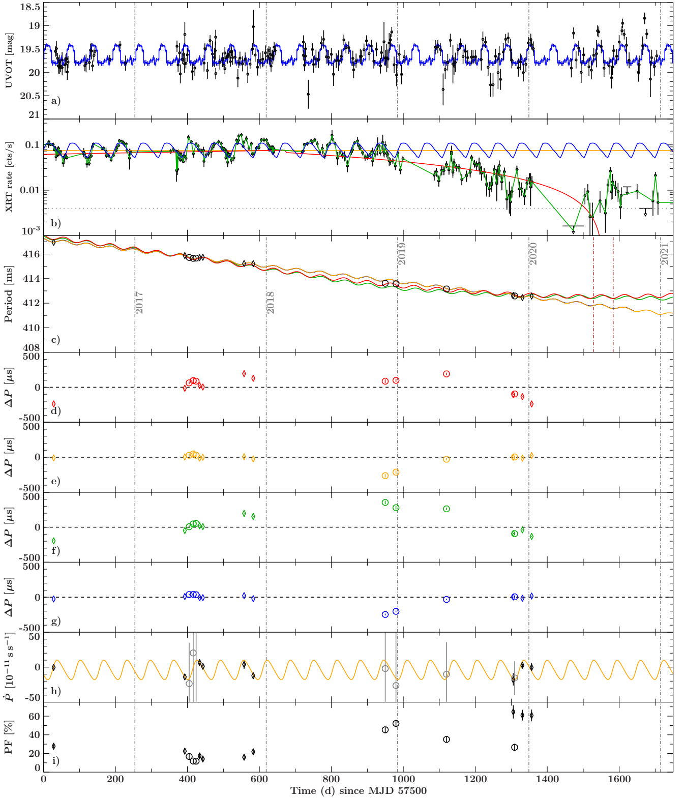
Fig. 2. a) Swift /UVOT light curve in the U -band. b) Swift /XRT lightcurve. The colored lines show the four different assumed flux evolutions, which are used as an input for the pulse period evolution: constant flux (orange), linear brightening and dimming trend (red), measured XRT lightcurve (green), and extrapolated X-ray super-orbital period profile (blue). The dotted line represents the estimated count rate at the Eddington limit. c) Pulse period evolution as measured by XMM-Newton (circles) and NuSTAR (diamonds). Superimposed are the best-fit models for the four different input lightcurves in the same colors as in panel b) . The brown dotted-dashed lines indicate the times of observations when no pulsations were seen. d) Residuals with respect to the linear brightening/dimming input, e) residuals with respect to a constant input, f) residuals with respect to the original lightcurve as input, and g) residuals with respect to the X-ray profile input. h) Measured (black and gray) and predicted (orange) pulse period derivative \dot{P} . The model is based on the constant flux model. i) Pulsed fraction in the 3–10 keV energy band. For details see text.
