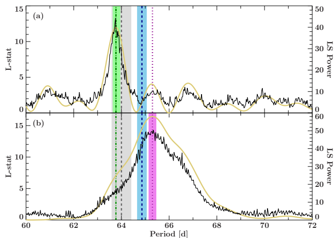
Fig. 1. Results from epoch folding (black left y -axis) and Lomb-Scargle periodogram (yellow, right y -axis) for the UV light-curve (top) and X-ray light-curve (bottom). The strongest UV period is marked by the green dotted-dashed line, the strongest X-ray period by the purple dotted line. The new orbital period is indicated by the blue dashed line, the old estimate of the orbital period is shown by the gray dashed line. The shading behind each period indicates their respective uncertainties (using the updated uncertainties for the old orbital period in gray).
