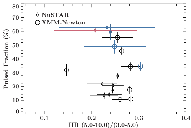
Fig. 6. Pulsed fraction in the 3–10 keV band as a function of the hardness ratio between the 5.0–10.0 keV and the 3.0–5.0 keV energy band. NuSTAR data are shown as diamonds, XMM-Newton data are shown as circles. Data from 2019 are shown in blue, data from 2020 in red.
