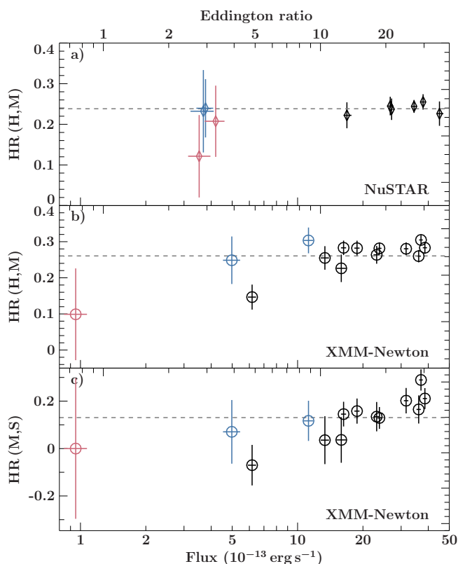
Fig. 4. Hardness ratio as a function of flux for all XMM-Newton and NuSTAR data. a) HR between the 5.0–10.0 keV and 3.0–5.0 keV energy band for NuSTAR . b) HR between the same bands as in (a) but for XMM-Newton . c) HR between the 3.0–5.0 keV and 0.5–1.5 keV band for XMM-Newton . Data taken in 2020 are shown in red, data from 2019 in blue, and all previous data in black. The dashed lines show the respective average HR for each instrument for all data before 2019. The top y -axis gives the flux as a fraction of the Eddington luminosity for a 1.4 M_{\odot} neutron star at a distance of 3.4 Mpc.
