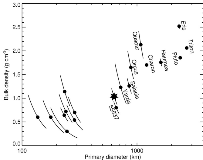
Fig. 3. Densities and sizes of transneptunian bodies, with \text{Gl}k\acute{u}n\|h\grave{o}m\acute{d}\acute{i}m\grave{a} indicated by a star. Other values are from Benecchi et al. (2010), Brown et al. (2010), Sicardy et al. (2011), Grundy et al. (2012), Stansberry et al. (2012), Brown (2013), Fornasier et al. (2013), Vilenius et al. (2012, 2014), Grundy et al. (2015), Brown and Butler (2017), McKinnon et al. (2017), and Ortiz et al. (2017).
