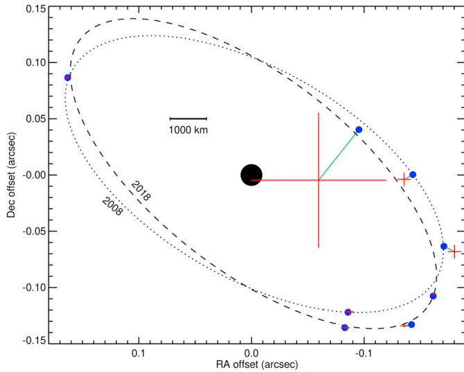
Fig. 2. Relative astrometry (points with error bars, red in on-line version) compared with model positions (small circles, blue in on-line version). Parallax shifts are illustrated by projecting the orbit to the sky plane at the time of the initial 2008 observation (dotted) and the final 2018 observation (dashed). (For interpretation of the references to color in this figure legend, the reader is referred to the web version of this article.)
