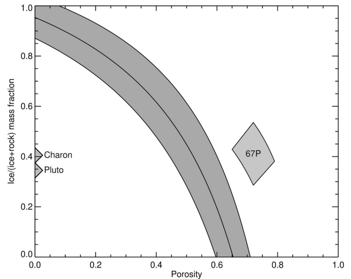
Fig. 4. Interpretation of the density of \text{Gl}k\acute{u}n\|h\grave{o}m\acute{d}\acute{i}m\grave{a} in terms of cold H 2 O ice ( \rho = 0.945 \text{ g cm}^{-3} ), rock ( \rho = 3 \text{ g cm}^{-3} ), and void space, compared with ice/(ice + rock) fractions for Pluto and Charon (assuming zero porosity) and for Churyumov-Gerasimenko.
