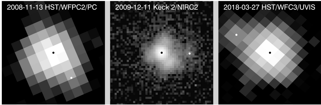
Fig. 1. Example frames from the 3 different telescope/instrument combinations we used to observe G!kún||hòmdímàG!kún||hòmdímà, logarithmically stretched to reveal the much-fainter G!ò'é !húG!ò'é !hú. Black and white dots mark best fit locations of G!kún||hòmdímà and G!ò'é !hú, respectively, from the ensemble of frames associated with each visit. Each panel is ½ arcsec on a side, with North up and East to the left. The spatial sampling of Keck NIRC2 is clearly superior, although the PSF exhibits a complicated and time-variable trefoil pattern in the Airy ring.
