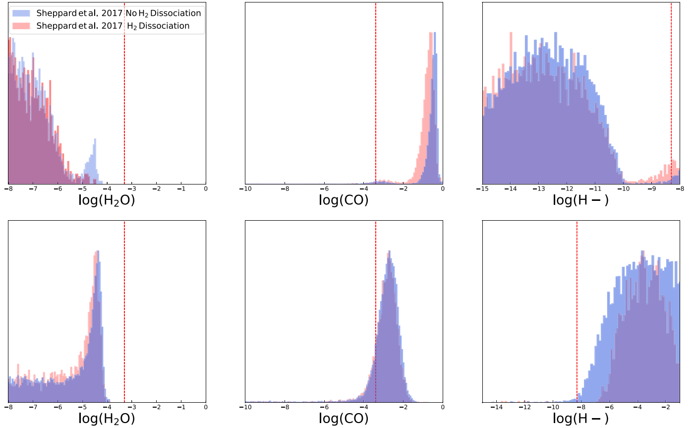
Figure 8. Posterior probability distributions of undissociated \text{H}_2\text{O} , CO, and \text{H}^- abundances for the retrievals of the Sheppard et al. (2017) data set. The red and blue histograms show the retrievals with and without \text{H}_2 dissociation, respectively. The top panels show the fiducial case where the \text{H}^- prior was restricted to be between \log(\text{H}^-) = -15 and -7 , whereas the bottom panel shows the wide prior case where the upper \text{H}^- prior was extended to \log(\text{H}^-) = -0 . The red dashed line shows the expected abundance for each of the species assuming chemical equilibrium with solar elemental abundances (Parmentier et al. 2018).
