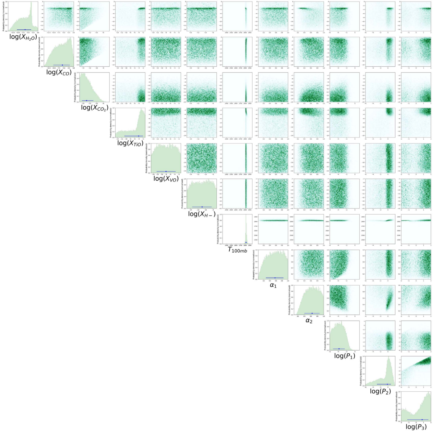
Figure 10. Posterior distribution for the fiducial retrieval of WASP-18b’s dayside spectrum from the Arcangeli et al. (2019) data set. We retrieve six parameters representing the undissociated abundance of the chemical species and six parameters parameterizing the P–T profile as discussed in Madhusudhan & Seager (2009).
