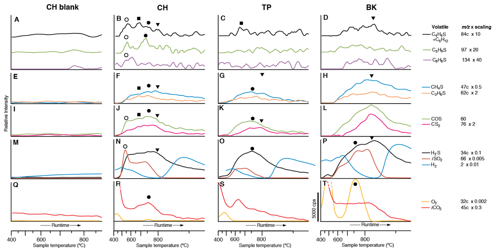
Fig. S1. EGA profiles for thiophenes (A-D), thiols and sulfides (E-L), other volatiles (M-P), and \text{O}_2 and \text{CO}_2 (Q-T) with peaks indicating possible combustion in Murray mudstone samples: Confidence Hills blank (CH blank), Confidence Hills (CH sample), Telegraph Peak (TP) and Buckskin (BK). Legend shows volatile, m/z , and scaling factor for each profile. Symbols mark correlations between panes in peak maxima within \pm 25^\circ\text{C} error due to signal smoothing. Axes and scaling factors are the same in Fig. 1-2 and S1-S6. Temperature placement of symbols are the same in Fig. 1-2, S1-S3. X-axis is scaled linearly to runtime to show the changing oven ramp rate and peak areas that scale to abundances. Y-axis scale bar in counts per second (cps) is for all panes. Profiles within panes are multiplied by scaling factors. All profiles are background subtracted, but profiles in A-D are shifted along the y-axis to show peaks clearly. "i", isotopologues in formulas. "c", corrections to profiles to remove other volatile contributions (11).
