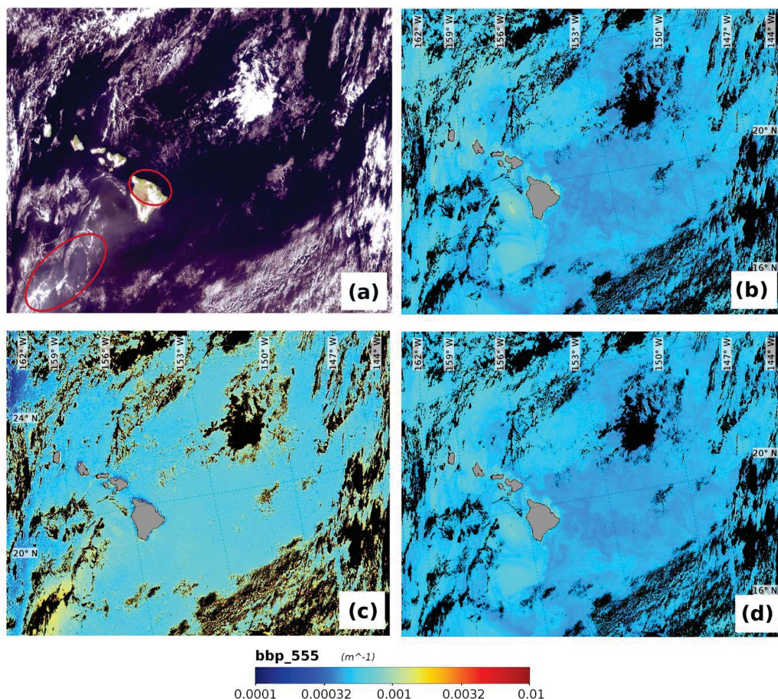
Figure 5: SeaWiFS imagery of the Hawaiian Island region of the North Pacific Ocean captured on the 1 December 2000. Panel a is a Quasi-true color image. Panels b, c, and d are of b_{bp}(555) derived using the LH, GIOP, an Huot models, respectively. Red ellipses denote regions where the GIOP exhibits artifacts in the retrievals. Clouds contaminated pixels are masked in black.
