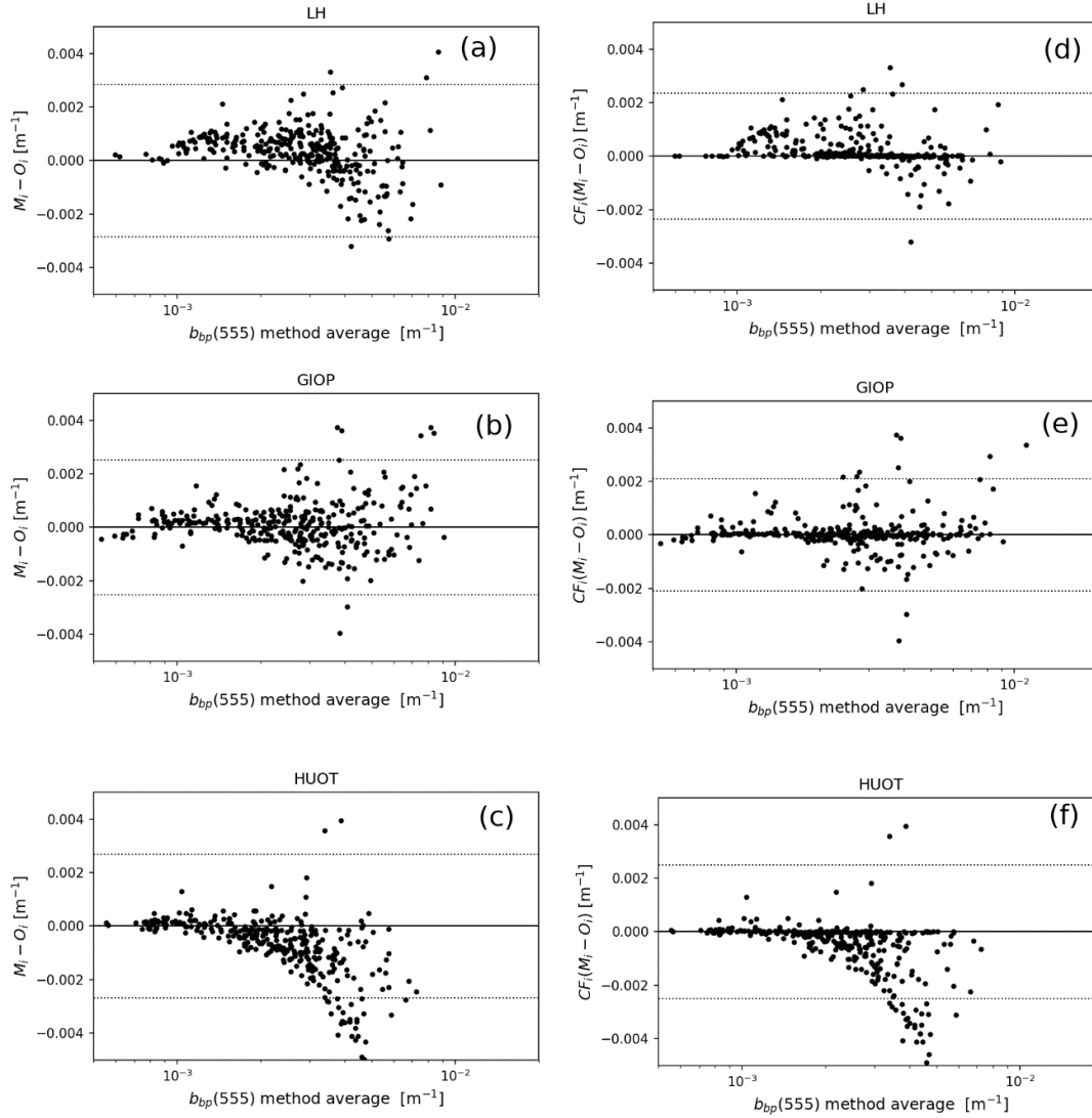
Figure 3: Bland-Altman plots of differences between modelled and observed b_{bp}(555) varying with the method average values of b_{bp}(555) . Subplots a, b, c correspond to LH, GIOP, and Huot models, respectively. Subplots d, e, and f are Bland-Altman plots with corresponding differences for the LH, GIOP, and Huot models, respectively. Dashed horizontal lines represent 97.5% confident interval about zero.
