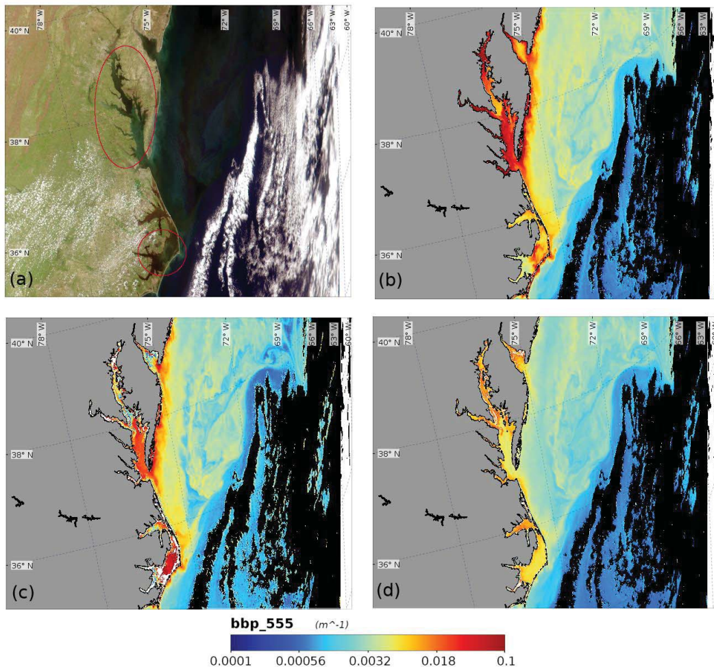
Figure 6: SeaWiFS imagery of the Chesapeake Bay region captured on the 28 April 2003. Panel a is a Quasi-true color image. Panels b, c, and d are of b_{bp}(555) derived using the LH, GIOP, and Huot models, respectively. Red ellipses denote spatial features visible in the quasi-true color image that LH model resolves. Clouds contaminated pixels are masked in black.
