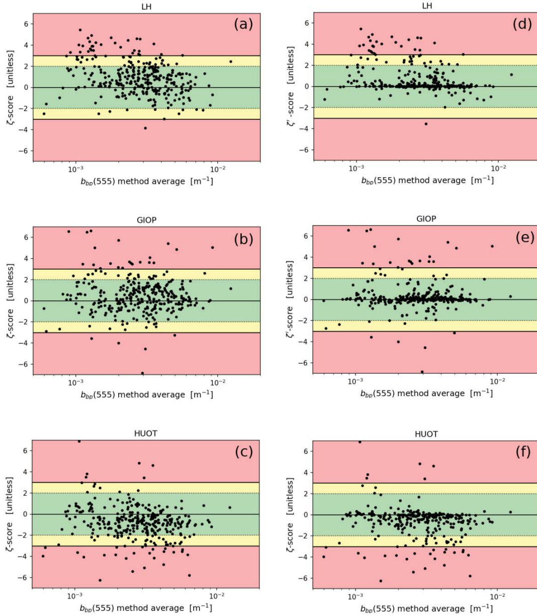
Figure 4: Zeta score plots comparing modelled and observed b_{bp}(555) varying with the method average values of b_{bp}(555) . Subplots a, b, c correspond to LH, GIOP, and Huot models, respectively. Subplots d, e, and f use corrected zeta scores for the LH, GIOP, and Huot models, respectively.
