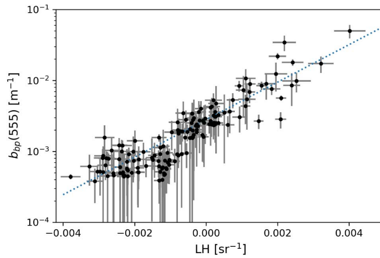
Figure 1: Scatter plot of LH vs b_{bp}(555) shows a strong log-linear relationship. Gray bars represent estimated standard uncertainties.
