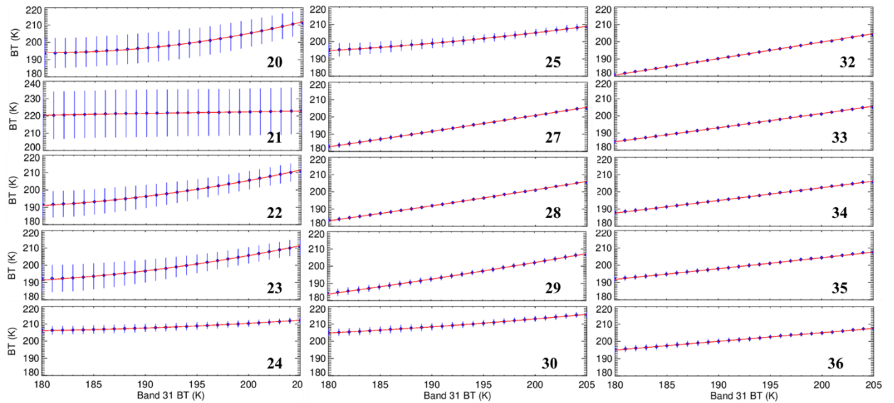
Figure 9a. The BT measurements as a function of the TEB 31 BTs (blue) over nighttime qDCC for January 2019, and the empirical model for the reference dependency (red) for Aqua MODIS TEBs. Due to the large number of DCC samples, the BTs are binned every temperature degree. The average binned BT and its standard deviation are plotted.
