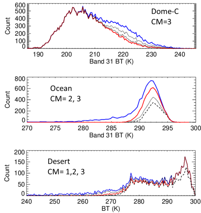
Figure 3. Terra TEB 31 BT measurements distribution over Dome-C, the ocean, and the desert under different CM thresholds. The blue curves represent all the nighttime measurements, and the other three curves are CM ranges from 3 to 1, 3 to 2, and 3 only. The red curves denote the CM-filtered measurements used in this work.
