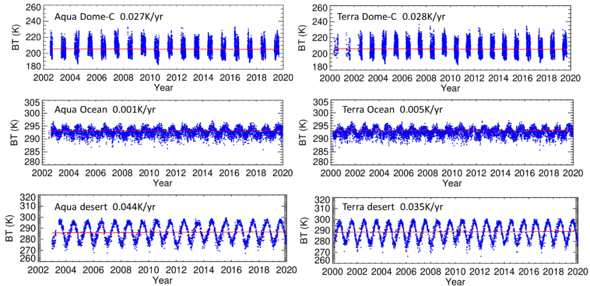
Figure 2. The trending and change rate of MODIS band 31 BT measurements over Dome-C, ocean, and desert.
