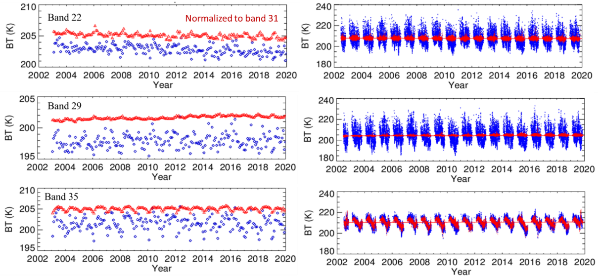
Figure 10. (Left) The entire mission BT trends for Aqua MODIS TEBs 22, 29, and 35 over the nighttime qDCC. The blue symbols define BTs averaged over each month, while the red symbols represent the average BTs after normalization. The normalization band 31 BT is set to 200 K for every month. (Right) Aqua mission BT trends for TEBs 22, 29, and 35 over Dome-C during nighttime. The blue symbols represent Dome-C MODIS BTs, while the red symbols define the MODIS BTs after being normalized using the TEB 31 BTs as reference.
