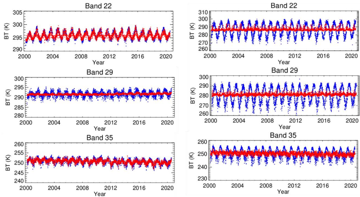
Figure 11. (Left) Terra mission BT trends for TEBs 22, 29, and 35 over the ocean site during nighttime. The blue symbols represent the ocean site MODIS BTs, while the red symbols define the MODIS BTs after being normalized using the TEB 31 BTs as reference. (Right) Terra mission BT trends for TEBs 22, 29, and 35 over the desert site during nighttime. The blue symbols represent the desert site MODIS BTs, while the red symbols define the MODIS BTs after being normalized using the TEB 31 BTs as reference.
