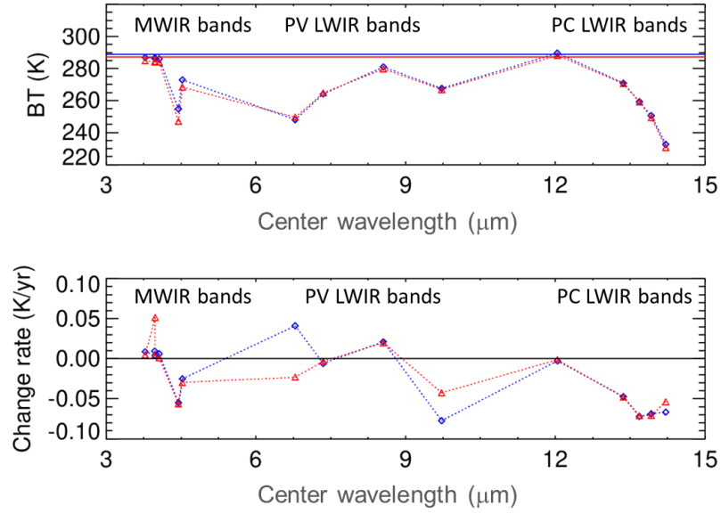
Figure 12. (Top) BT for each band corresponding to the reference BT of band 31 over the desert site. The horizontal lines represent the band 31's BT. (Bottom) The mission-long BT change rate for each band. The BT and BT change rates are plotted at each band's center wavelength. Blue and red define Terra and Aqua MODIS, respectively.
