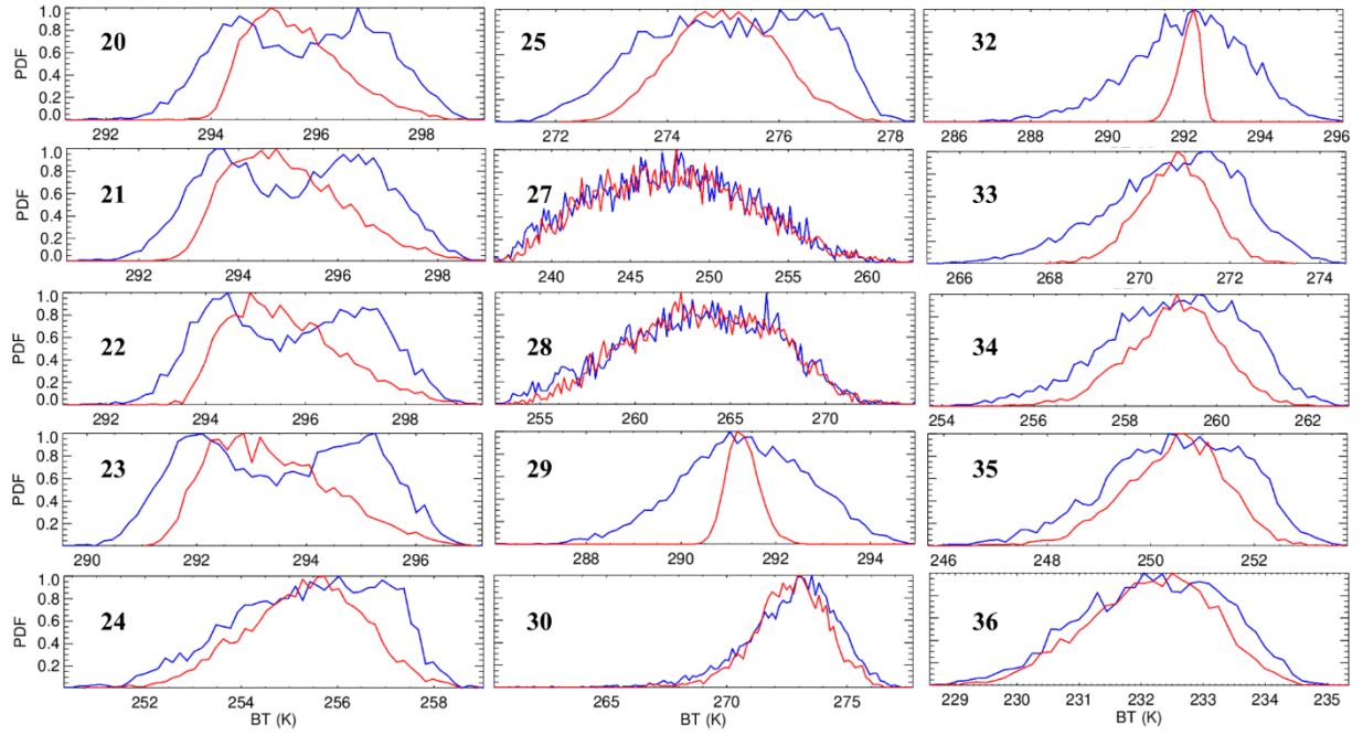
Figure 6b. PDF for MODIS BTs (blue) and its PDF after normalization (red) for all TEB over ocean during nighttime.
