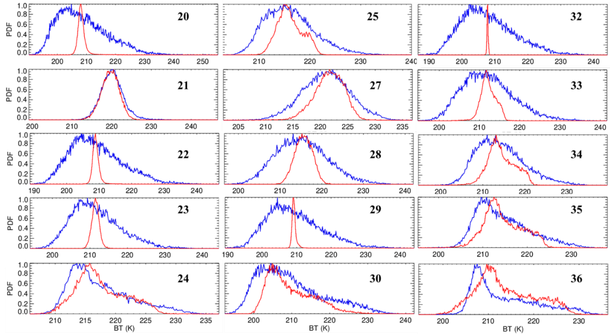
Figure 5b. PDF for MODIS BTs (blue) and its PDF after normalization (red) for TEB over Dome-C during nighttime.
