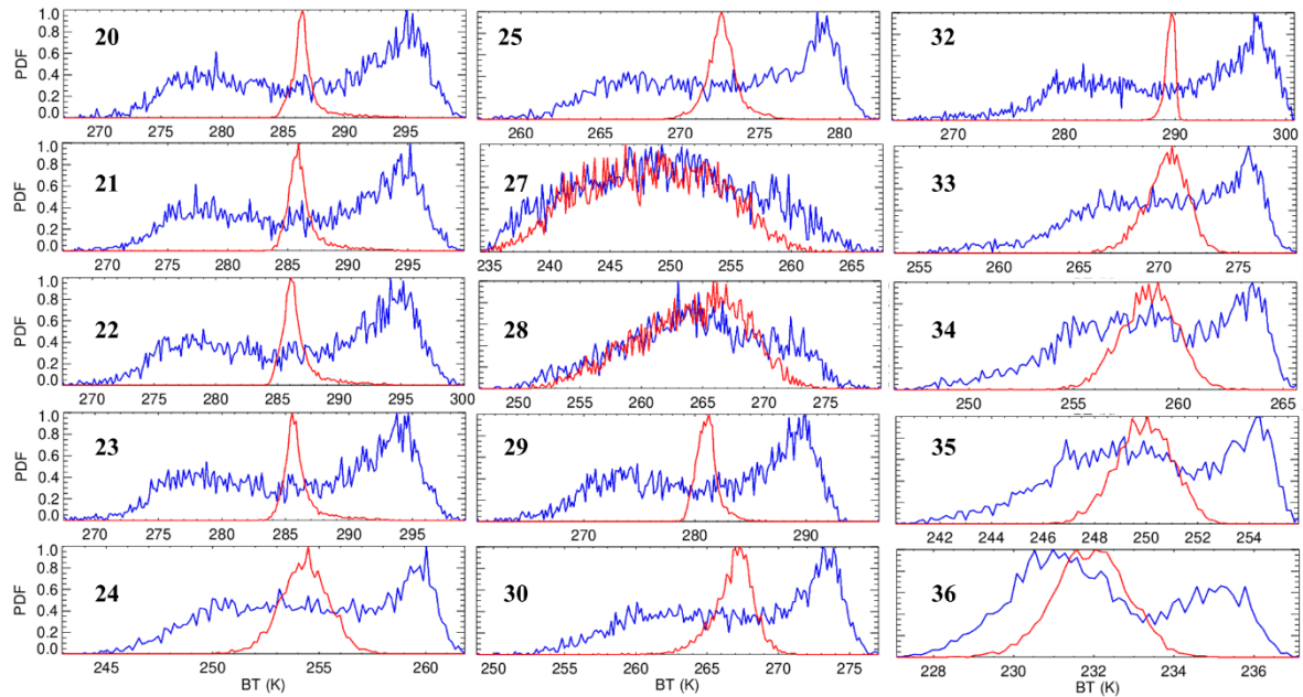
Figure 7b. PDF for MODIS BTs (blue) and its PDF after normalization (red) for all TEB over desert during nighttime.
