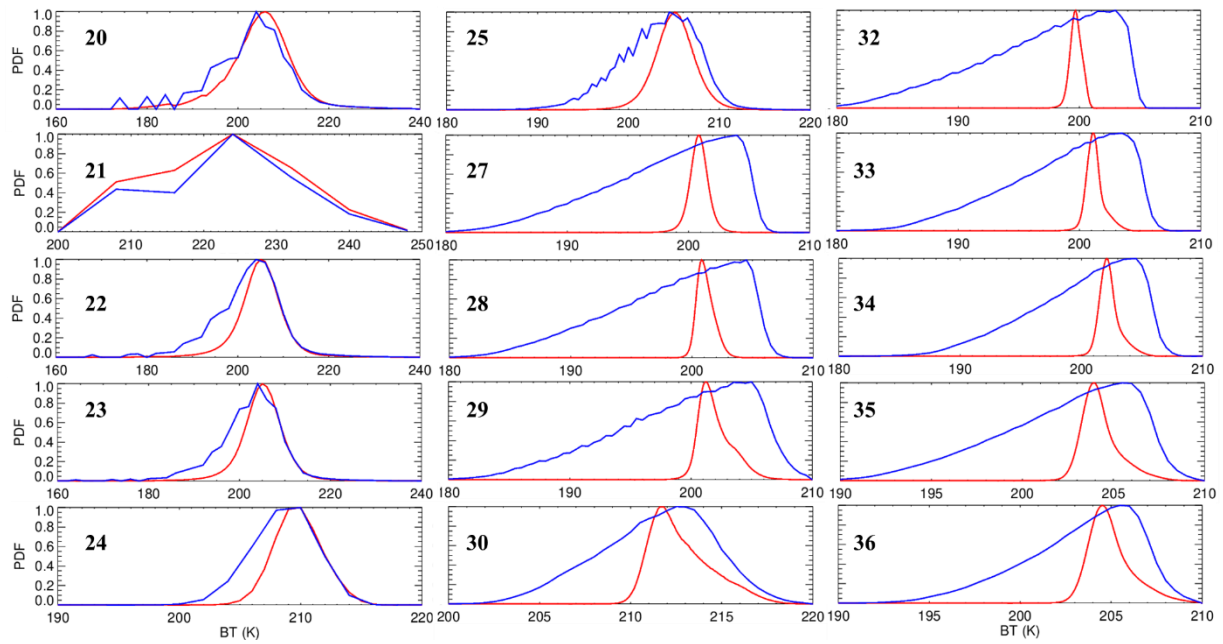
Figure 9b. PDF of bands BTs before (blue) and after (red) normalization. The normalization BT is set to constant 200 K for the band 31 reference.
