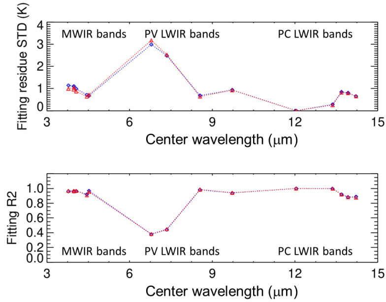
Figure 4. (Top) Standard deviation of the absolute fitting residuals for the normalization model for the desert measurements and each band. In order to show the spectral features, the STD is shown as a function of each band's center wavelength. (Bottom) Fitting model's R^2 over desert measurements for each band with respect to band 31. Samples from the entire satellite missions are used. Band 31 is not shown in either chart, since it is the reference. Blue and red define Terra and Aqua, respectively.
