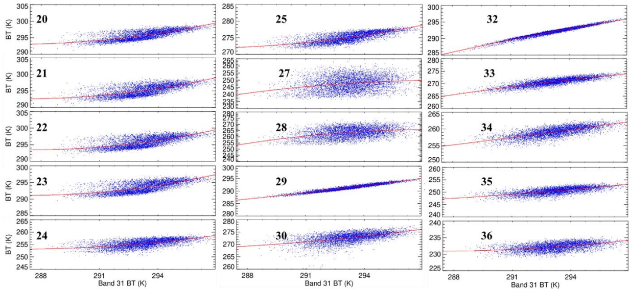
Figure 6a. Terra MODIS mission-long BTs as a function of the MODIS band 31 BTs (blue) and its empirical model (red) for all TEB over the ocean site during nighttime.
