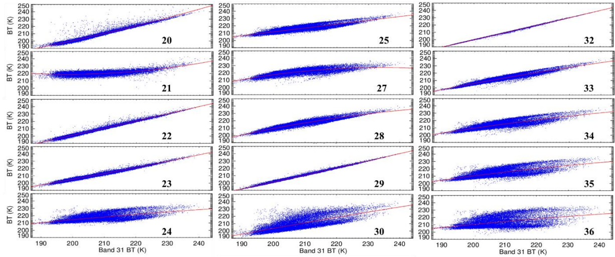
Figure 5a. Terra MODIS mission-long BTs as a function of the MODIS band 31 BTs (blue) and their empirical model (red) over Dome-C during nighttime.
