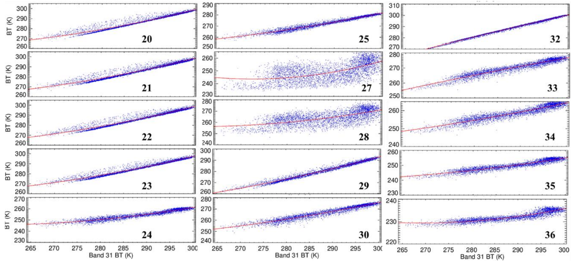
Figure 7a. Terra MODIS mission-long BTs as a function of the MODIS TEB 31 BTs (blue) and its empirical model (red) over the desert site during nighttime.
