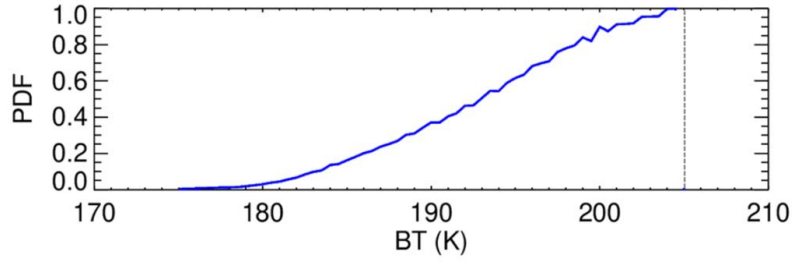
Figure 8. Aqua TEB 31 BTs PDF over nighttime qDCC for January 2019. The dashed line indicates the 205 K BT used for DCC pixel identification.
