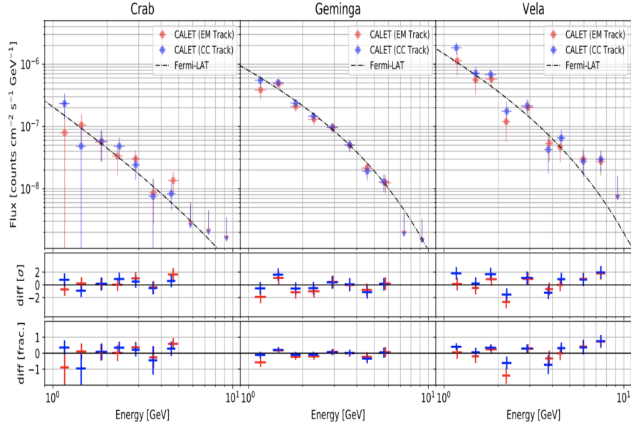
FIG. 5: Source spectra for Crab, Geminga, and Vela as measured by CALET [23]. The lower panels in each plot show the difference between the CAL observations and the Fermi-LAT parameterization in units of CAL error (top) and fractional difference (bottom).
