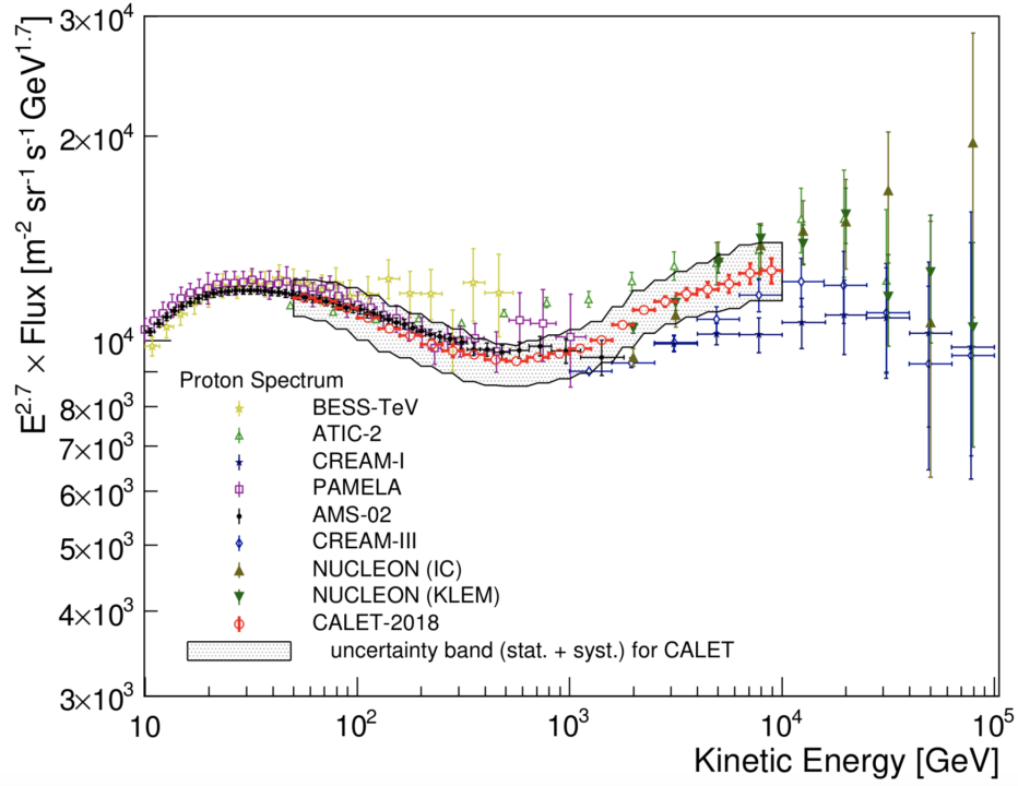
FIG. 2: Cosmic-ray proton spectrum measured by CALET from 50 GeV to 10 TeV [18]. The gray band indicates the quadratic sum of statistical and systematic errors. Also plotted are recent direct measurements [13, 19, 29–32].
