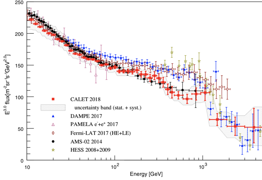
FIG. 1: Cosmic-ray all-electron spectrum measured by CALET from 10.6 GeV to 4.75 TeV [9]. The width of each bin is shown as a horizontal bar, the statistical errors as vertical bars, while the gray band indicates the quadratic sum of statistical and systematic errors (not including the uncertainty on the energy scale). Also plotted are direct measurements in space including [10–12, 26] and from ground-based experiments [27, 28].
