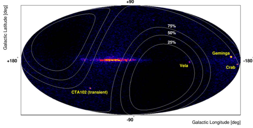
FIG. 4: Gamma-ray sky map shown in a Mollweide projection of galactic coordinates [23]. White contours show the relative level of exposure compared to the maximum on the sky. The Crab, Geminga, and Vela pulsars are clearly visible, as is a flare of the AGN CTA 102.
