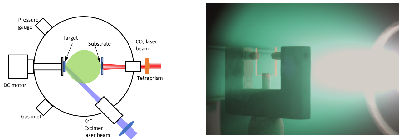
Fig 1. Schematic (left) and photograph of the PLD setup (right).
