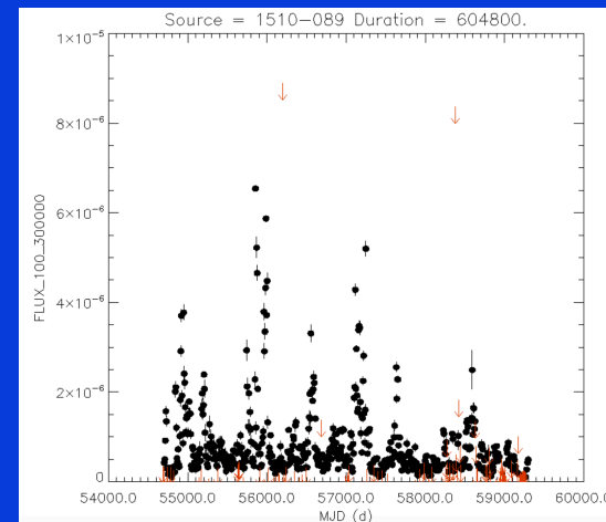
Multi-year light curve of a blazar.
