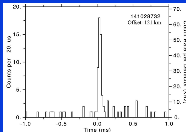
Terrestrial Gamma-ray Flash
