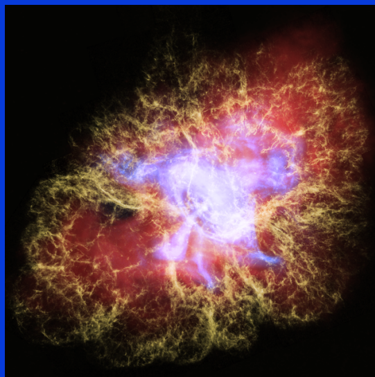
IR-Optical-X-ray image of the Crab Nebula. Gamma rays can barely resolve the nebula as spatially extended.
