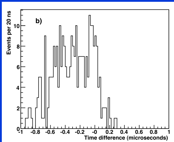
Fermi-LAT ground test comparing onboard times with an independent GPS system.
