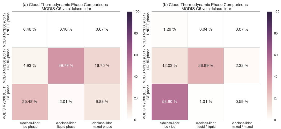
Figure 5: MYD06 C6.1 cloud thermodynamic phase compared to 2B-CLDCLASS-lidar cloud phase: (a) monolayer clouds (about 63% of the dataset), and (b) multilayer clouds having the same phase (about 10% of the co-located dataset). Here, mono/multilayer clouds are defined by 2B-CLDCLASS-lidar.
