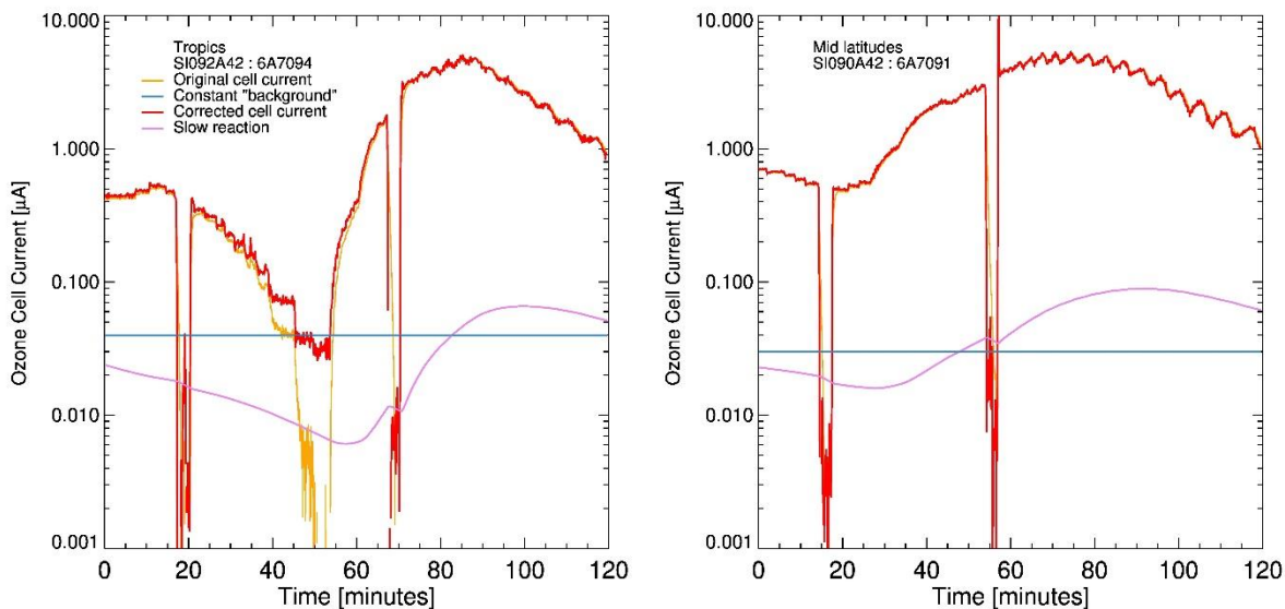
680 Figure 4: Cell current components of the tropical and mid-latitude simulations shown in Figure 3. Red lines: Fast cell current contribution. Purple lines: Slow reaction contribution. Orange lines: Originally measured cell current minus constant background. Light blue lines: Constant background.
