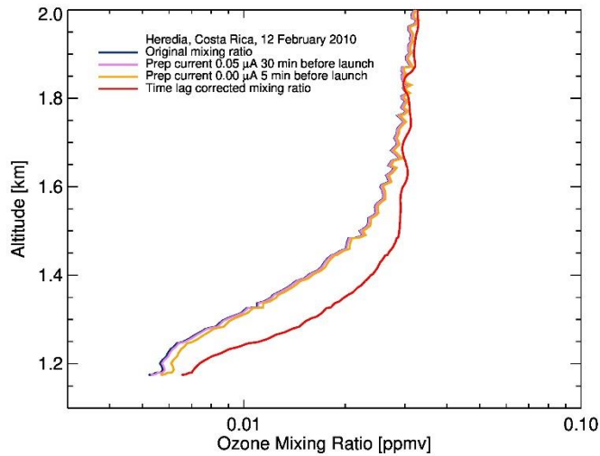
Figure 10: Boundary layer detail of the ozone profile shown in Figure 7. The different assumptions for the preparation current prior to launch have only been corrected for the slow reaction path, but not time lag corrected for the fast reaction path.
