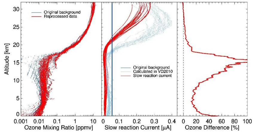
Figure 13: Left: Original and reprocessed CEPEX ozonesonde profiles. Center: Original constant background, reprocessed background following VD2010 and slow reaction contribution. Right: Difference between reprocessed and original ozonesonde profiles.
