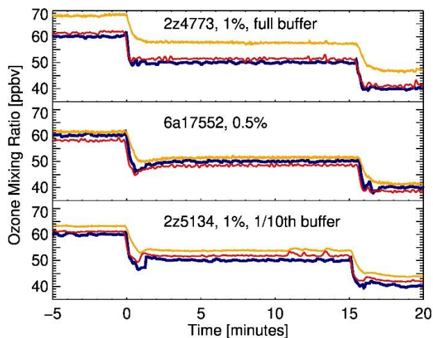
665 Figure 2: Response of three ECC sondes using three different solutions during two plateau changes. The color-coding is the same as in Figure 1. The reference time is defined as the time, when the TEI 49C drops below 59 ppb during the first change of plateaus.
