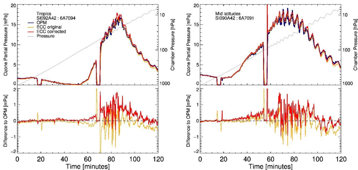
670 Figure 3: Reprocessing of JOSIE 2000 environmental simulation chamber ozonesonde data. Left: Tropical simulation; right: mid-latitude simulation. Blue lines in top panels: ozone photometer measurements. Orange lines: originally processed ozonesonde measurements. Red lines: Reprocessed ozonesonde measurements using the separation of slow and fast reaction contribution. Thin grey line: chamber pressure.
