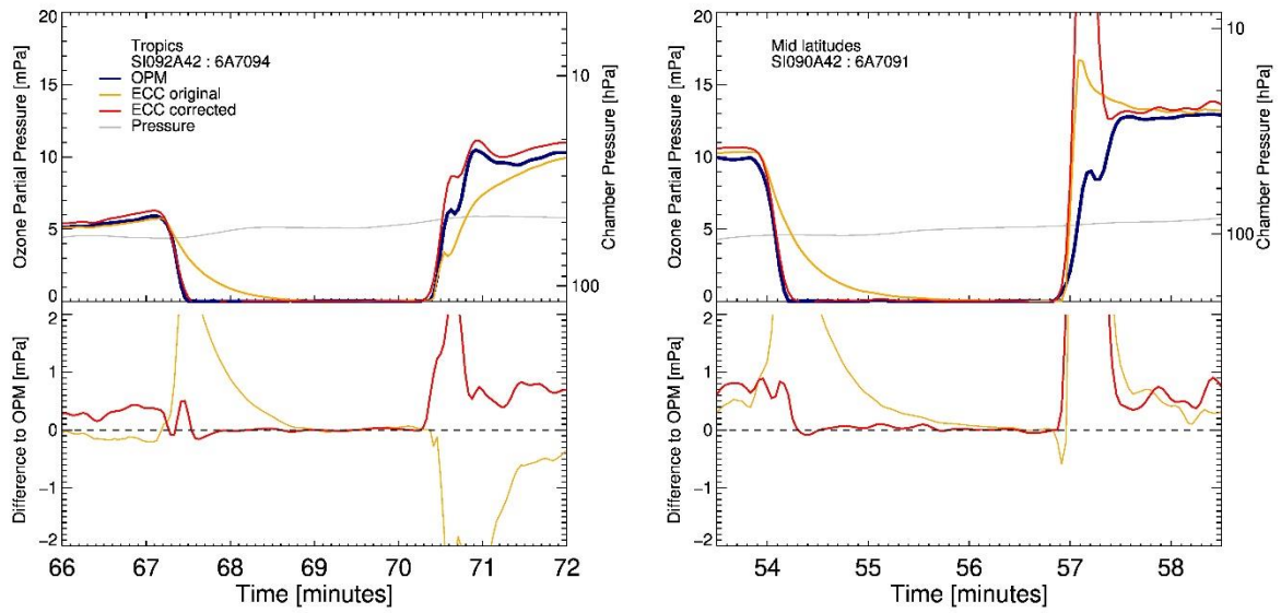
685 Figure 5: Same data as Figure 3 showing the time response periods after about 1 hour. Left: Tropical simulation; Right: Mid-latitude simulation. The differences are shown as absolute differences, since the reference achieves zero ozone.
