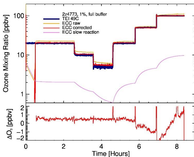
660 Figure 1: Top: Ozone mixing ratio generated by the TEI 49C ozone calibrator (blue) and measured by the ECC (original processing in orange, time response corrected in red). The contribution of the slow reaction is shown in purple. Bottom: Difference of corrected ECC measurements and TEI 49C ozone concentration.
