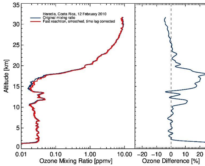
695 Figure 7: Ozone profile measured at Costa Rica. The original profile is shown in blue, the reprocessed profile in red. The right hand profile shows the difference of the reprocessed profile minus the original profile.
