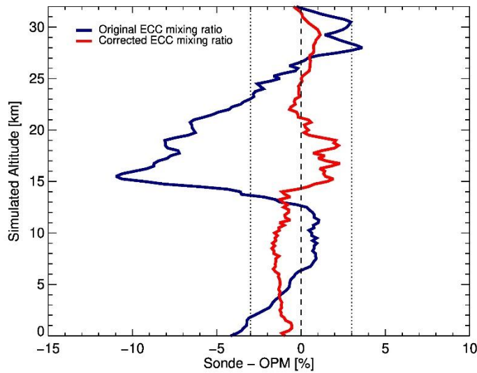
690 Figure 6: Comparison between ECC and OPM mixing ratio in 77 simulation experiments during JOSIE 2017. The originally reported difference is shown in blue; the difference calculated using the corrected data is shown in red. Dotted lines indicate \pm 3\% .
