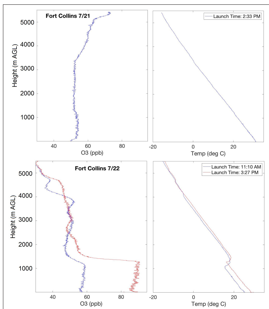
Figure 3: \text{O}_3 and temperature profiles on July 21 and 22, 2014 at Ft. Collins. DOI: https://doi.org/10.1525/elementa.345.f3
