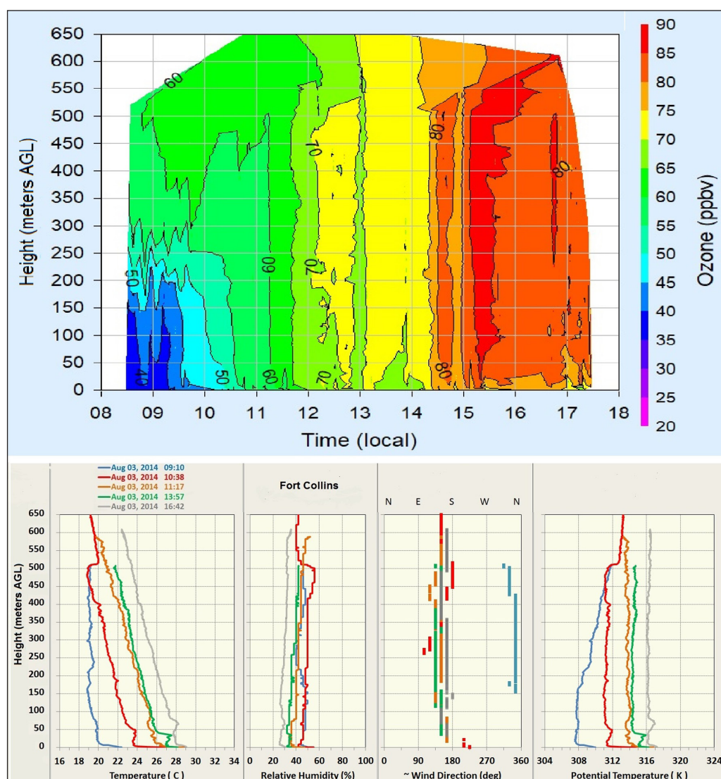
Figure 5: Height/Time cross-section of O_3 at Ft. Collins West on August 3, 2014. Height/Time cross-section of O_3 mixing ratio from tethered sonde profiles at Ft. Collins West on August 3, 2014 (upper panel). Selected meteorological profiles (lower panel). DOI: https://doi.org/10.1525/elementa.345.f5
