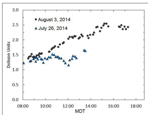
Figure 6: Integrated O_3 from each profile at Ft. Collins West from tethered sonde measurements. Integrated O_3 from each profile at Ft. Collins West from tethered sonde measurements on July 26 and August 3, 2014 between the Surface – 400 m (See tabulated data in Table S1). DOI: https://doi.org/10.1525/elementa.345.f6
