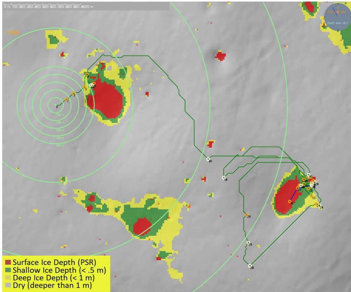
Figure 5-2 Notional traverse at the Nobile study region. The landing site is at the center of the smaller light green circles at the upper left of the image (each of these light green circles are 100 meters apart). The colored areas indicate ISR types (see key).
