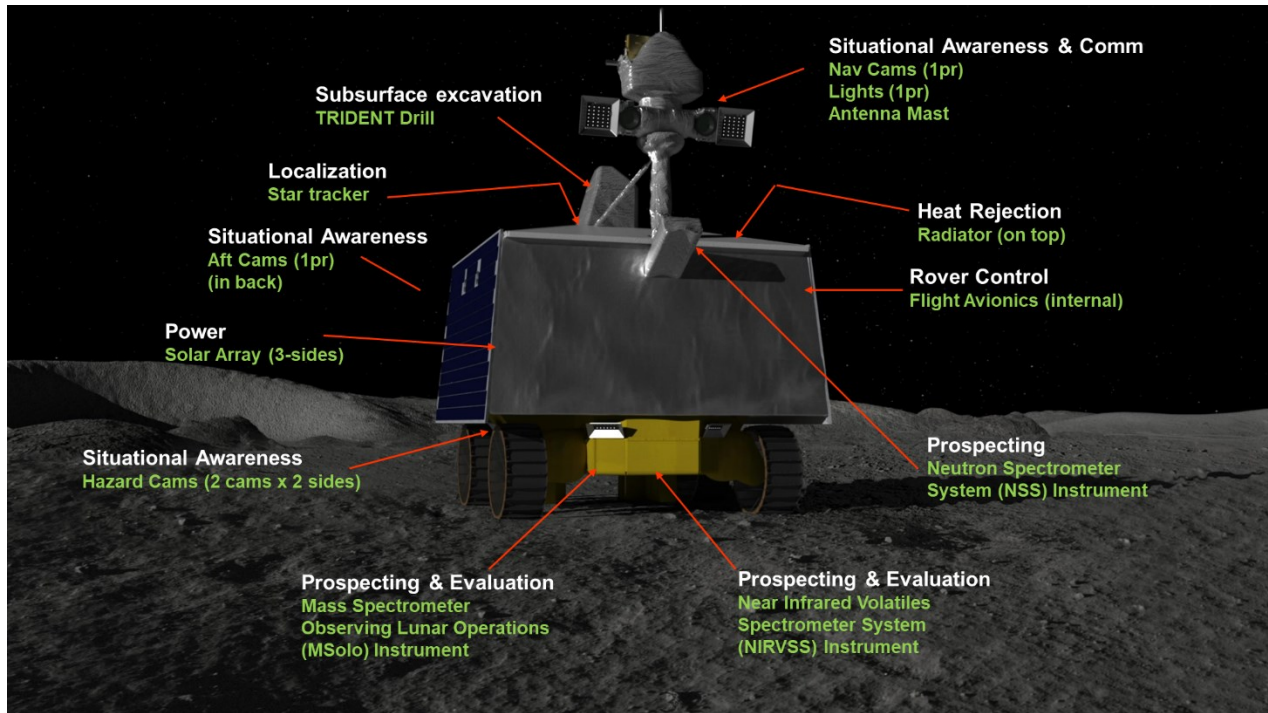
Figure 3-1. VIPER and its navigation, prospecting, surface and subsurface assay science instruments.
