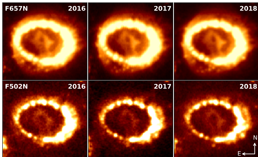
Figure 6. WFC3 narrow-band images. The top row shows F657N, for which all emission sites are dominated by \text{H}\alpha . The bottom row shows F502N, where the ER emission is dominated by [\text{O III}] and the ejecta emission by \text{Fe I } \lambda 5007 . The emission in the south-east corners is due to Star 3 (see Figure 1). The images have been scaled by an asinh function in order to highlight the weak emission outside the ER. The FOV is 2''.7 \times 2''.4 .
