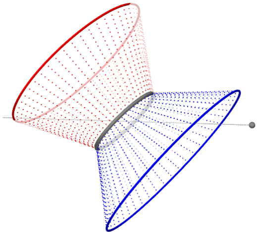
Figure 2. A 3D view of the ring system surrounding SN 1987A. The ER is shown in grey, the NOR in red and the SOR in blue. The dashed lines represent hypothetical material connecting the ER and ORs. The grey sphere and line show the position of the observer and the line of sight, respectively.
