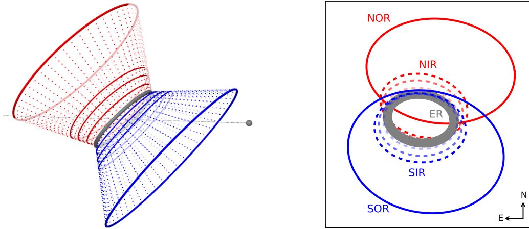
Figure 15. Left: 3D model for the ring nebula surrounding SN 1987A. The ER is shown in grey, the NOR in red and the SOR in blue. The model assumes that there is material connecting the ER and ORs, as illustrated by the red and blue dashed lines. The three additional rings on each side show where spherically symmetric freely expanding ejecta with velocities of 7000, 8000 and 9000 \text{km s}^{-1} would intersect this material at 11,500 days in 2018. These interacting regions make up the intermediate rings (IRs) in the images. The grey sphere and line show the observer and the line of sight, respectively. Right: Projection of the ring system on the sky. The material connecting the rings has been omitted for clarity. The FOV is 5''.0 \times 5''.5 .
