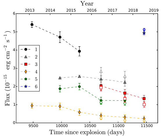
Figure 13. Light curves for six of the new spots that have appeared outside the ER. The numbers are the same as in Figure 5. Filled and open symbols show fluxes in the R band and in F657N, respectively. All the observations were made with WFC3, but the R-band fluxes have been normalized to WFPC2 using the correction factor in Table 3 in order to allow for comparison with the light curves of the ER. The F657N fluxes have been multiplied by a factor of 1.6.
