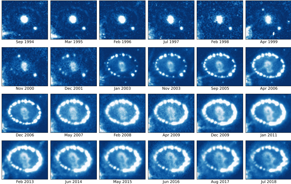
Figure 4. Same as Figure 3, but for the B band.
