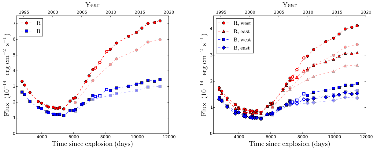
Figure 11. Left: Light curve of the inner ejecta. The flux was measured in an expanding, circular aperture with radius 2800 \text{ km s}^{-1} in the plane of the sky (see Figure 9). Right: Same, but separately for the eastern and western parts of the ejecta. Note the brightening of the western ejecta at late times. The statistical error bars are always similar in size or smaller than the plot symbols. The light colored (semi-transparent) points have been corrected for scattered light from the ER using the models described in Appendix B. The late WFC2 fluxes are uncertain because the images are affected by CTE losses, but no corrections have been applied (see text for details). These points are plotted with open symbols.
