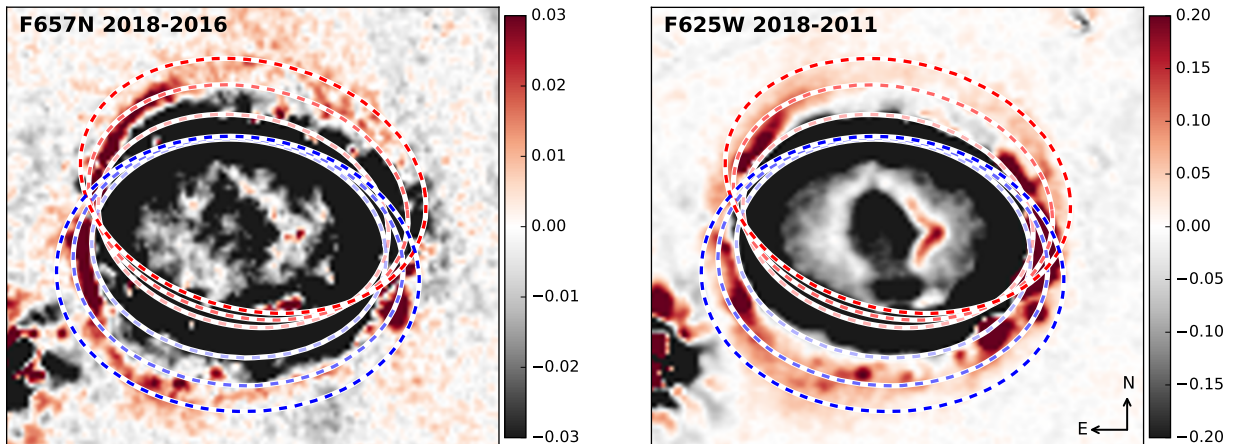
Figure 16. Projection of the IRs from the model in Figure 15, shown superposed on difference images in \text{H}\alpha (left, 11,500 – 10,700 days, 2018 – 2016) and the R band (right, 11,500 – 8700 days, 2018 – 2011). The blue rings are on the near side of the ER and the red ones on the far side. The southern parts of the red rings would thus be obscured by the ER, as shown in Figure 15. For each color, the three gradually darker rings correspond to ejecta velocities of 7000, 8000 and 9000 \text{km s}^{-1} , respectively. The residuals in the south-east corners are due to Star 3 (see Figure 1). The unit for the color bar is \text{counts s}^{-1} per 0''.025 pixel. The FOV is 2''.6 \times 2''.7 .
