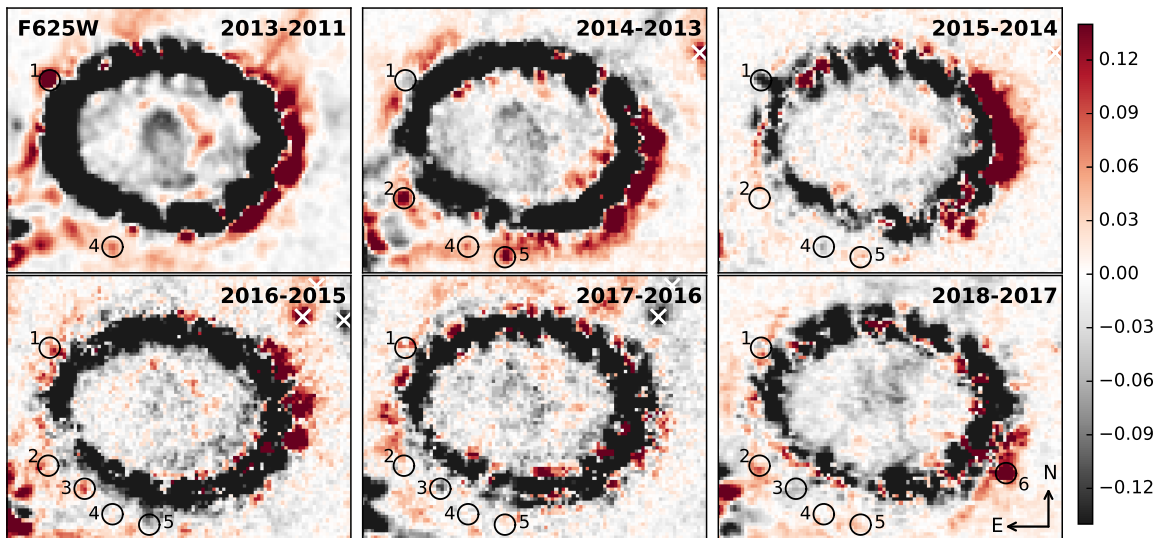
Figure 5. WFC3/F625W differences images. All images except the first one are separated by one year. The spots marked by white crosses to the north-west of the ER are ghost reflections. There are also diffraction spikes and other residuals from Stars 2 and 3 in the north-west and south-east corners, respectively (see Figure 1). We provide flux measurements for the six labelled spots outside the ER in Section 7. The numbering of the spots is done anti-clockwise from north. The unit for the color bar is \text{counts s}^{-1} per 0''.025 pixel. The FOV is 2''.5 \times 1''.9 .
