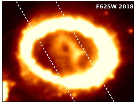
Figure 19. Slit position for the VLT/UVES observation at 11,200 days (2017) shown superposed on the WFC3/F625W image from 11,500 days (2018). The image has been scaled by an asinh function in order to highlight the weak emission outside the ER. The FOV is 2''.7 \times 2''.1 .
