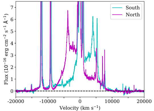
Figure 14. VLT/UVES H \alpha line profiles from 11,200 days (2017). Spectra from the northern and southern halves of the slit are shown in magenta and cyan, respectively. The narrow lines are from slow shocks into the ER, while the extremely broad profiles extending to \sim 9000 \text{ km s}^{-1} are from the RS. The features at \sim \pm 4000 \text{ km s}^{-1} originate from the RS just inside the ER.
