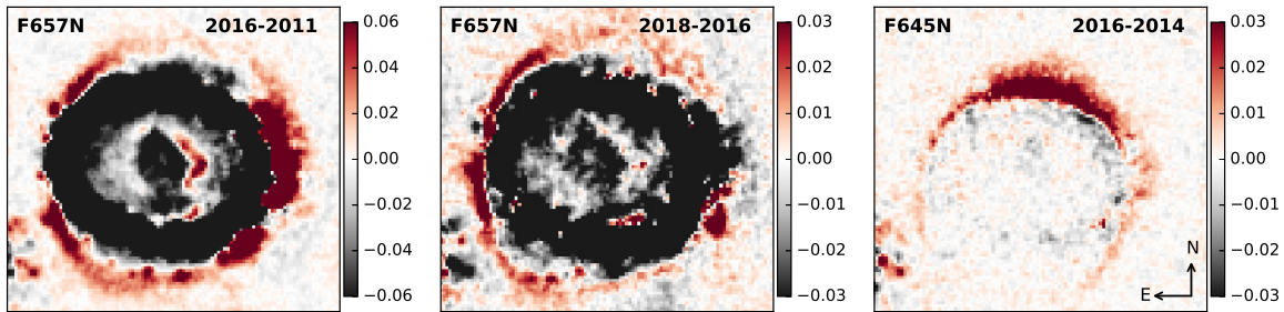
Figure 7. Differences of narrow-band images in H\alpha . The left and middle panels show differences in F657N between 10,700 – 8700 days (2016 – 2011) and 11,500 – 10,700 days (2018 – 2016), respectively. This filter covers H\alpha in the velocity range [-3500, +3600] \text{km s}^{-1} . The right panel shows the difference in F645N (blueshifted H\alpha in the range [-7900, -2700] \text{km s}^{-1} ) between 10,700 – 10,000 days (2016 – 2014). The residuals in the south-east corners are due to Star 3 (see Figure 1). The unit for the color bar is counts \text{s}^{-1} per 0''.025 pixel. The FOV is 2''.7 \times 2''.4 .
