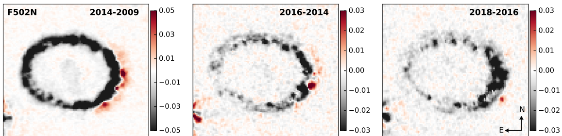
Figure 8. Differences of F502N [O III] images. The epochs from left to right are 10,000 – 8300 days (2014 – 2009), 10,700 – 10,000 days (2016 – 2014) and 11,500 – 10,700 days (2018 – 2016). The residuals in the south-east corners are due to Star 3 (see Figure 1). The unit for the color bar is counts \text{s}^{-1} per 0''.025 pixel. The FOV is 2''.7 \times 2''.4 .
