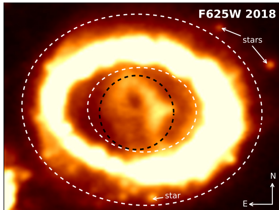
Figure 9. WFC3/F625W image from 11,500 days (2018) together with the apertures used to produce the light curves. The dashed, white and black lines show the apertures for the ER and the ejecta, respectively. The aperture for the ejecta was expanded over time in order to always cover the same part of the inner ejecta. The image has been scaled by an asinh function in order to highlight the weak emission outside the ER. The FOV is 2''.7 \times 2''.1 .
