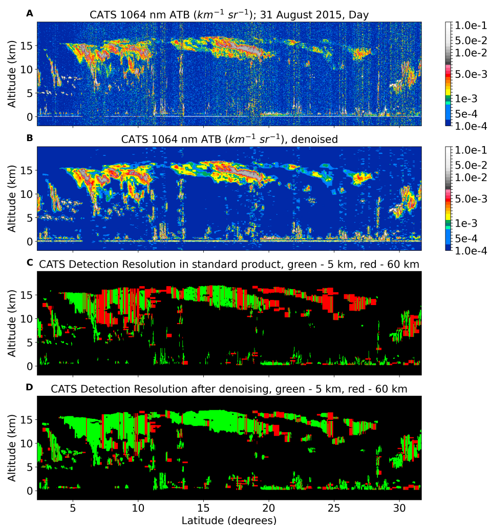
Figure 7. The CATS 1064 nm attenuated total backscatter (ATB) averaged horizontally to 5 km (A) and then after the wavelet denoising algorithm was applied (B), as well as the layers reported in the V3-00 data products before the denoising (C) and after (D) detected at both 5 km (green) and 60 km (red) for a case on 31 August 2015.
