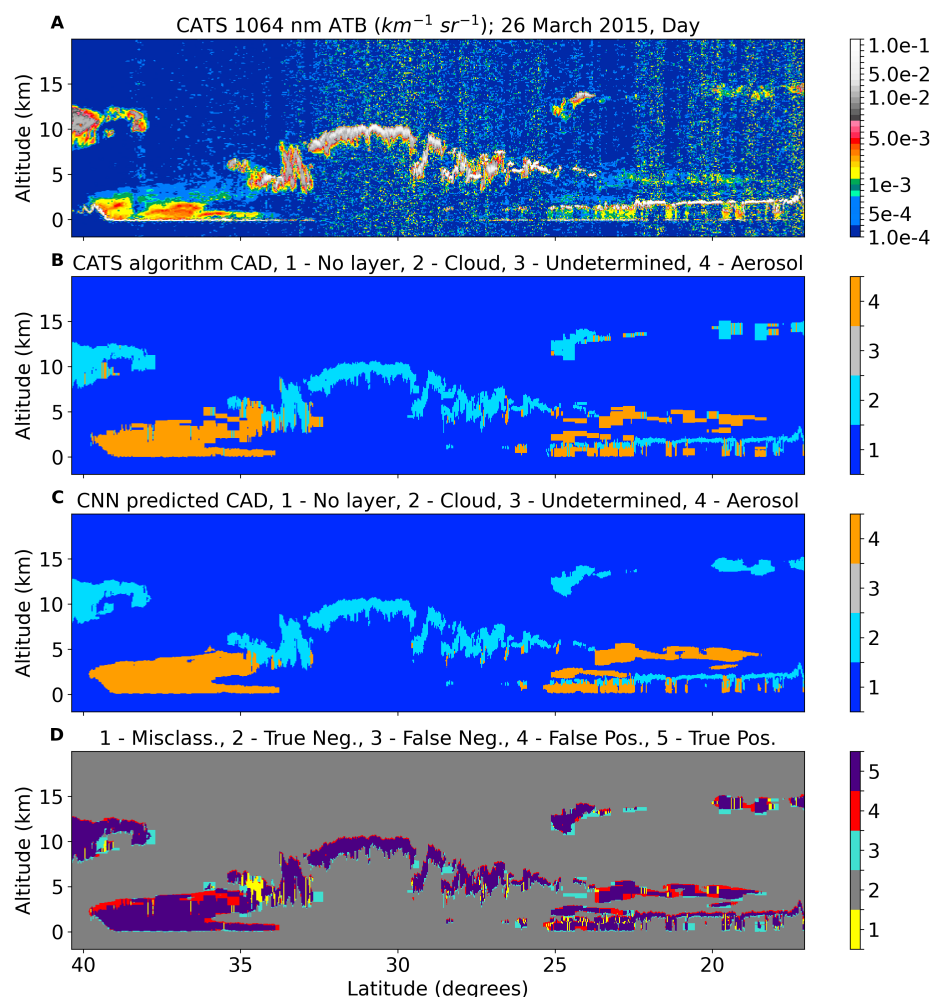
Figure 8. The CATS 1064 nm attenuated total backscatter averaged horizontally to 5 km (A) the cloud-aerosol classification designated by the traditional algorithms (B) the predicted classifications from the CNN (C) with a comparison image between the two (D) for a case on 26 March 2015. Yellow in (D) is a misclassification between cloud and aerosol feature types.
