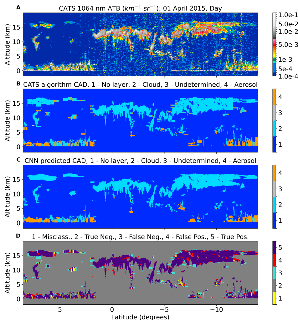
Figure 9. The same four plots as Figure 8 for a case on 1 April 2015.
