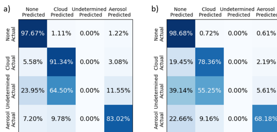
Figure 12. Confusion Matrices for CNN predictions ( x -axis) and actual layer typing from CATS operational data products ( y -axis) from September 2015 during (a) Nighttime and (b) Daytime.
