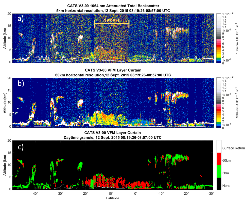
Figure 3. The CATS 1064 nm attenuated total backscatter (ATB) averaged horizontally to 5 km (a) and 60 km (b), as well as the layers reported in the V3-00 data products (c) detected at both 5 km (green) and 60 km (red) for a case on 12 September 2015 over bright deserts of the Middle East.
