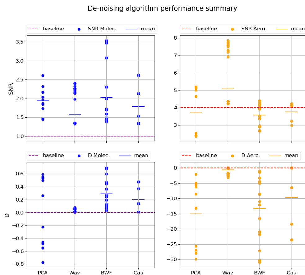
Figure 5. A comparison of denoising techniques on simulated photon-counting lidar data. The Signal-to-Noise Ratio (SNR) and Deviation (D) calculated for both molecular (blue) and aerosol (orange) signals for each test iteration(circle) with varying de-noising technique input parameters. The dashed line in each plot is the baseline value computed on the data before any denoising.
