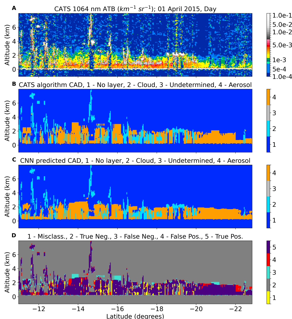
Figure 10. The same four plots and example as Figure 9. Images are focused on the PBL region.
