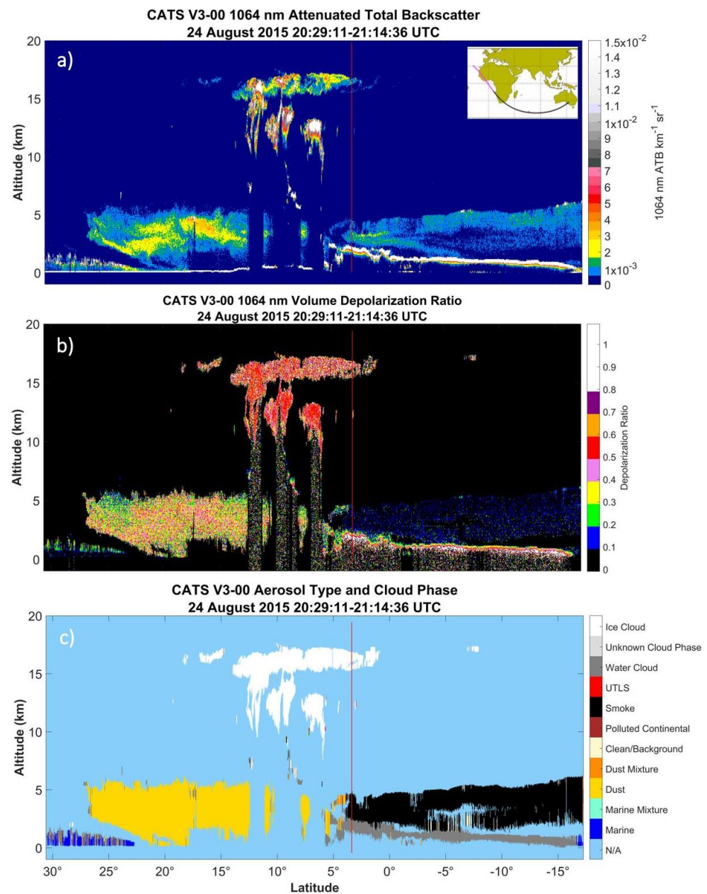
Figure 1. The CATS 1064 nm attenuated total backscatter (ATB) (a), volume depolarization ratio (b), and vertical feature type (c) on 24 August 2015 near the west coast of Africa. The red line shows the location of the vertical profile plotted in Figure 2.
