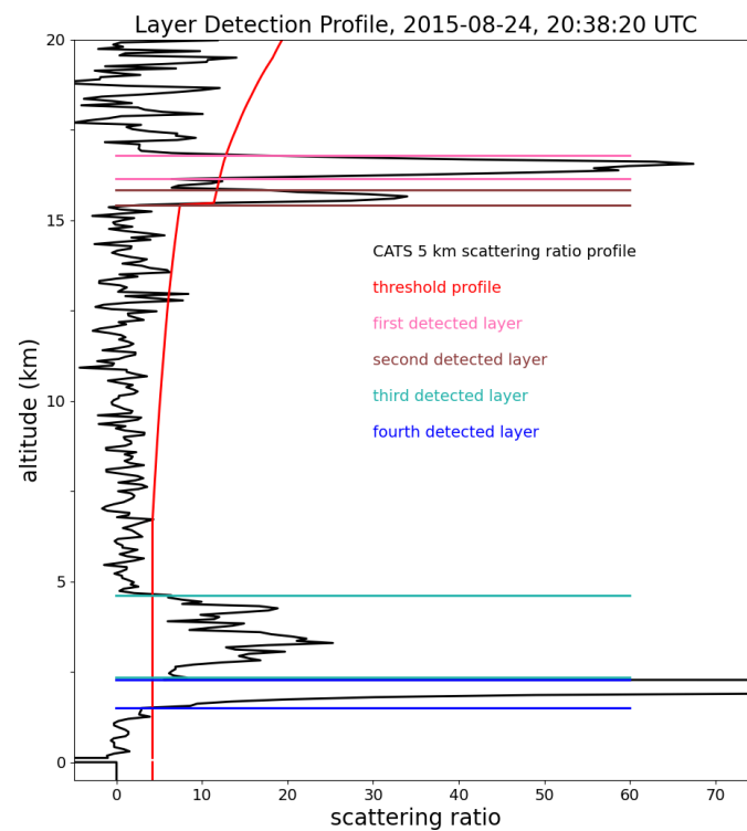
Figure 2. The CATS 1064 nm attenuated scattering ratio profile (black) from 24 August 2015 at 20:38:20 UTC (red line in Figure 1), averaged to 5 km horizontally. The CATS layer detection algorithm uses a threshold profile (red) to detect features, which in this case, identified four distinct layers (pink, brown, teal, and blue) with scattering ratio values greater than the threshold profile.
