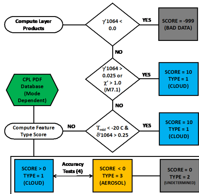
Figure 4. A flowchart of the CATS V3 L2O CAD algorithm.
