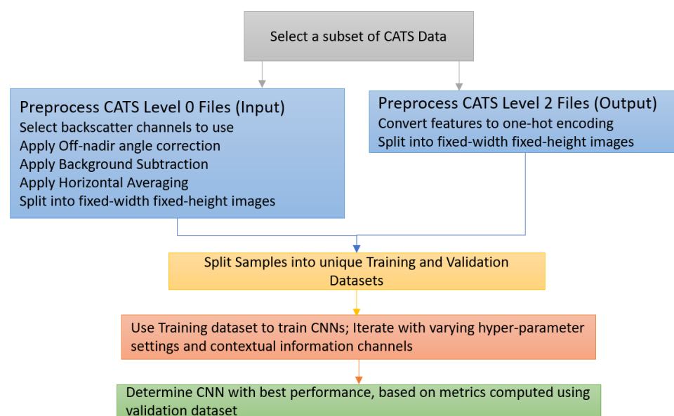
Figure 6. The flow of the CATS CNN model development starts with the subset of the CATS data chosen as the test data and ends with a selection of the CNN model with the best prediction metrics, as shown in this schematic.
