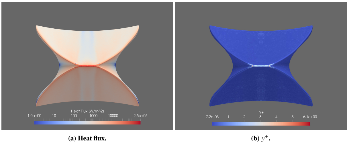
Fig. 13 The computed wall heat flux and y^+ values on the final BOLT grid.
