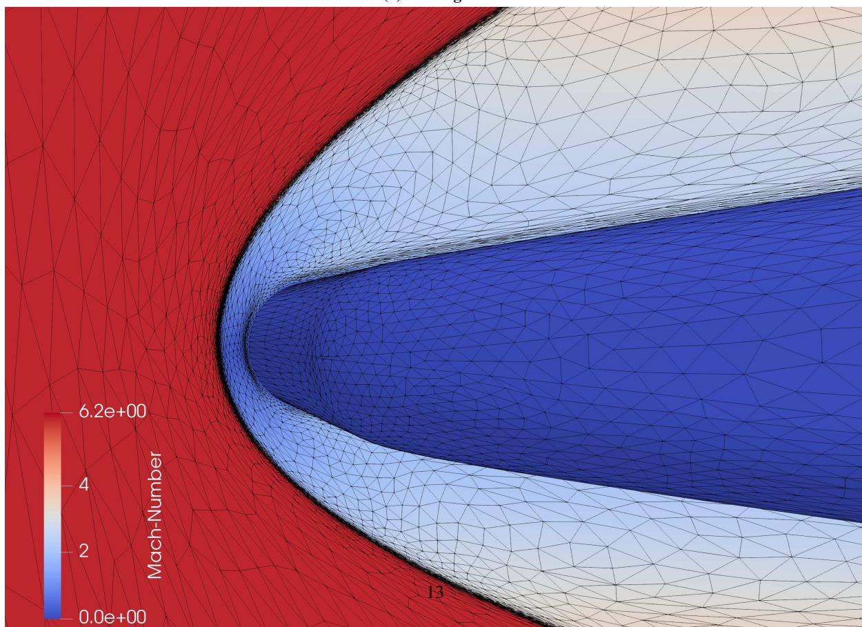
(b) Final grid.
