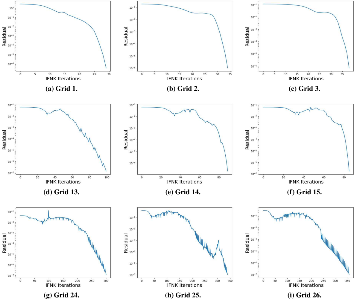
Fig. 3 Mach 6 flat plate convergence history for the first three, middle three, and final three grids in the adaptation sequence using the JFNK nonlinear solver.
