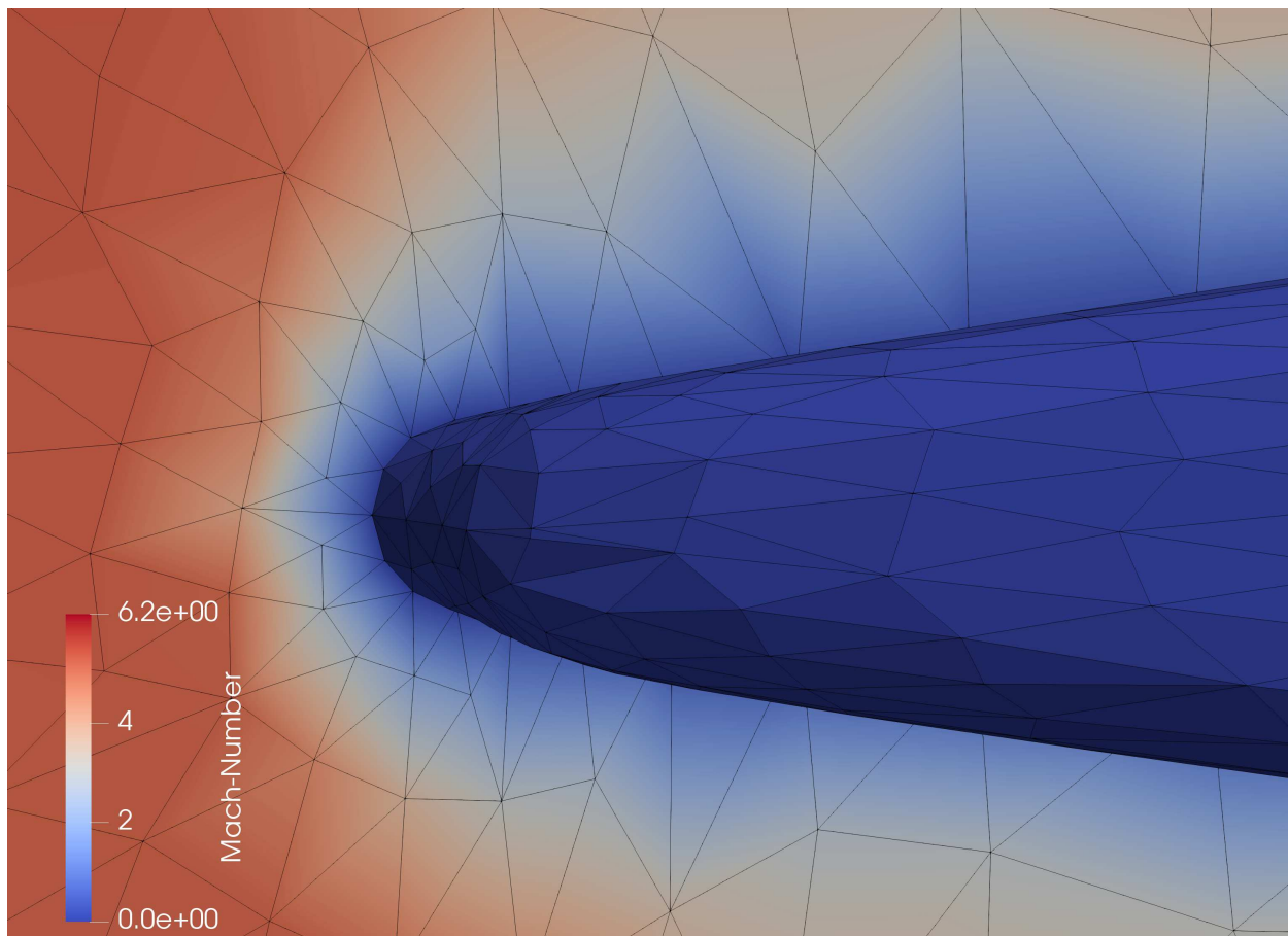
(a) Initial grid.
