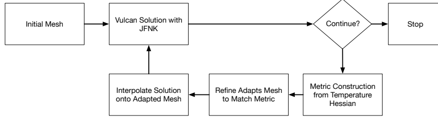
Fig. 1 Adaptation workflow: An initial mesh is iteratively adapted to control interpolation error in the temperature field.
