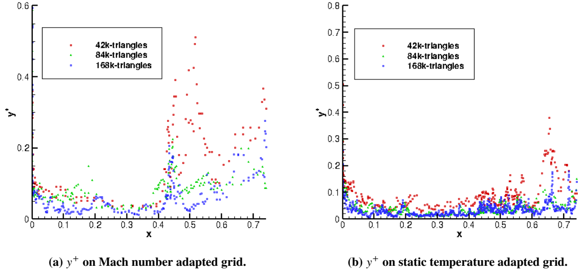
Fig. 8 Computed y^+ on coarse, medium, and fine grids for Mach number and static temperature trajectories.
