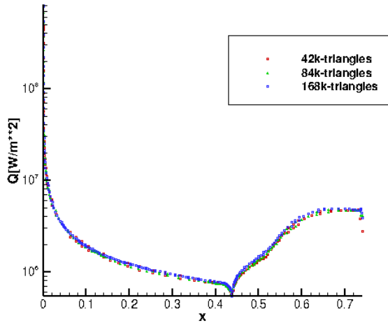
(a) Heat flux on Mach number adapted grid.
