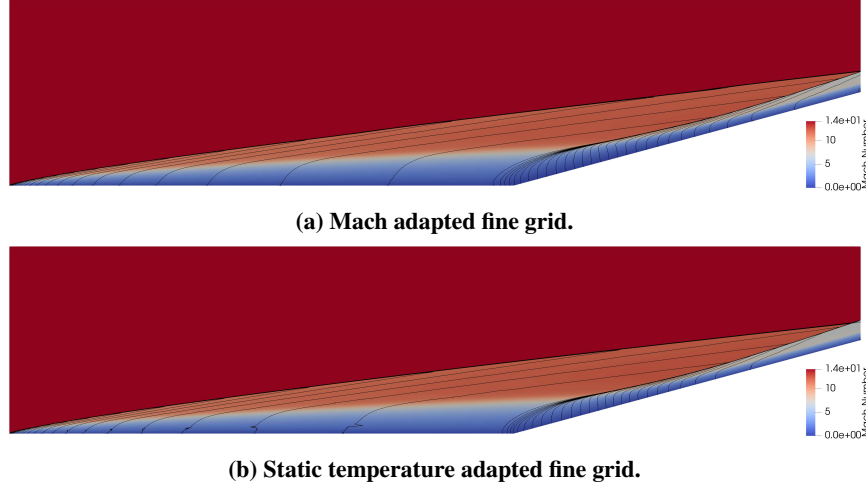
Fig. 5 Mach field with contour lines of static pressure on the fine grid from Mach number- and static temperature-based adaptation trajectories.
