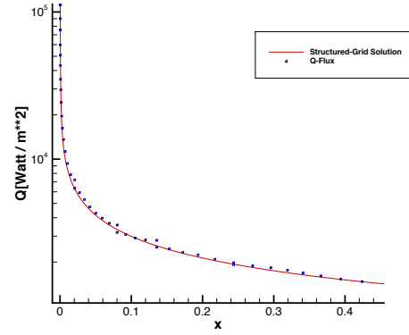
(b) Static temperature adapted Q .
