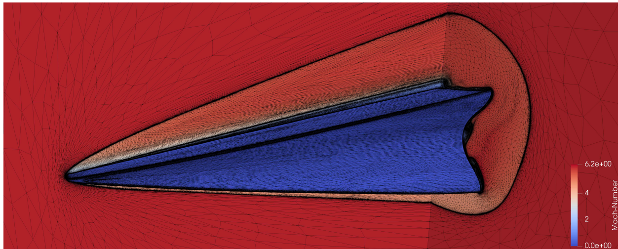
Fig. 10 Vehicle surface, symmetry plane, and outflow plane on the final adapted grid.
