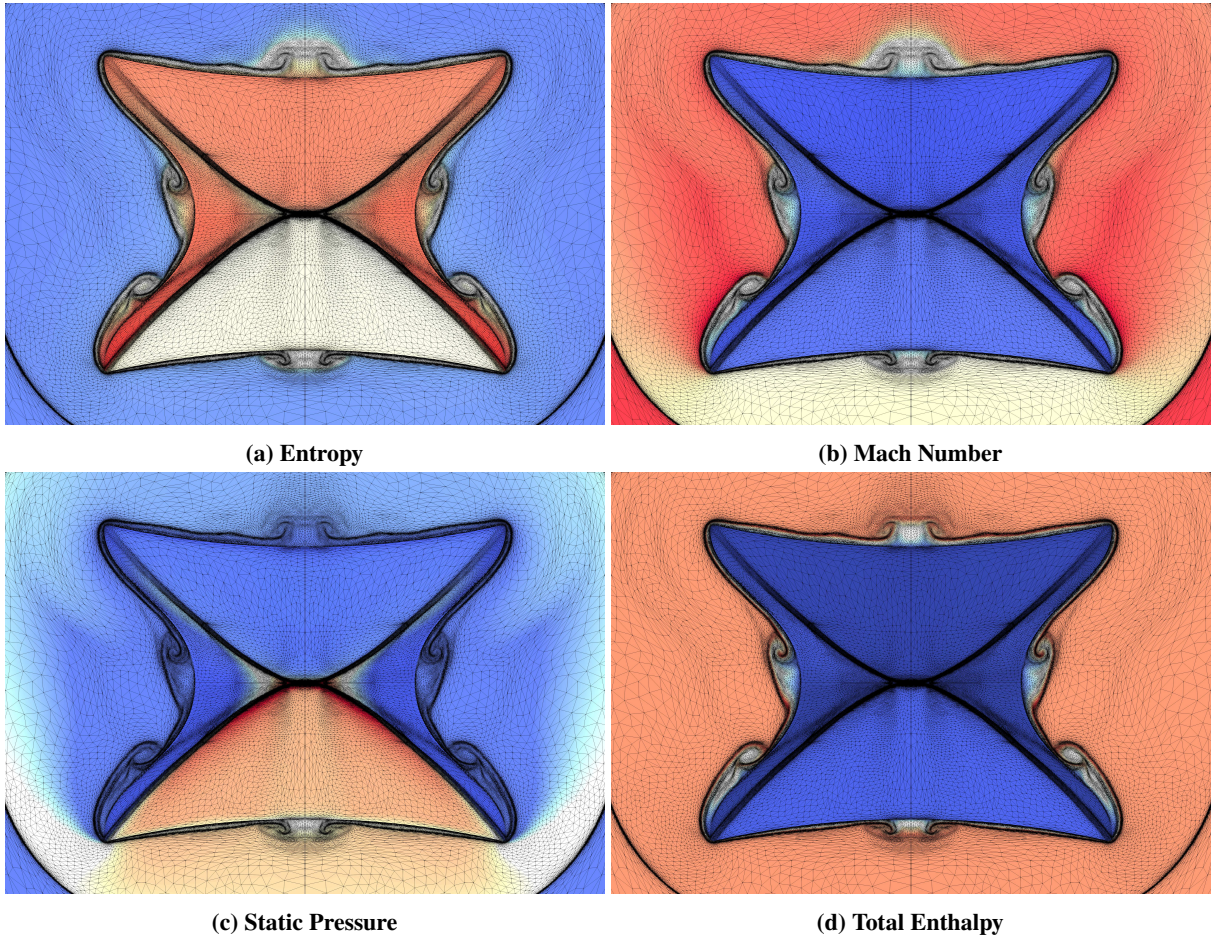
Fig. 12 Results for a laminar flow over the BOLT configuration at M_\infty = 6 and Re_\infty = 6.69 million on an adaptive tetrahedral grid.
