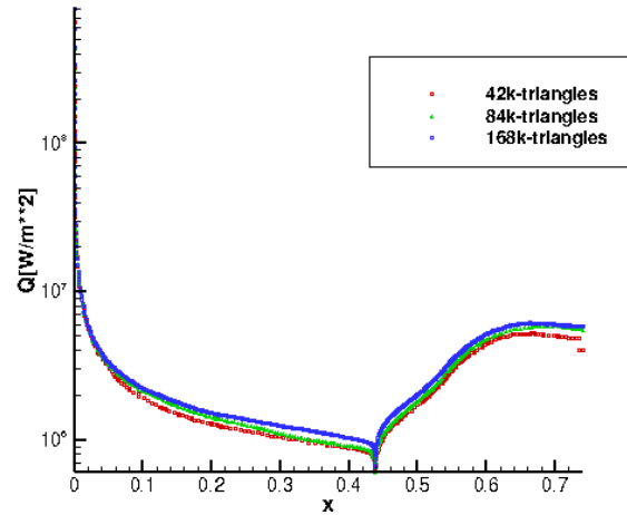
(b) heat flux on static temperature adapted grid.
