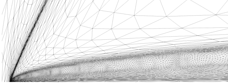
(b) Final adapted mesh with static temperature sensor.
