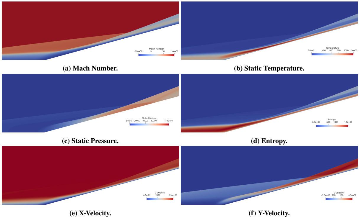
Fig. 9 Results for a laminar flow over a 15-degree compression corner at M_\infty = 14.1 and Re_\infty = 1.04 million on an adaptive triangular grid using the static temperature sensor.
