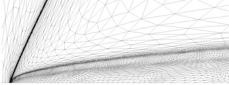
(a) Final adapted mesh with Mach sensor.
