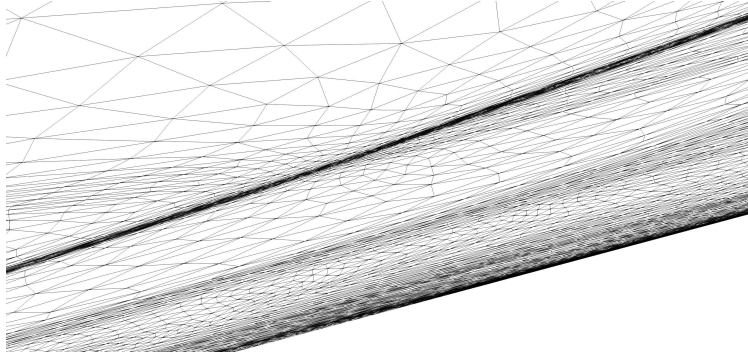
(b) 21k triangle grid with temperature-only error estimate.
