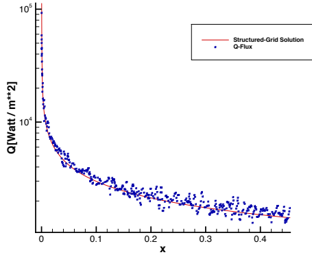
(a) Mach number adapted Q .
