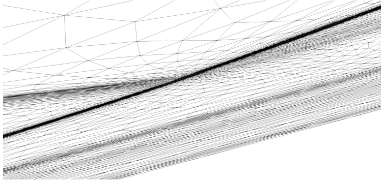
(a) 21k triangle grid with Mach-only error estimate.
