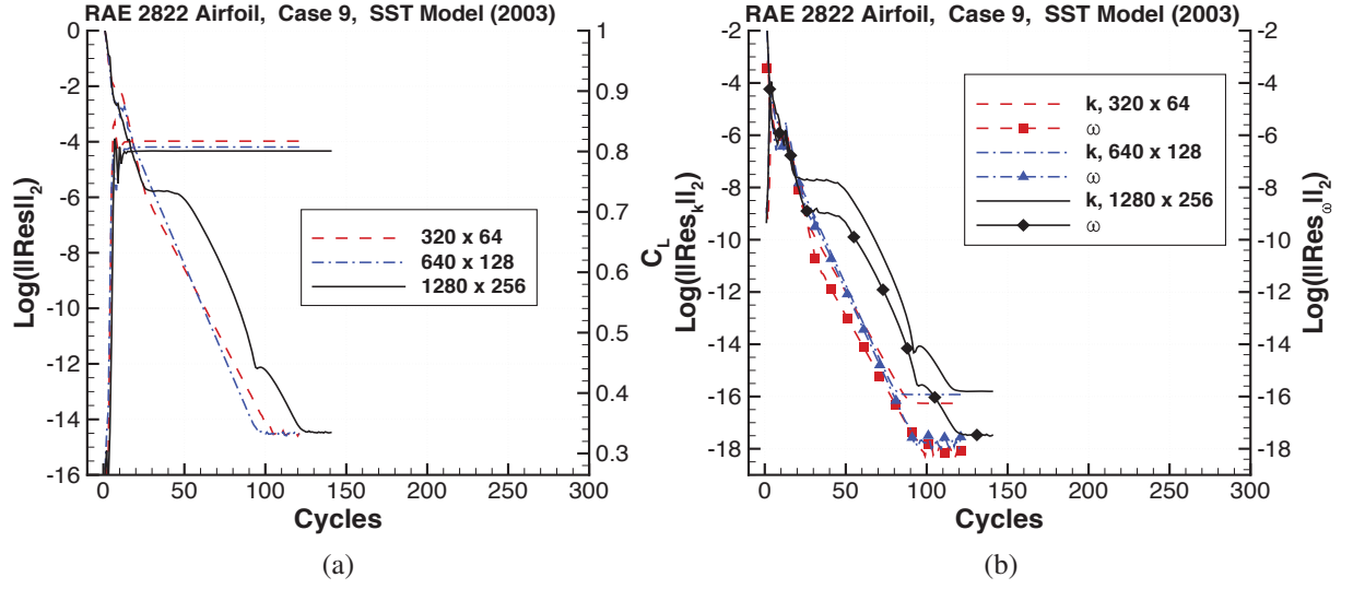
Figure 13: Convergence histories for Case 9 on three grids using the 2003 Menter SST model with strain rate in production term. (a) mean flow equations, (b) k-\omega equations.
