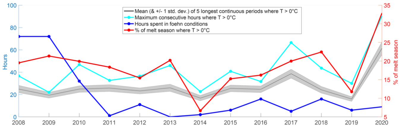
400 Figure 6. Analysis of sustained warm ( \geq 0^{\circ}\text{C} ) air temperature (T) periods and foehn wind occurrence for the 2007/2008 to 2019/2020 melt seasons. The cyan line shows the maximum number of consecutive hours in each melt season when T \geq 0^{\circ}\text{C} . The black line shows the mean length (hours) of the five longest periods when T \geq 0^{\circ}\text{C} for each season, with the grey shading indicating \pm 1 standard deviation from that mean. The red line shows the proportion of each season (1 November to 31 March) when T \geq 0^{\circ}\text{C} . The blue line shows the total number of hours spent in a foehn condition (see Section 3.4 for definition) each season. The x-axis dates indicate the second year of each austral summer, e.g., 2020 corresponds to the 2019/2020 season.
