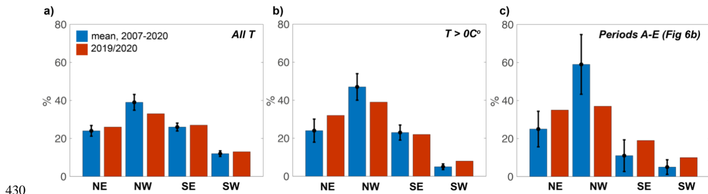
Figure 8. Percentage (%) of wind each season (1 November to 31 March) at Fossil Bluff AWS that is northeasterly (NE), northwesterly (NW), southeasterly (SE), southwesterly (SW), with the interannual (2007/2008 to 2019/2020) mean shown in blue and the 2019/2020 values shown in red. (a) Wind direction proportions using all recorded air temperatures. (b) Wind
