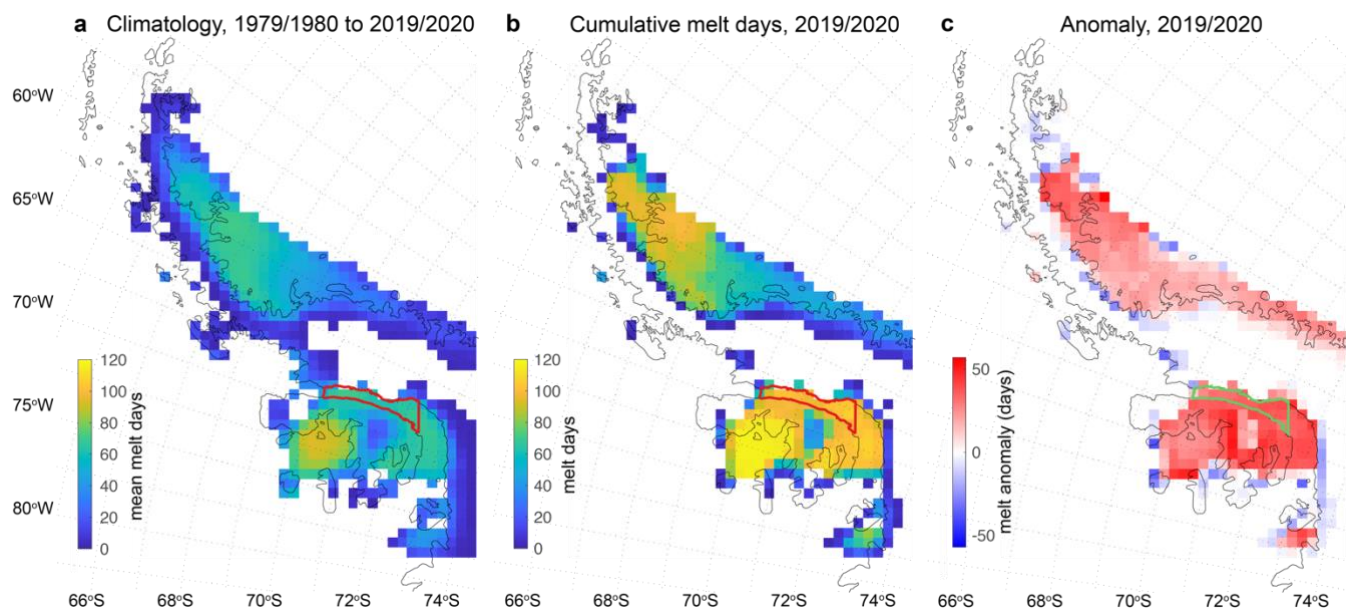
Figure 2. Microwave radiometer-derived maps of surface/near-surface melt days over the AP. (a) the climatology (i.e. mean cumulative melt days per season) from 1979/1980 to 2019/2020 (excluding 1987/1988 due to missing data); (b) cumulative melt days in 2019/2020; (c) the 2019/2020 melt season anomaly (i.e. (b) minus (a)). Melt days are counted within the period 1 November to 31 March (inclusive) each austral summer. The location of the study AOI is shown by a red outline in panels a) and b), and as a green outline in panel c). The black outline of the AP is from the MODIS Mosaic of Antarctica (Haran et al., 2014).
