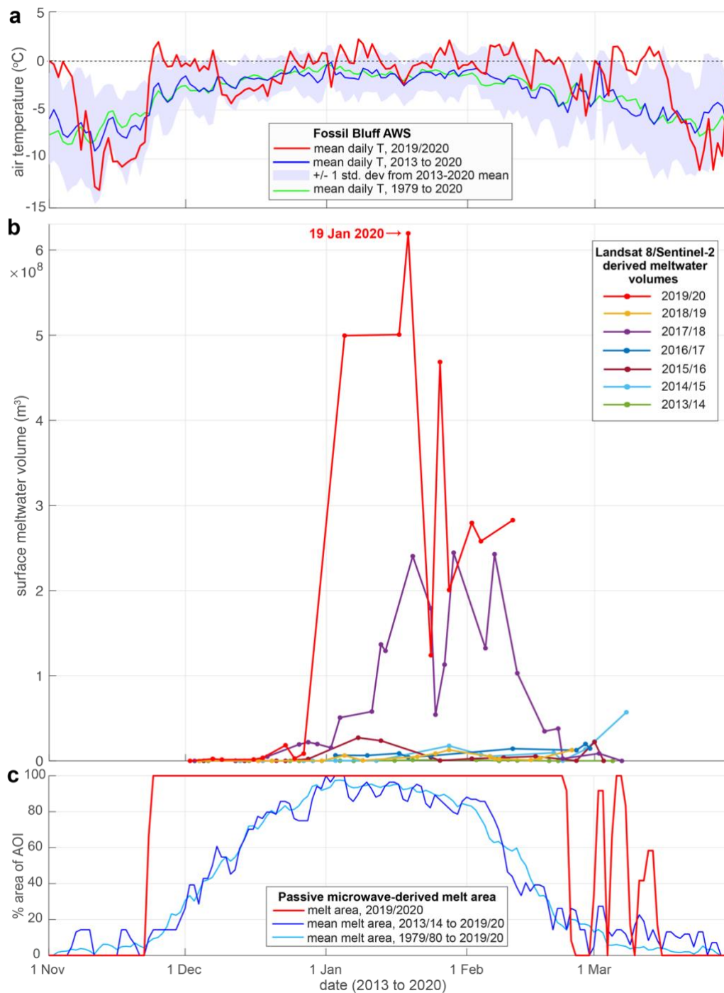
Figure 5 (a) Surface (2 m) air temperature data from the Fossil Bluff AWS (location in Fig. 1b, yellow star). The daily mean air temperature for the 2019/2020 melt season are shown by the red line, the daily mean for the 7 melt seasons from 2013/2014 to 2019/2020 are shown by the blue line, +/- one standard deviation from that blue line is shown by the areas of blue shading,
