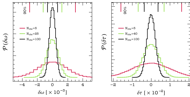
Figure 15. Posterior probability distributions for GR deviations within the QNM spectrum of rotating BHs observed by LGWA, as a function of the number of observed events. We assume that only the fundamental \ell = m = 2 mode is detected, and that the S/N of each event is fixed to 100. Vertical bars identify 90% confidence intervals. Time is measured in units of GM/c^3 .
