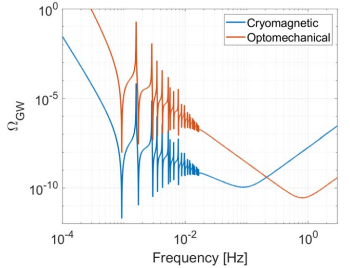
Figure 4. Predicted LGWA sensitivity to stochastic GW backgrounds.
