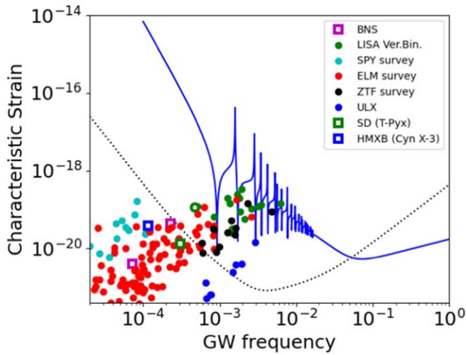
Figure 8. Strength of the GW emission from known short-period binary systems in the Galaxy compared with the expected sensitivity of LGWA (blue line, cryogenic) and LISA (black dotted line).
