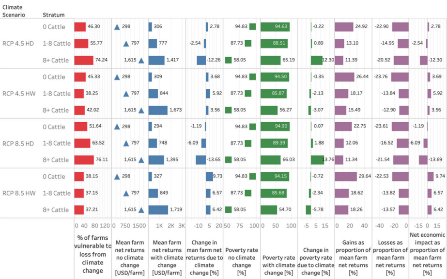
Fig. 4 Sensitivity to climate change (CC), for climate scenarios (hot/dry, hot/wet), emission scenario (RCP 4.5, RCP 8.5) and farm types in Nkayi, Zimbabwe, using APSIM results as input
