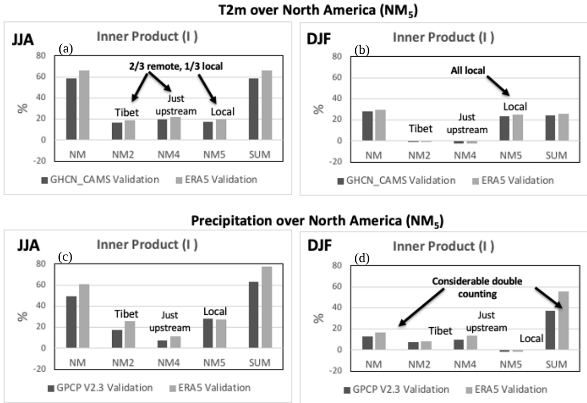
Figure 9: T2m bias correction in NM 5 from TBC in various NM Subregions. The contributions from the NM region and from the NM 2 , NM 4 , and NM 5 subregions, as well as the sum of the corrections from all 6 NM subregions, are shown. The biases are computed with respect to station observations (dark bars) or ERA-5 (light bars). The values are the normalized inner products as defined in eq. 3 of the text. See Figure 2 for the definitions of the regions.
