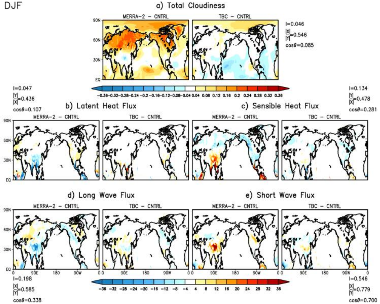
Figure 13: Impacts for DJF of global TBC on a) total cloudiness (fraction of area), b) latent heat flux, c) sensible heat flux, d) longwave flux at the surface and, e) shortwave flux at the surface. In each set of two panels the left panel is the negative of the bias (MERRA-2 minus CNTRL), and the right panel is TBC minus CNTRL. Values are averaged over the period 1980-2017. Units are: W/m^2 .
