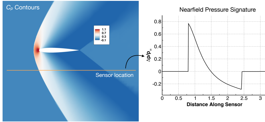
Figure 3: Near-body flow (left) and pressure signature (right) for the NACA 0012 airfoil at M_\infty = 1.4
