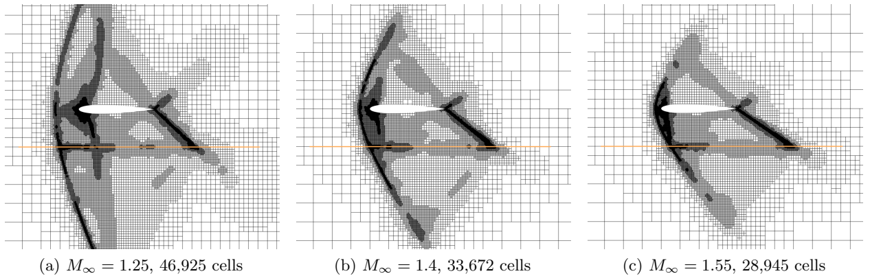
Figure 7: Near-body meshes for the mean and 3\sigma realizations of M_\infty with the location of the sensor indicated
