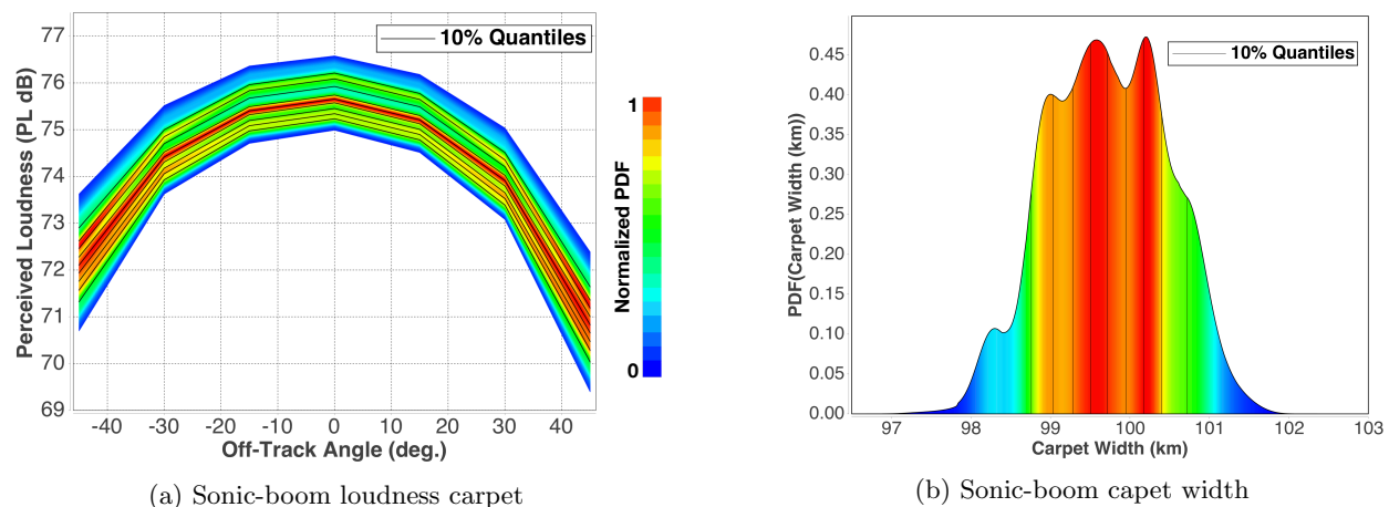
Figure 20: Probability density functions for loudness carpet and carpet width due to uncertainty in M_\infty .
