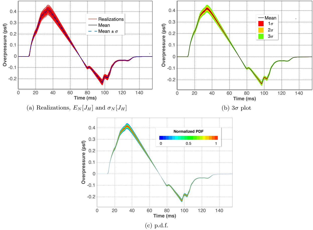
Figure 17: Uncertainty quantification for on-track ground signature
