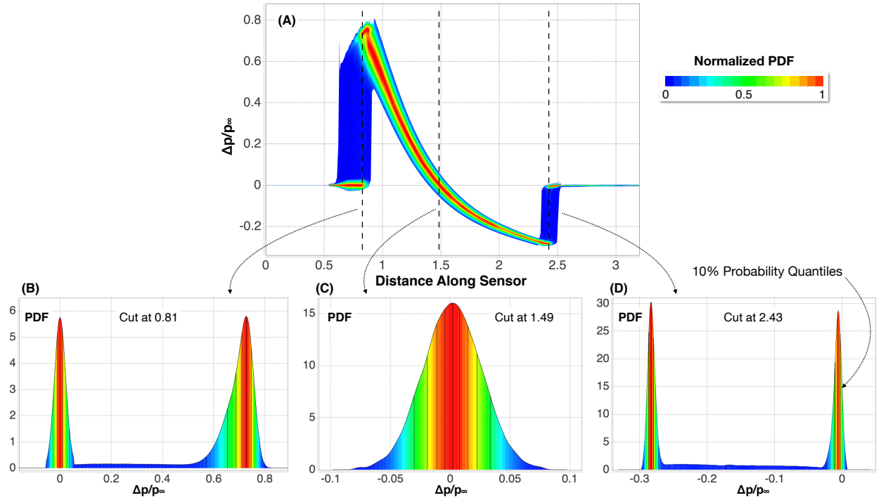
Figure 5: (A) Probability density function p for the nearfield signature due to uncertain Mach number. (B) p cut in the front-shock region showing a bimodal distribution. (C) p cut near the zero-crossing of the expansion showing a normal distribution. (D) p cut in the aft-shock region showing a bimodal distribution. Vertical lines in frames B, C and D mark 10% quantiles.
