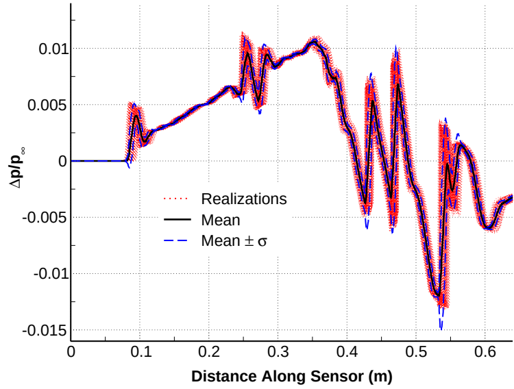
(c) Pressure signatures and moment statistics
