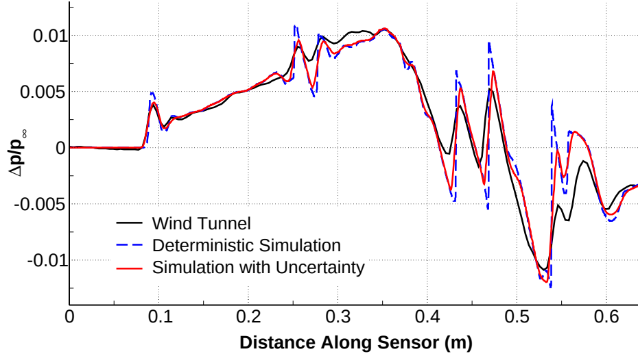
Figure 13: Assessment of experimental discrepancy: pressure signatures obtained from the LM 1044 test (Wind Tunnel), simulation with no statistical uncertainty (Deterministic Simulation) and the mean signature obtained via uncertainty analysis (Simulation with Uncertainty)
