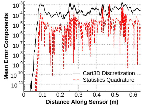
(b) Numerical error balance: realization E[\varepsilon_H] and quadrature \varepsilon_Q[J_H] errors
