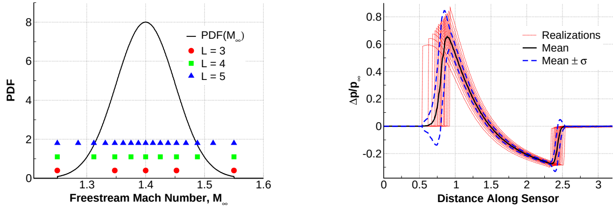
(a) Input uncertainty M_\infty = \text{Gaussian}_{3\sigma}(\text{mean} = 1.4, \sigma = 0.05) and nodes for quadrature levels L
