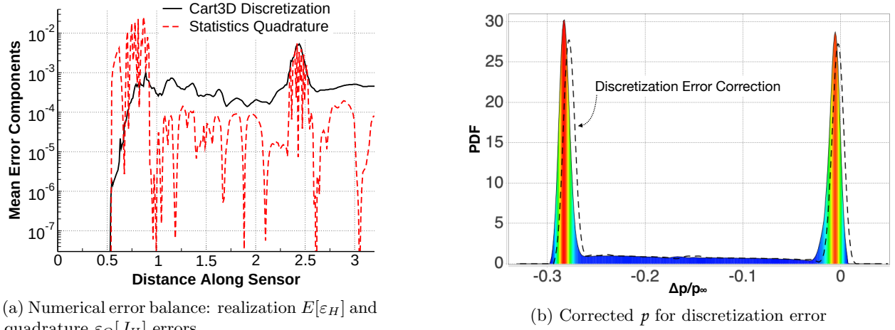
Figure 8: Numerical error balance for the mean (left) and p.d.f of aft-shock region with discretization error correction (right)
