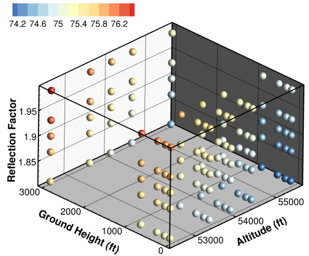
Figure 18: All realizations (125) colored by level of perceived loudness (PLdB)
