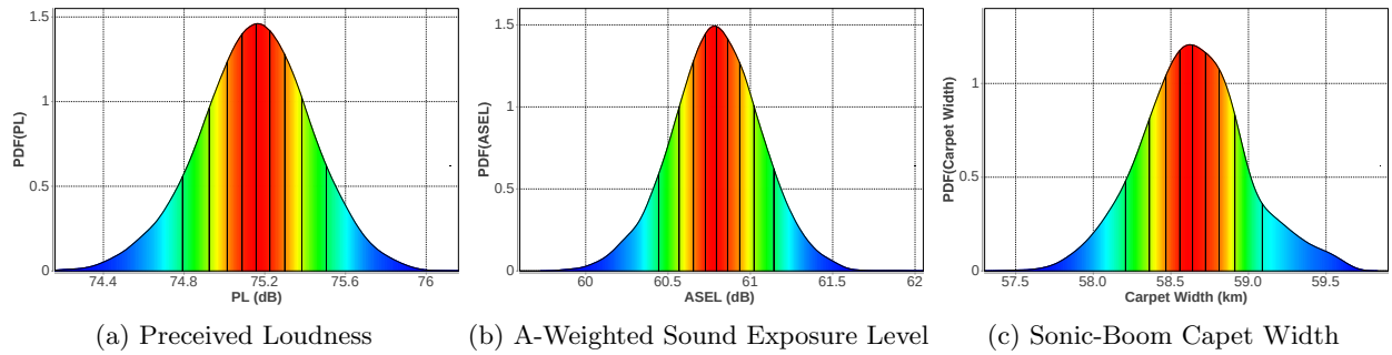
Figure 19: Probability density functions for noise metrics and boom carpet width. Black vertical lines mark 10% quantiles and colors represent normalized probability: red=1 (very likely) and blue=0.01 (unlikely).
