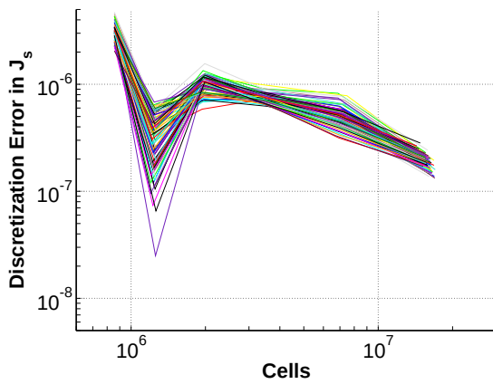
(a) \varepsilon_H adaptation history, 81 realizations
