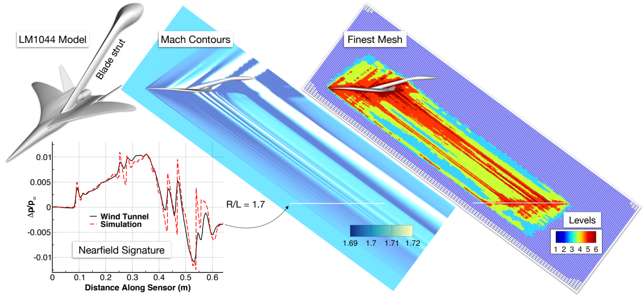
Figure 9: LM 1044 model (upper left), Mach contours on plane of symmetry with pressure sensor indicated (center), final mesh after six adaptations (right), and extracted pressure signature with comparison to measured data (lower left), M_\infty = 1.7 and \alpha = 2.17^\circ
