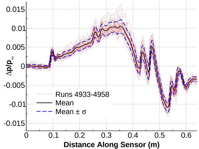
Figure 10: Pressure signatures from each of the 26 model positions for the LM 1044 tests, and the resulting mean signature and standard deviation.
