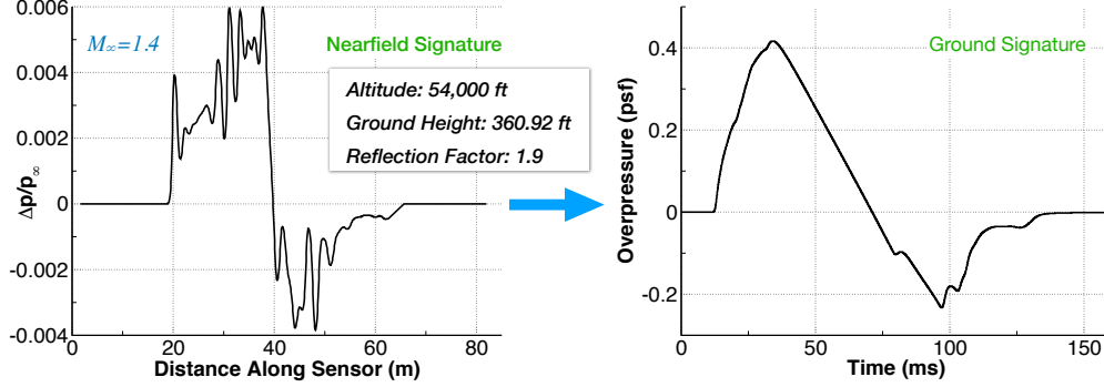
Figure 15: Case 2 from SBPW3: Nearfield signature (left), and Ground signature (right)
