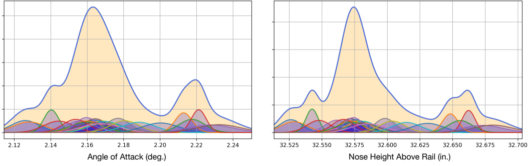
Figure 11: Estimated probability density functions for \alpha (left) and h_{\text{nose}} (right) from the LM 1044 tests.
