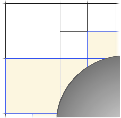
Figure 2: Multilevel Cartesian mesh in two-dimensions with a cut-cell boundary. Adjacent cells cannot exceed 2:1 ratio.
