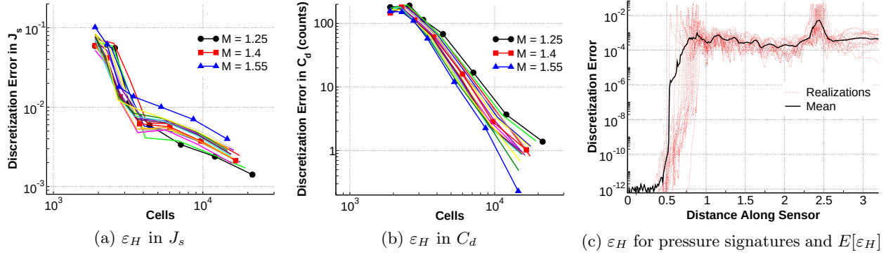
Figure 6: Estimate of discretization error \varepsilon_H , Eq. 11, for all 17 realizations. Mean and 3\sigma simulations are indicated with symbols in (a) and (b) that also mark adaptation cycles.
