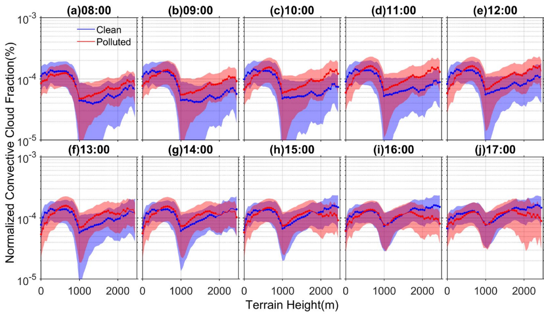
Figure 10. Same as Figure 9, but for CCF_{C(P)} that is normalized by the number of cases under polluted and clean conditions during each hour, i.e. NCCF_{C(P)} , respectively (Equation 4).
