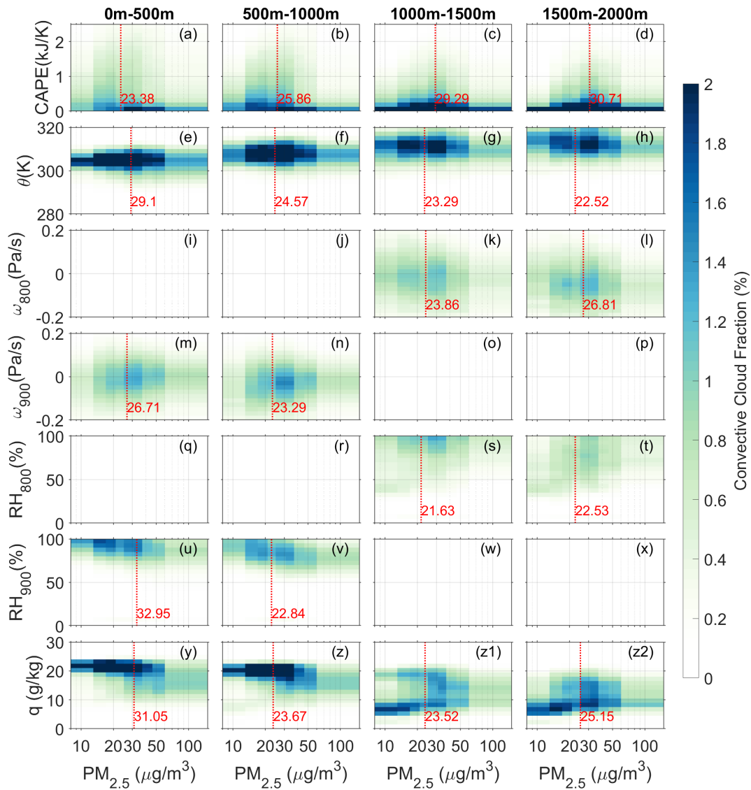
915 Figure 14. Same as Figure 13, but for different terrain heights; each column represents a different terrain height range.
