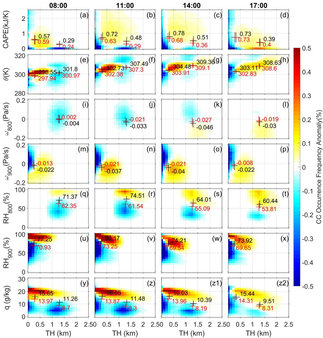
855 Figure 5. Over-land convective cloud occurrence frequency(CC OF) anomaly with respect to terrain height (TH) and (a-d) convective available potential energy (CAPE), (e-h) potential temperature ( \theta ), (i-l) vertical pressure velocity at 800 hPa ( \omega_{800} ) over terrain above 1000 m, (m-p) vertical pressure velocity at 900 hPa ( \omega_{900} ) over terrain below 1000 m, (q-t) relative humidity at 800 hPa ( RH_{800} ) over terrain above 1000 m, (u-x) relative humidity at 900 hPa ( RH_{900} ) over terrain below 1000 m, (y-z2) specific humidity at 2m (q). The columns represent local time over the ROI of 08:00, 11:00, 14:00 and 17:00, respectively. Black (red) crosses and numbers beside mark the mean values of the variables with convective cloud (under all-sky conditions) over regions with terrain
