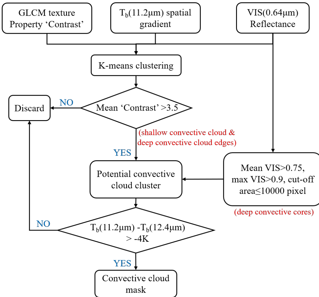
Figure 2. Flowchart of the convective cloud identification method.
