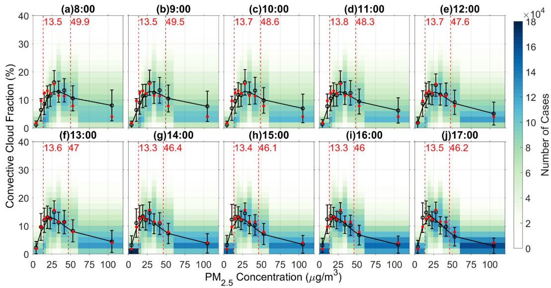
Figure 8. Convective cloud fraction with respect to PM 2.5 concentration at different times of day during May-September, 2016-2017. Color shading indicates the number of cases corresponding to each specific convective cloud fraction (CCF) and PM 2.5 bin. Note that PM 2.5 is separated into ten equal-sample bins. Black circles and error bars are the mean values and standard deviations of CCF in each PM 2.5 bin within each hour, red dots indicate the mean CCF over all times. Black solid lines represent the three-point moving average of the black circles. Red dashed lines (with red numbers) mark the mean polluted and clean thresholds during each hour.
