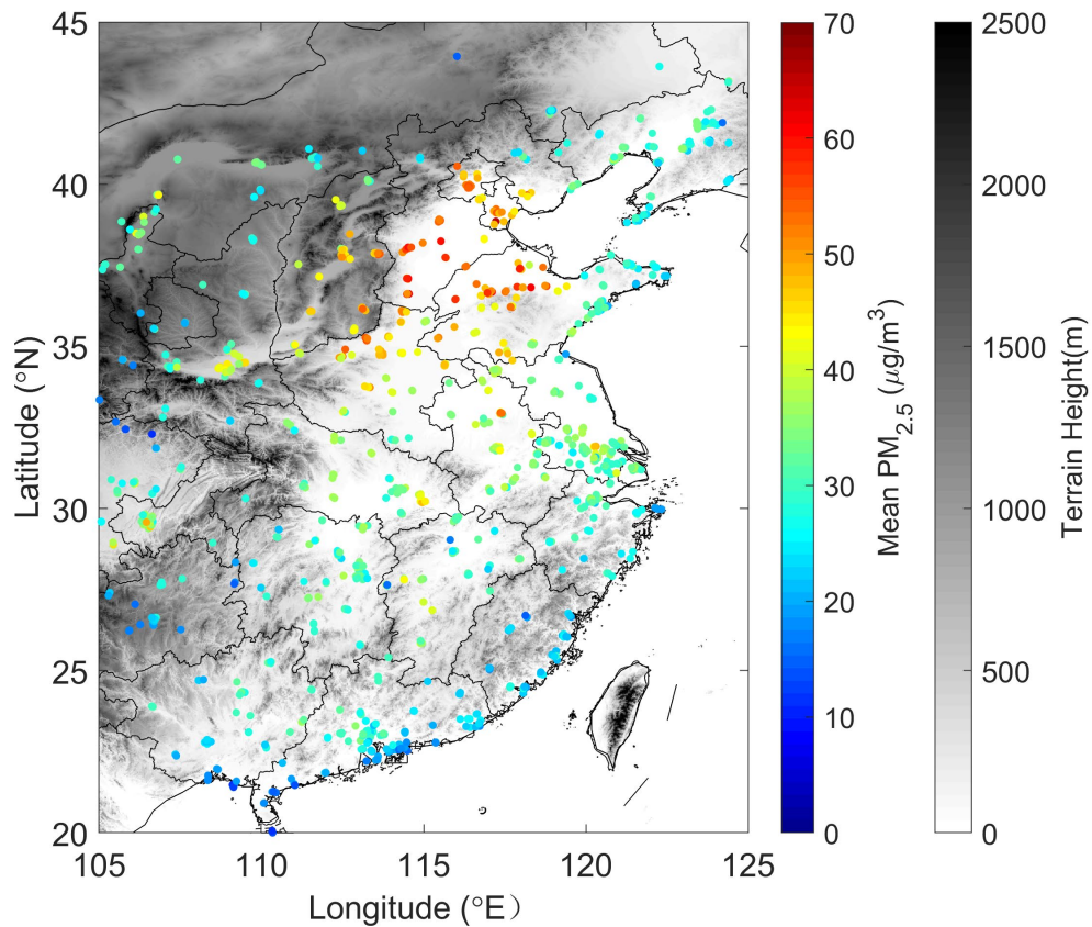
840 Figure 1. Surface elevation and the mean value of ground-based PM 2.5 measurements over eastern China. The terrain height (TH) of this region is represented with gray shading. Colored dots show the mean PM 2.5 concentration from 1205 surface stations during May-September in 2016-2017 over this area.
