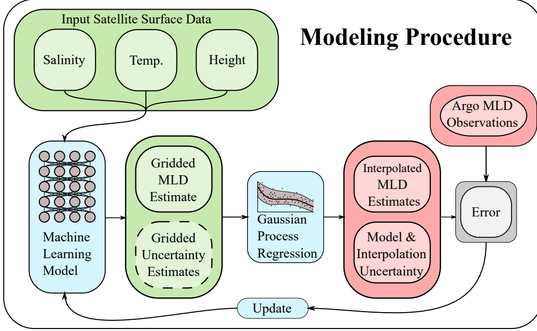
Figure 3. A schematic of the Argo dataset experiment modeling procedure. Satellite sea surface data is fed into the machine learning model to produce a gridded MLD estimate (with some form of an uncertainty estimate if the machine learning model is probabilistic). To compare with the observations and optimize parameters, these gridded estimates are fed into a Gaussian process regression model (with its own hyper-parameters that are optimized) to produce MLD estimates interpolated to the locations where the Argo observations exist. These interpolated estimates are automatically associated with uncertainty estimates that are derived from either just the Gaussian process interpolation uncertainty (if the model is deterministic) or a combination of the Gaussian process uncertainty with ML model uncertainty (if the ML model has uncertainty estimates). The interpolated estimates are then compared with the observations to estimate various errors. The CESM POP2 ocean model dataset experiments have the same modeling design but do not require interpolation, since ocean model MLD is on the same grid as the inputs.
