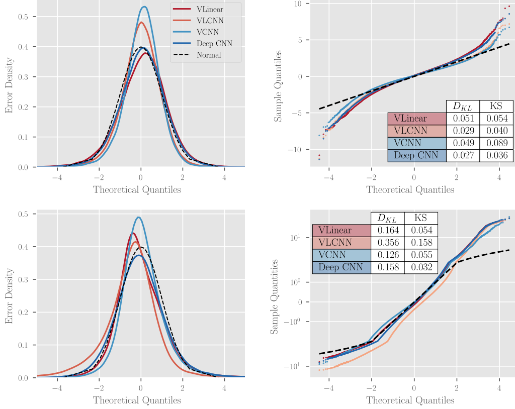
Figure 8. A study of the distribution of normalized errors for 4 of the top performing probabilistic methodologies and architectures from Fig. 7 assessed by grid-point. Each model assumes that the difference between model predictions and reality, normalized by the model standard deviation, should be approximately normal with mean zero and unit variance. For (top) EPO and (bottom) SIO, we present (left) a visual comparison of the error distribution probabilistic density functions and (right) a quantile-quantile comparison of the given error distribution and a standard normal distribution (dotted black line, optimal) with a table showing the KL Divergences and relative L_2 norm between sample and theoretical distributions (see text for definitions). Notice the semi-log scale on the bottom-right plot. For an interpretation of the right plots, see the accompanying discussion in the text.
