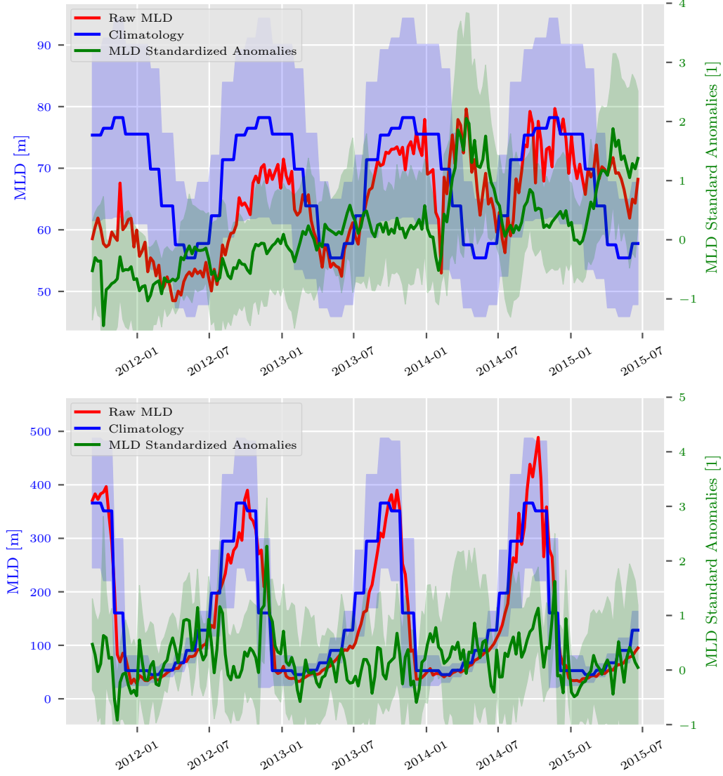
Figure 2. Several time series of the average MLD in each region at weekly resolution in the (top) equatorial Pacific and (bottom) southern Indian Ocean, including the ensemble average of the MLD profiles over the domain (red), the ensemble average of the corresponding standardized MLD anomalies (green), and the area-average of the gridded monthly MLD climatology (blue). The blue shading represents the area-average of the gridded monthly standard deviations, and the green shading represents the ensemble standard deviation of the profile-wise standard anomalies.
