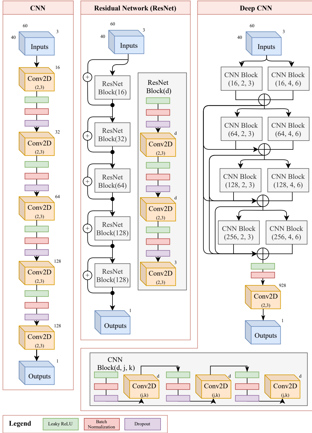
Figure B1. Architecture map of the three leading types of machine learning models used in this manuscript: ‘CNN’, ‘ResNet’, and ‘Deep CNN’. See the text for details.
