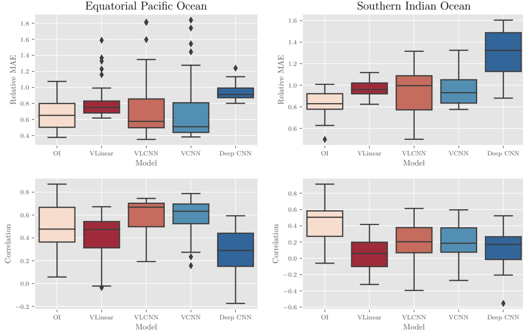
Figure 10. Deterministic results of various machine learning methodologies and OI as applied to the Argo profile data experiment. Boxes capture 25-75% of the weekly errors with the middle line representing the median error. Dots are considered outliers - values which are 1.5\times lower/upper quantile. In the top row, a comparison of the relative mean absolute errors (MAEs) for each method in the (left) equatorial Pacific Ocean (EPO) and (right) southern Indian Ocean (SIO). In the bottom row, a comparison of the correlation coefficients between predictions and truth in the (left) EPO and (right) SIO. Each metric is unit-less and a lower MAE and higher correlation are equated with better performance. For each pair of graphs, notice the different scales for the EPO and SIO results as performance is generally better in the EPO compared to the SIO.
