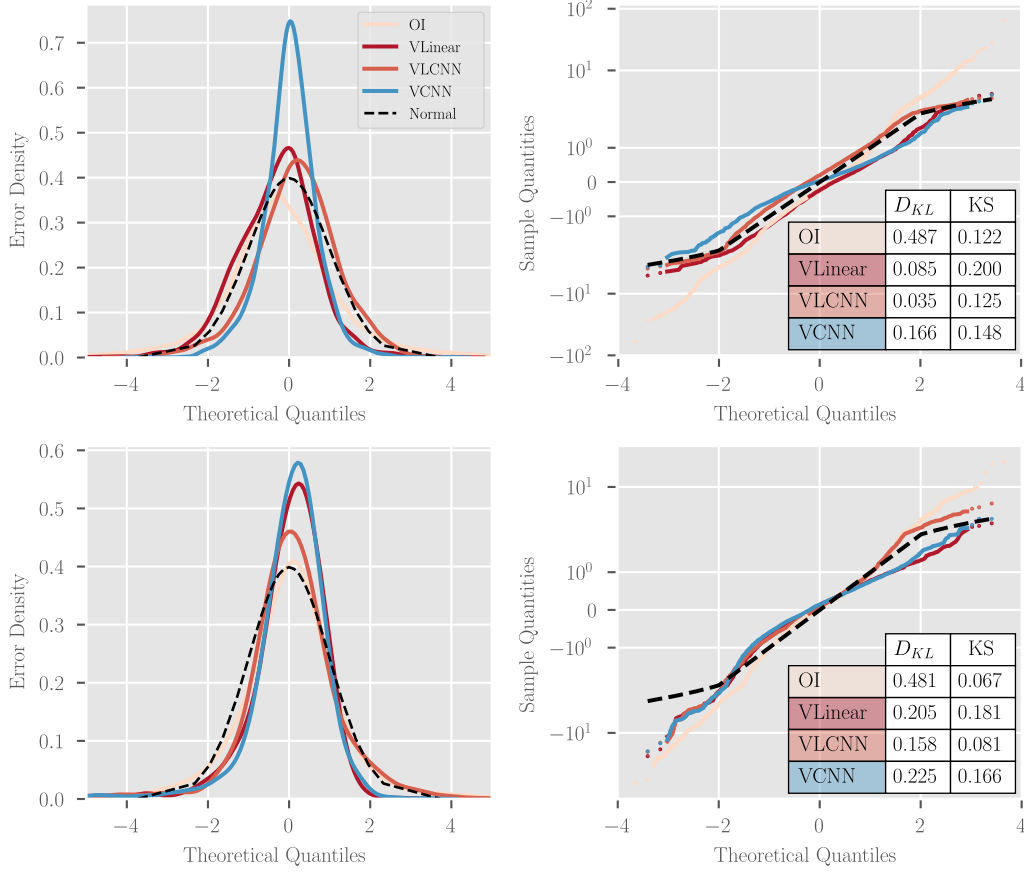
Figure 11. Probabilistic calibration for temporal out-of-sample prediction as in Fig. 10. Statistics are calculated on each datapoint for the 50 withheld validation weeks. For (top) EPO and (bottom) SIO, we present (left) a visual comparison of the error distribution probabilistic density functions and (right) a quantile-quantile comparison of the given error distribution and a standard normal distribution (dotted black line, optimal) with a table showing the KL Divergences and relative L_2 norm between sample and theoretical distributions (see text for definitions). Notice the semi-log scale on the right plots.
