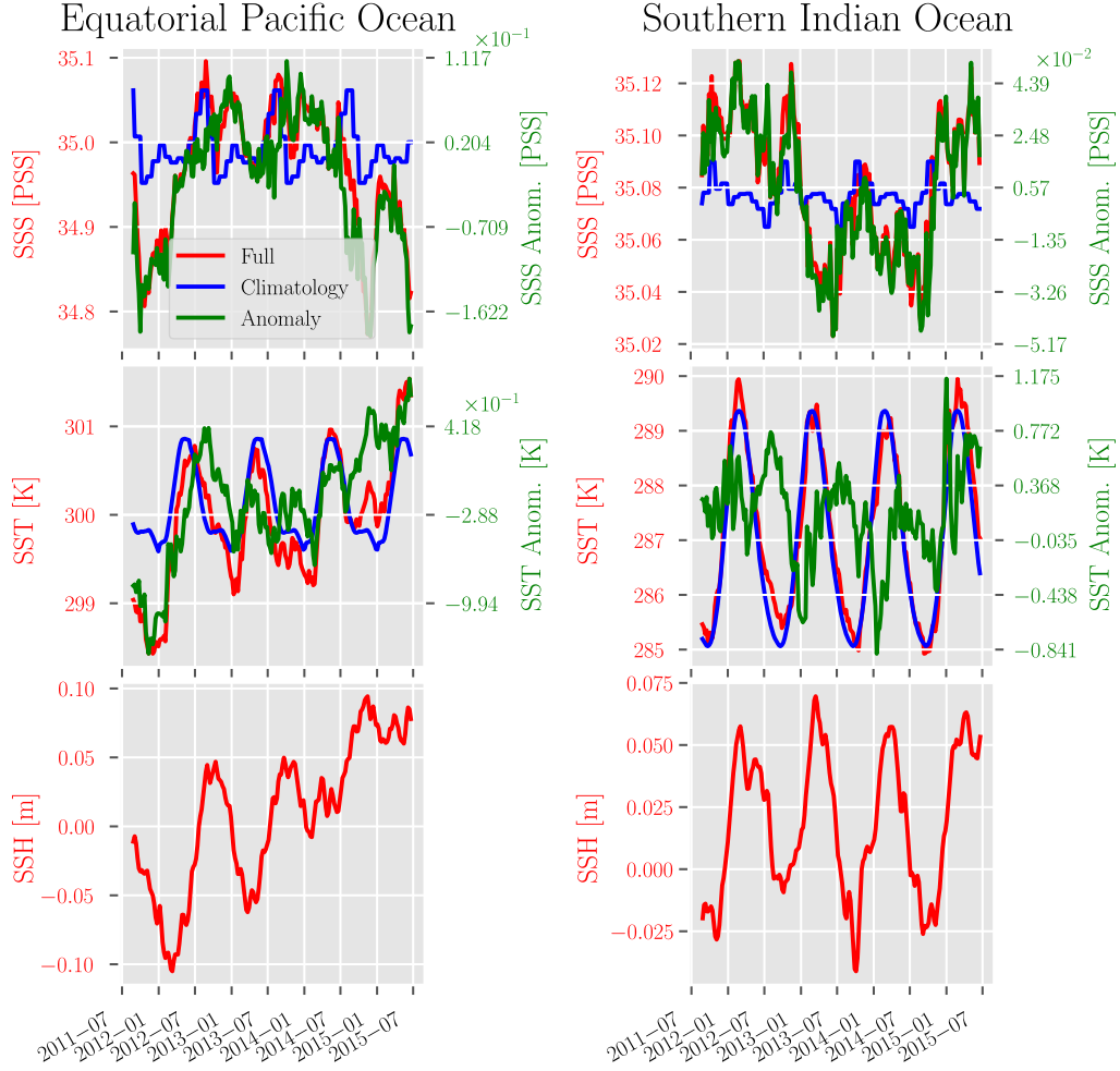
Figure 1. Several time series of the spatially averaged SSS, SST, and SSH in each region at weekly resolution in the (left) equatorial Pacific (120W, 10S) - (150W, 10N) and (right) southern Indian Ocean (45S, 55E) - (35S, 115E) regions. The time series include the spatially averaged (red) satellite data, (blue) estimated climatology, and (green) resulting anomaly.
