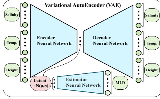
Figure A1. A schematic of the modified VAE. On the left hand side, the SSS, SST, and SSH inputs are fed into a neural network, called the Encoder network, that produces an output of smaller dimension - the latent space. On the right hand side, a second neural network, called the Decoder network, takes the latent variables as inputs and attempts to reproduce the original SSS, SST, and SSH inputs. In our implementation of the VAE, there is a third neural network that takes the latent space as inputs and outputs an estimate of the MLD. Training is informed by the decoder and estimator networks losses. For a full description of the training procedure for a typical VAE, see Kingma and Welling (2014).
