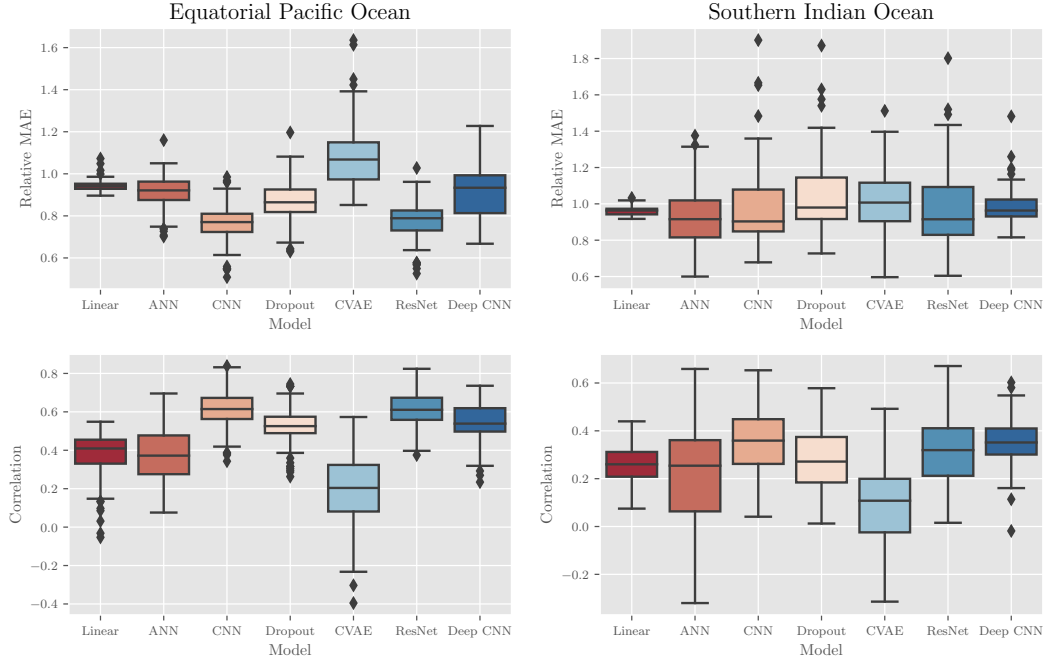
Figure 4. Deterministic results of various machine learning methodologies as applied to the CESM POP2 Ocean Model data experiment. Boxes capture 25-75% of the weekly errors with the middle line representing the median error. Dots are considered outliers - values which are 1.5 \times lower/upper quantile. In the top row, a comparison of the relative mean absolute errors (MAEs) for each method in the (left) equatorial Pacific Ocean (EPO) and (right) southern Indian Ocean (SIO). In the bottom row, a comparison of the correlation coefficients between predictions and truth in the (left) EPO and (right) SIO. Each metric is unit-less and a lower MAE and higher correlation are equated with better performance. For each pair of graphs, notice the different scales for the EPO and SIO results as performance is generally better in the EPO compared to the SIO.
