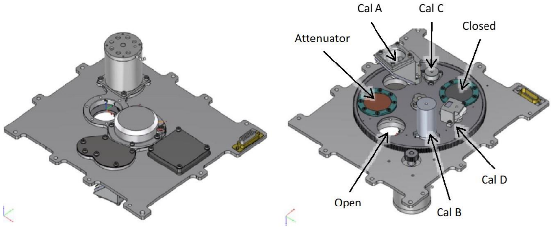
Figure 7: Filter and calibration wheel assembly (left: top view (+z); right: bottom view (-z))
