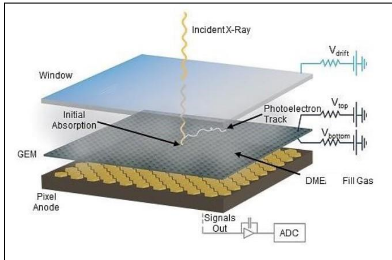
Figure 3: Schematic of the Gas Pixel Detector (GPD)
