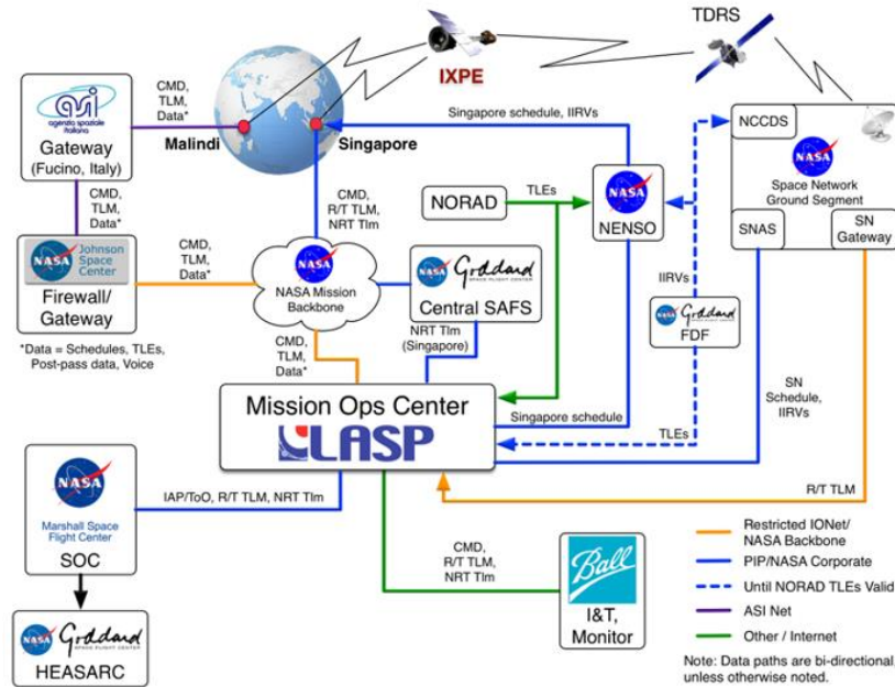
Figure 9: IXPE ground network
