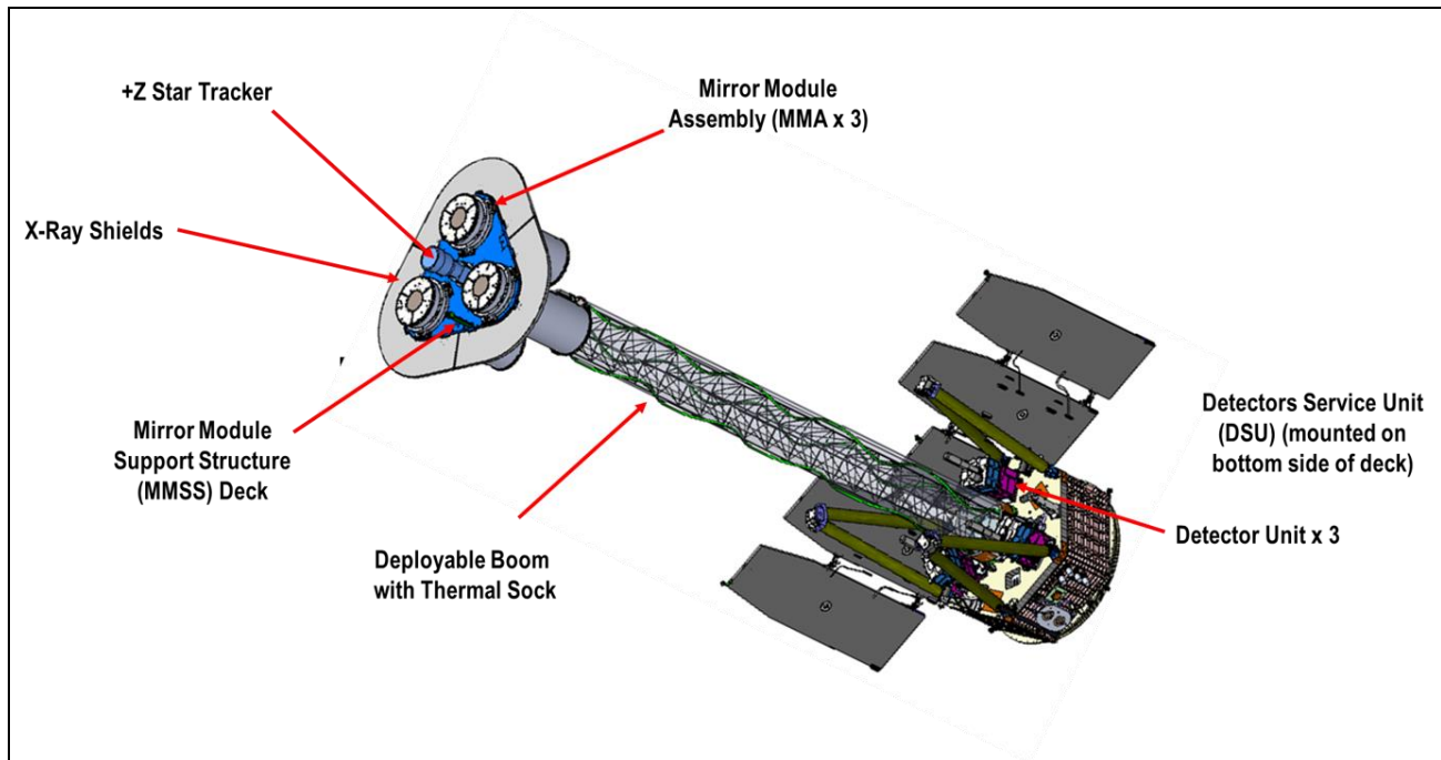
Figure 1: The IXPE Observatory payload elements
