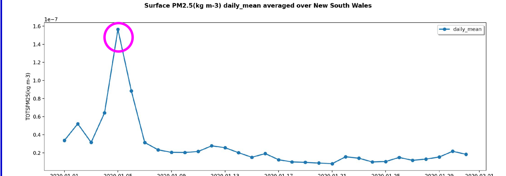
Figure 8. The evolution of daily mean of the MERRA-2 PM 2.5 over New South Wales in Australia in Jan. 2020.
