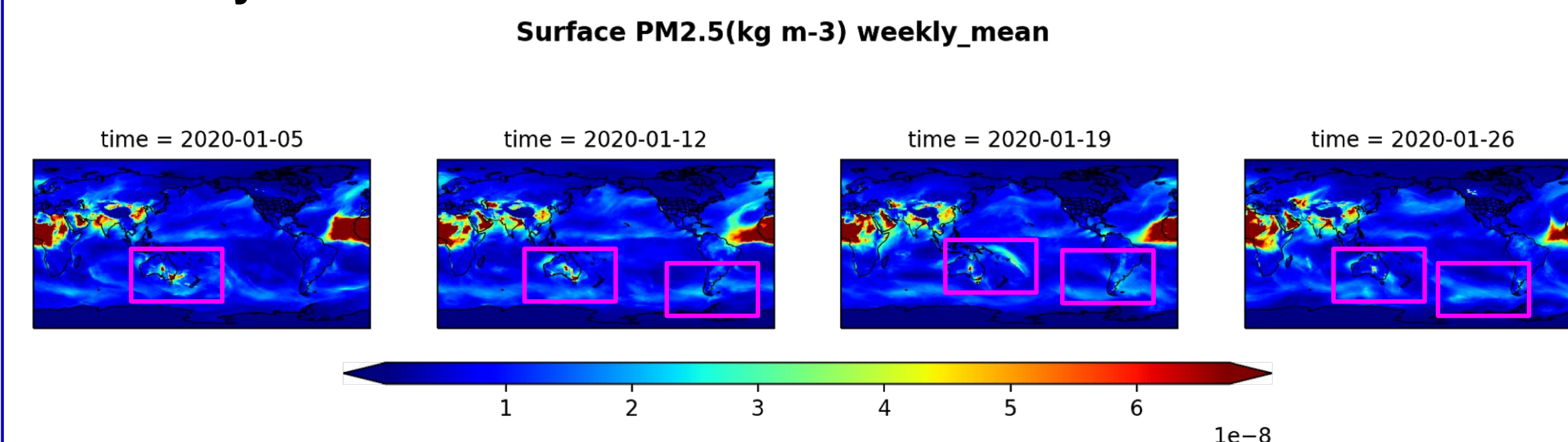
Figure 4. The evolution of weekly mean of the MERRA-2 PM 2.5 (Kg m -3 ) in Jan. 2020. Note that it is calendar week, starting from Monday to Sunday of each week. The time in the subtitle is labeled as the last day (Sunday) of that week..
