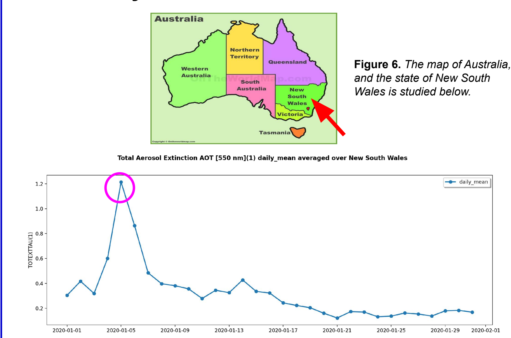
Figure 7. The evolution of daily mean of the MERRA-2 AOT over New South Wales in Australia in Jan. 2020.
