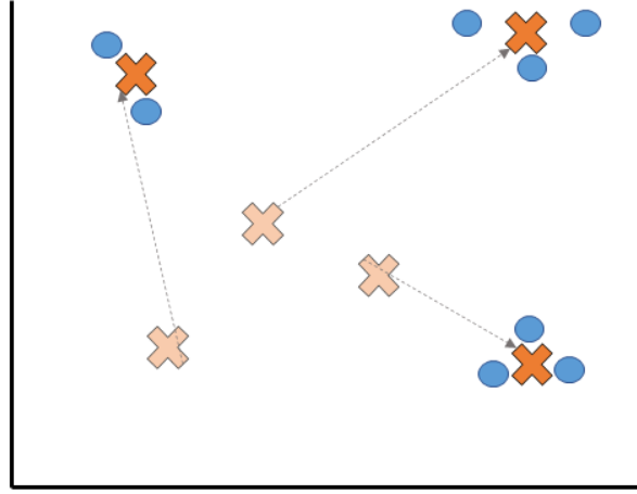
Fig. 2 Competitive Neural Network: initialized and post-training. The weight vectors w , indicated by an X , move to the location of a cluster through an iterative training process, in which a single input is inputted to the network. The weight that is closest to that location will "win," and the weight will update. After the course of successful training, weight vectors associate with clusters in the data set.
