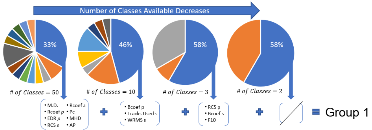
Fig. 5 Competitive Network grouping for close approach events. Strong correlations are observed with lagniappe weight initialization, such that 33% are still grouped together.
