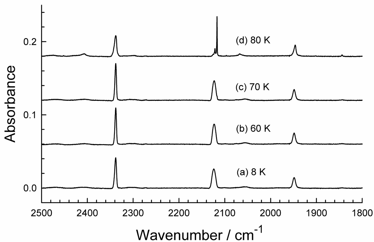
Fig. 12. Mid-IR spectra of C_3H_4 deposited at 8 K and warmed to the temperatures indicated. Spectra are offset for clarity. Spectra (a), (b), and (c) are for amorphous propyne, while (d) is for crystalline propyne. See the text for details.
