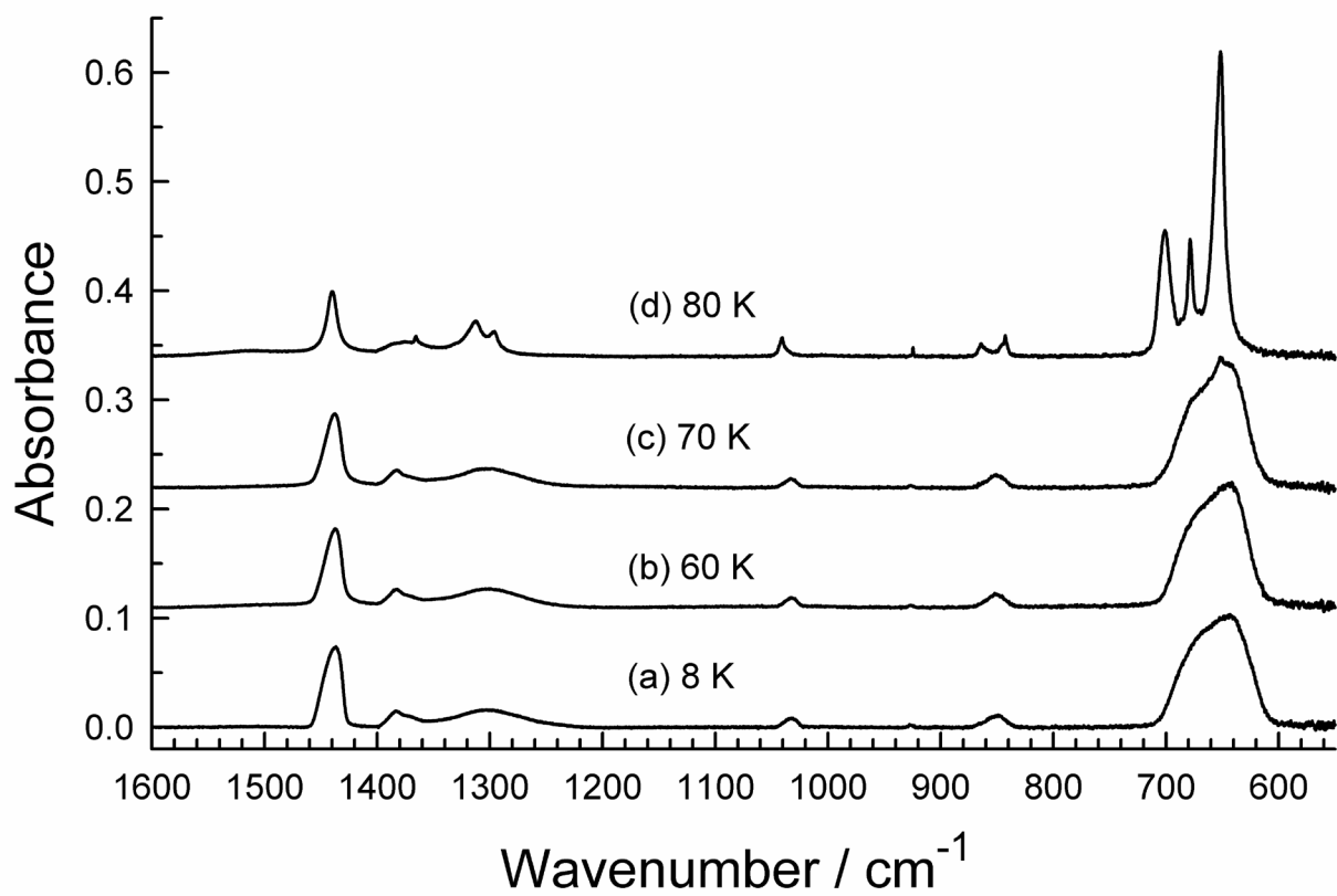
Fig. 13. Mid-IR spectra of \text{C}_3\text{H}_4 deposited at 8 K and warmed to the temperatures indicated. Spectra are offset for clarity. Spectra (a), (b), and (c) are for amorphous propyne, while (d) is for crystalline propyne. See the text for details.
