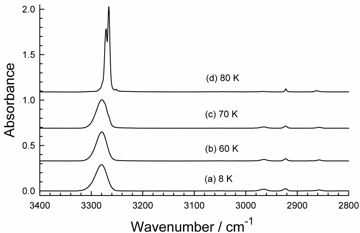
Fig. 11. Mid-IR spectra of C_3H_4 deposited at 8 K and warmed to the temperatures indicated. Spectra are offset for clarity. Spectra (a), (b), and (c) are for amorphous propyne, while (d) is for crystalline propyne. See the text for details.
