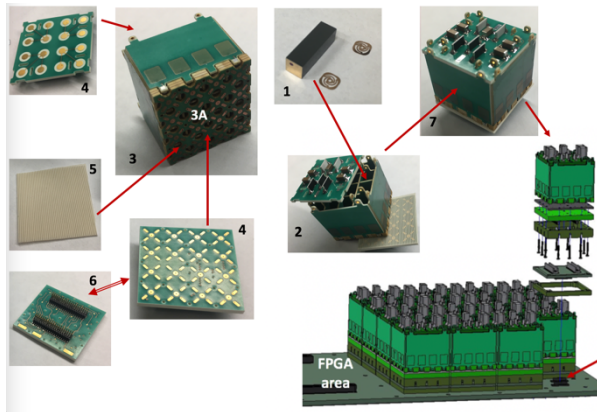
Figure 3. ImCal: single module components and 4 \times 4 module array are shown
