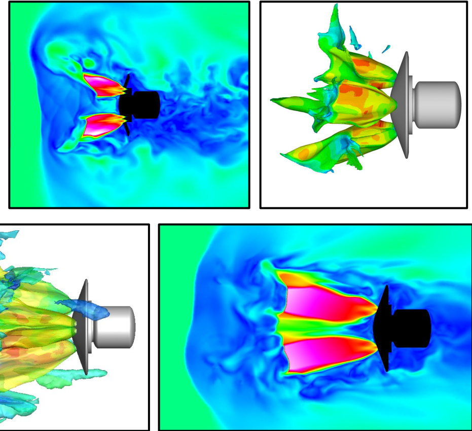
Examples of unsteady RANS solutions with insufficient spatial and temporal resolution (AIAA 2020-1510)
