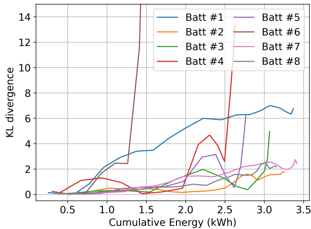
Figure 11. KL divergence cross-validation.
