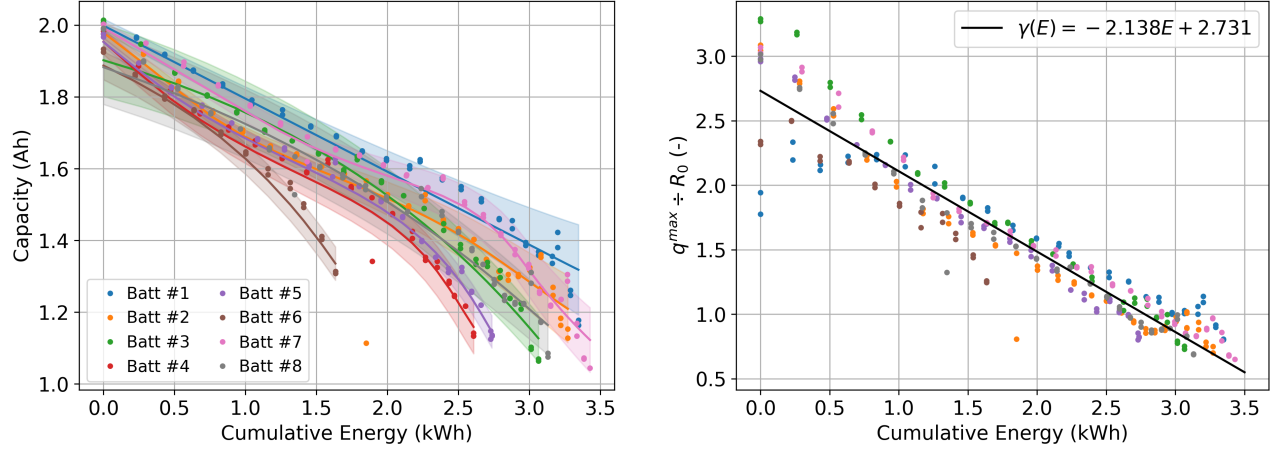
Figure 7. Variational model regressions for all 8 batteries in the data-set (left panel) and \gamma model to correlate R_0 to q^{\max} .
