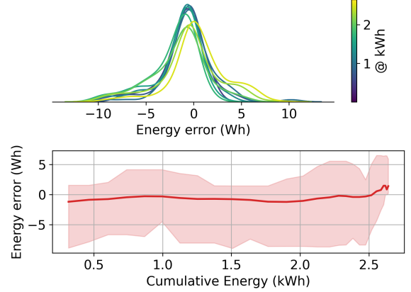
(a) Discharge cycles Energy (AUC of Power curve) error distributions (top) and evolution over Cumulative Energy (bottom).
