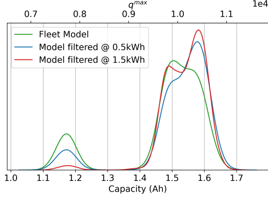
(a) Capacity and q^{max} distributions at 2.0 kWh.
