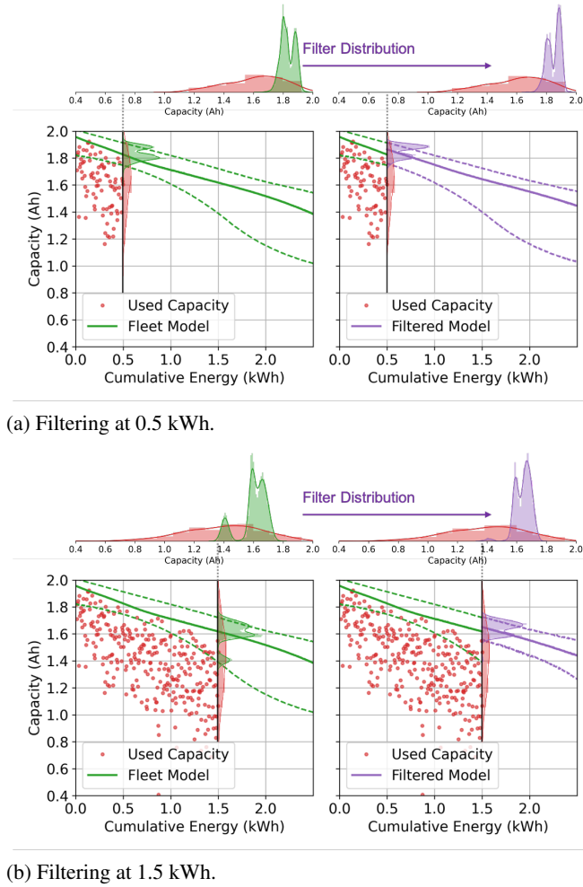
Figure 8. Filtering process using the distribution of available capacity from the fleet-wide ensemble model. The two panels refers to distributions filtered at 0.5 kWh (a) and 1.5 kWh (b).
