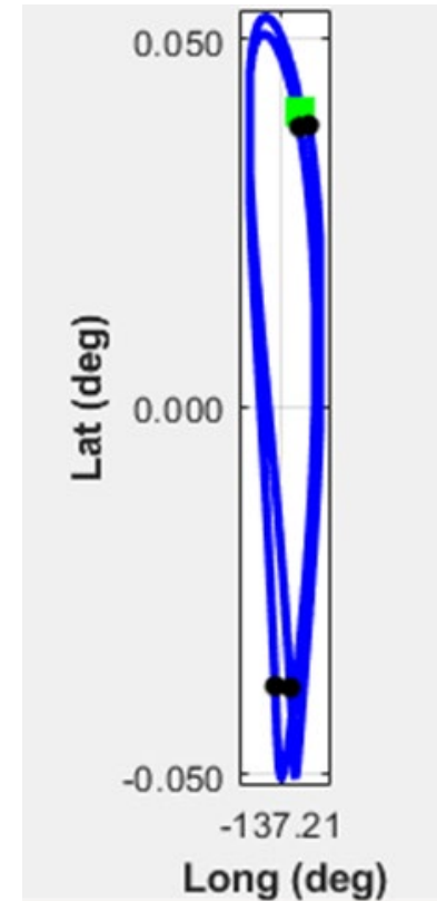
GOES-17
