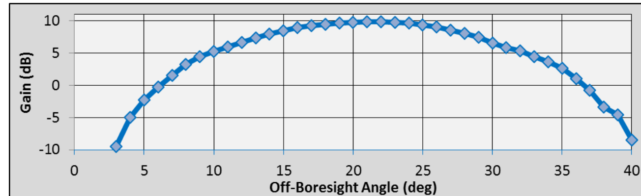
GOES-R GPS Rx Antenna Average Pattern
