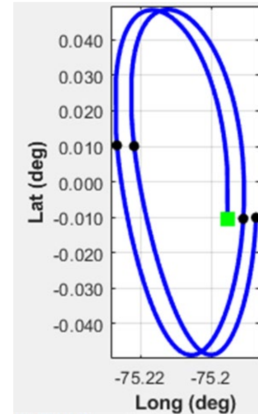
GOES-16
