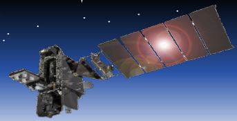
GOES-17
