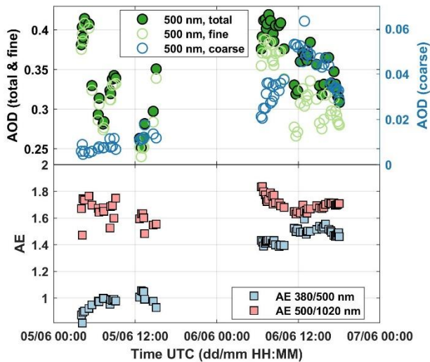
890 Figure 3. AERONET sun-photometer observations (in Kuopio station, on 5 and 6 June 2019, http://aeronet.gsfc.nasa.gov , last access: 3 May 2021) of (top) 500 nm aerosol optical depth (level 2.0 data) and (bottom) Ångström exponents (AE) computed from the optical depths measured at 380, 500, and 1020 nm. The fine-mode-related (for particle with diameters < 1µm) and coarse-mode-related aerosol optical depth (diameters > 1µm) are shown in addition (top, level 2.0 aerosol spectral deconvolution algorithm (SDA) products).
