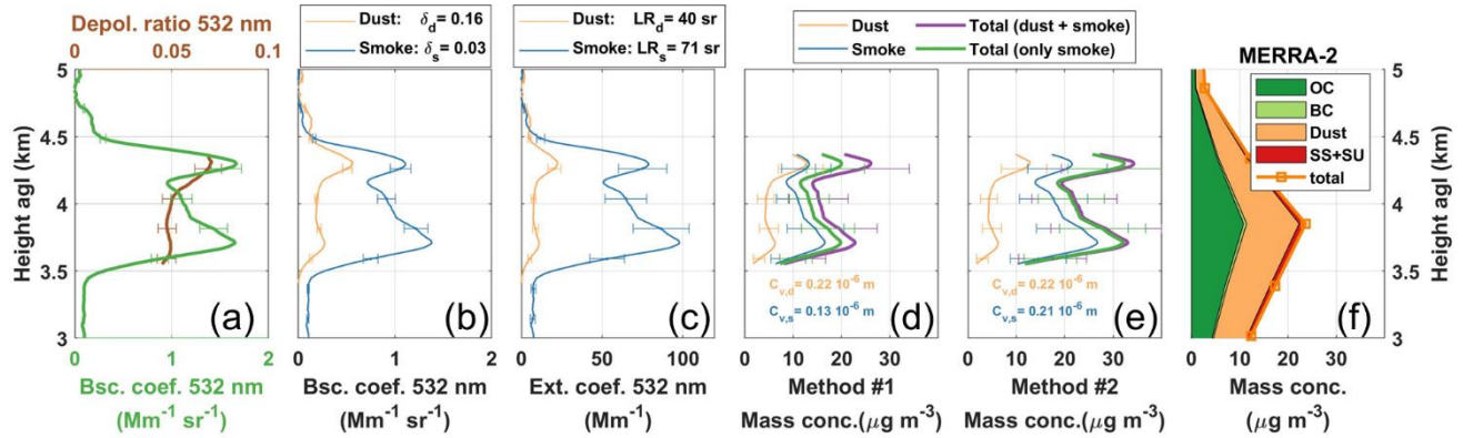
Figure 8. Lidar products obtained from PollyXT measurements on 5 June 2019, 8–10h UTC (2h signal average). (a) Measured 532 nm total particle backscatter coefficient (green) and particle linear depolarization ratio (brown). (b) Particle backscatter coefficients (BSCs) for fine dust (orange) and smoke (blue) particles, obtained with the POLIPHON method. (c) Respective fine dust and smoke extinction coefficients (EXTs) obtained by multiplying the BSCs (in b) with the lidar ratios. (d,e) The fine dust (orange), smoke (blue) particle mass concentrations derived from the EXT profiles (in c), by using parameters in Table 4 for method #1 (d) and #2 (e). The total mass concentrations of fine dust and smoke mixture (purple), or of only smoke particles (green) are shown. (f) Mass concentrations of organic carbon (OC, dark green), black carbon (BC, light green), dust (orange), sea salt and sulphate (SS+SU, red) from MERRA-2 model, at 9h UTC on 5 June. The total mass concentration profile is also given by orange squares. The horizontal lines illustrate the uncertainties range.
