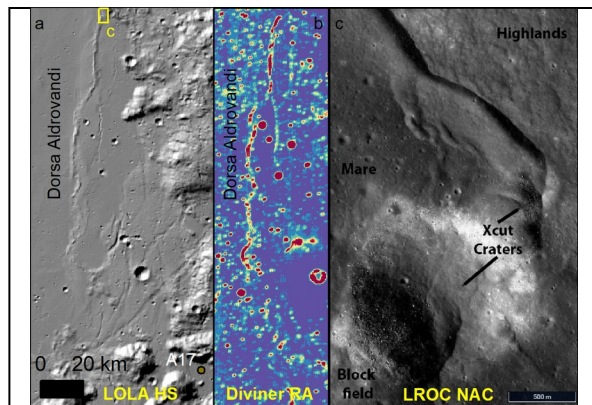
Figure 1. (a) The young, rocky wrinkle-ridge Dorsa Aldrovandi extends at its north from the mare-flood Le Monnier crater on the eastern rim of Serenitatis southward across several mare units. The Apollo 17 site in Taurus-Littrow is at the bottom right of (a). (b) The Diviner rock abundance [4] of the wrinkle-ridge is elevated over its entire length, which suggests recent activity. (c) Craters are cross-cut by the wrinkle-ridge (another argument for the ridge's youth). Blocks are exposed that could be examined with geology or geochemistry instruments during a long traverse. Detail here is centered at 29.1E, 25.7N.
