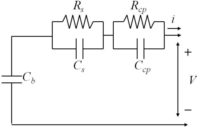
Fig. 5. Equivalent Circuit Based Model [13]
