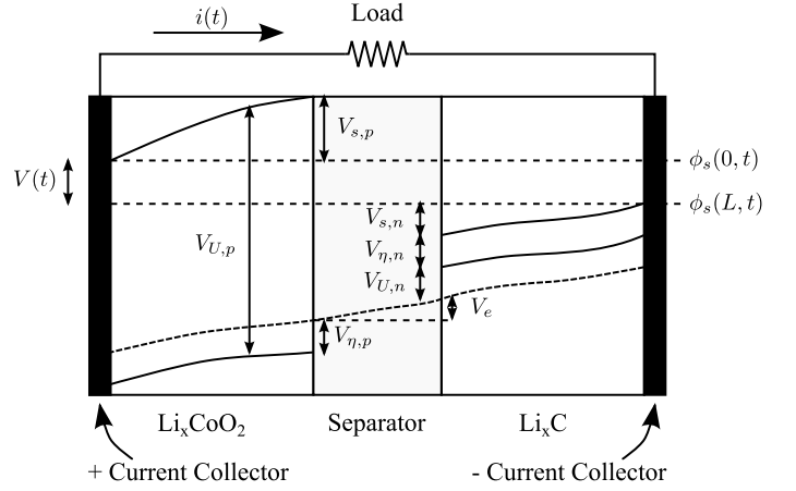
Fig. 3. Battery voltages [10]
