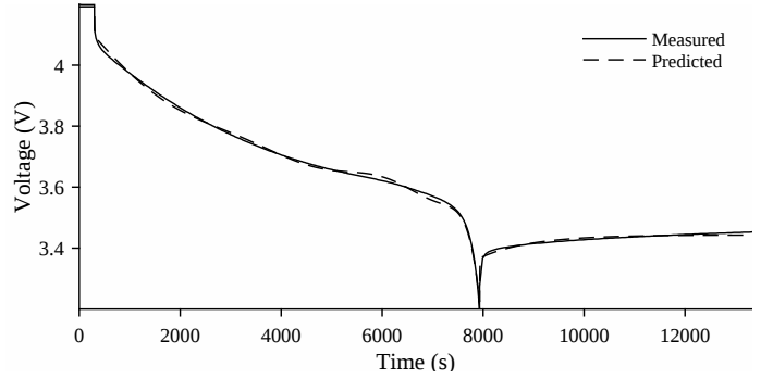
Fig. 4. Battery voltage during 1 A discharge cycle [10].
