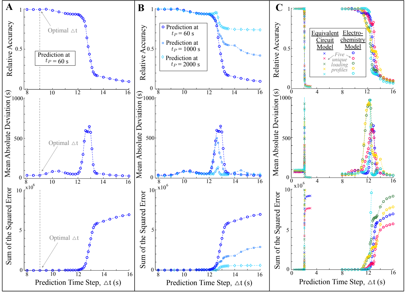
Fig. 7. Effect of time step on prediction results. A) RA, MAD, and Error as a function of \Delta t for battery data predicted from t_P = 60 sec (data comparable to that used in Fig. 6 and Fig. 8). B) Same as panel A , with addition of predictions made closer to EOL, starting at t_P = 1000 sec and t_P = 2000 sec. C) Same as in panel A , but including results from 5 other data sets with unique loading profiles (distinguished by color), and using both the electrochemistry battery model and the equivalent circuit battery model (distinguished by symbol). All panels reflect an average of 100 simulations.
